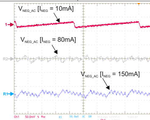
Figure 87. V NEG Output Voltage Ripple — SYNC = HIGH — L = 2.2 \mu H — C OUT = 2 × 10 \mu F
