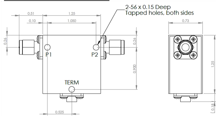
D3I2327S-3 Dimensions
