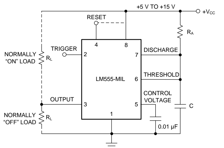
Figure 11. Monostable
