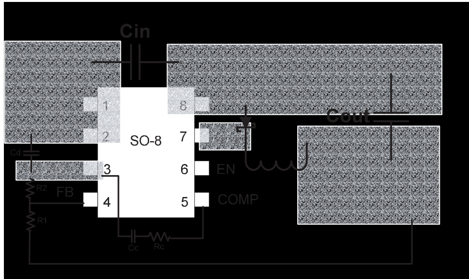
Figure 3. AOZ1019 PCB Layout
