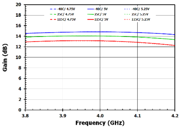
Figure 18. Gain
