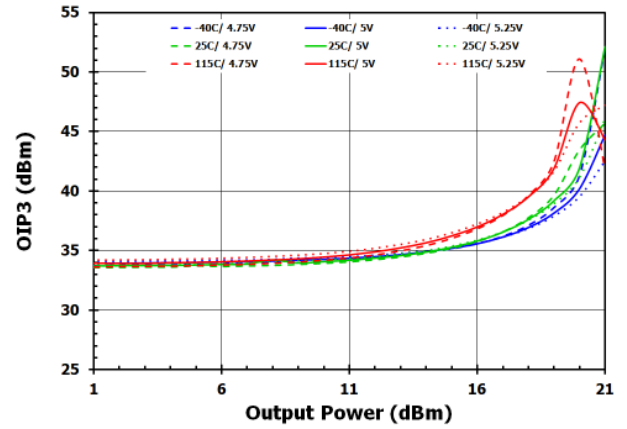
Figure 23. OIP3 vs Tone Power (4GHz)
