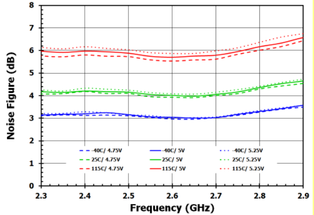
Figure 9. Noise Figure
