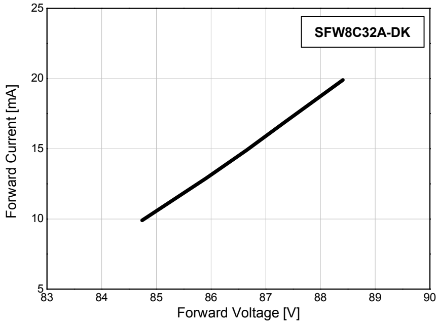
Fig 2. Forward Voltage vs. Forward Current, T_j=25^\circ\text{C}
