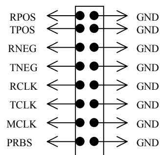
Figure 4. SYSTEM CONNECTOR
