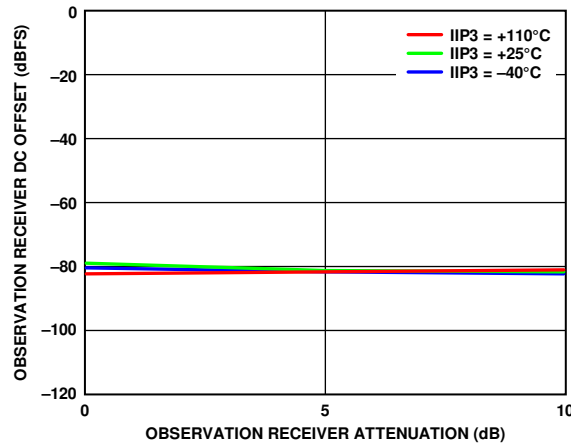
Figure 198. Observation Receiver DC Offset vs. Observation Receiver Attenuation, LO = 4600 MHz
