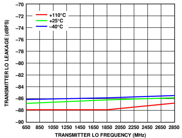
Figure 84. Transmitter LO Leakage vs. Transmitter LO Frequency, Transmitter Attenuation = 0 dB
