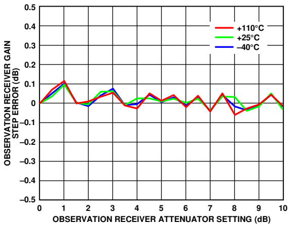
Figure 194. Observation Receiver Gain Step Error vs. Observation Receiver Attenuator Setting, LO = 4600 MHz
