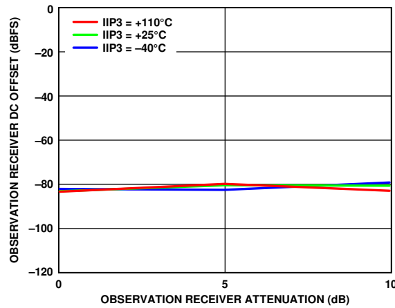
Figure 197. Observation Receiver DC Offset vs. Observation Receiver Attenuation, LO = 3600 MHz
