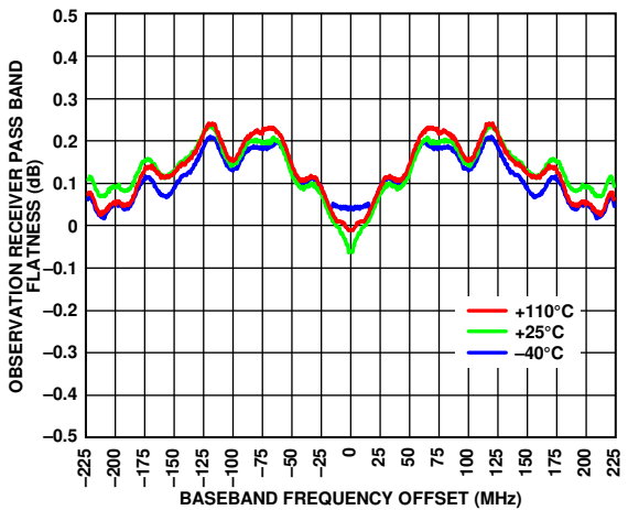
Figure 195. Observation Receiver Pass Band Flatness vs. Baseband Frequency Offset, LO = 3600 MHz
