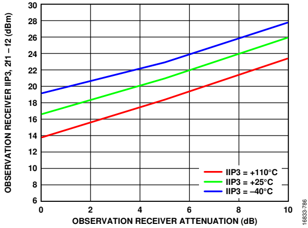
Figure 187. Observation Receiver IIP3, 2f1 - f2 vs. Observation Receiver Attenuation, LO = 3600 MHz, Tone 1 = 3602 MHz, Tone 2 = 3722 MHz, -22 dBm Plus Attenuation Each
