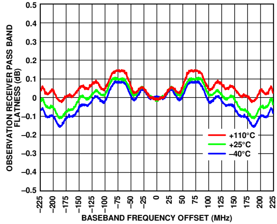
Figure 196. Observation Receiver Pass Band Flatness vs. Baseband Frequency Offset, LO = 4600 MHz
