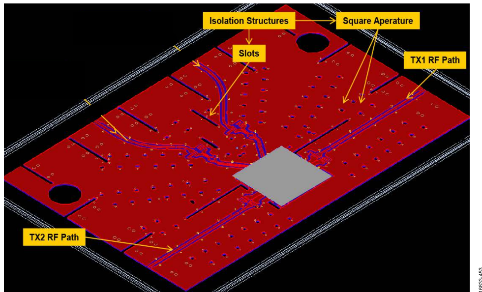
Figure 282. Isolation Structures on the ADRV9008-2W/PCBZ
