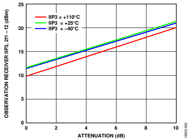
Figure 58. Observation Receiver IIP3, 2f_1 - f_2 vs. Attenuation, LO = 300 MHz, Tone 1 = 345 MHz, Tone 2 = 346 MHz at -24 dBm Plus Attenuation
