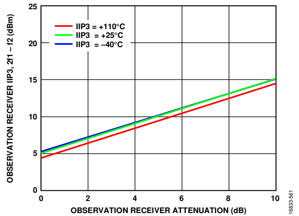
Figure 57. Observation Receiver IIP3, 2f_1 - f_2 vs. Observation Receiver Attenuation, LO = 75 MHz, Tone 1 = 100 MHz, Tone 2 = 101 MHz at -24 dBm Plus Attenuation
