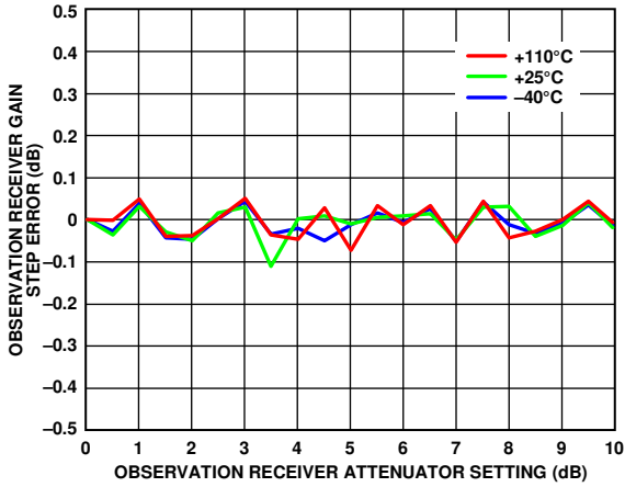
Figure 193. Observation Receiver Gain Step Error vs. Observation Receiver Attenuator Setting, LO = 3600 MHz
