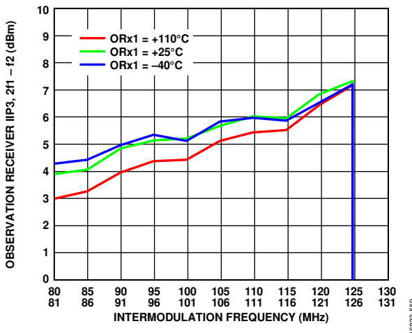
Figure 55. Observation Receiver IIP3, 2f_1 - f_2 vs. Intermodulation Frequency, LO = 75 MHz, Attenuation = 0 dB, Tones Separated by 1 MHz Swept Across Pass Band at -25 dBm Each
