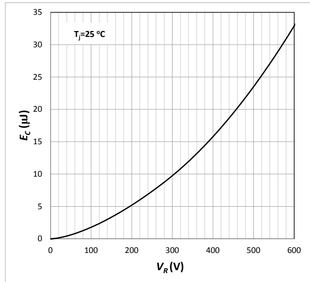
Fig. 8 Typical Capacitance Stored Energy
