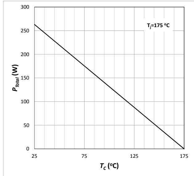
Fig. 4 Power Derating
