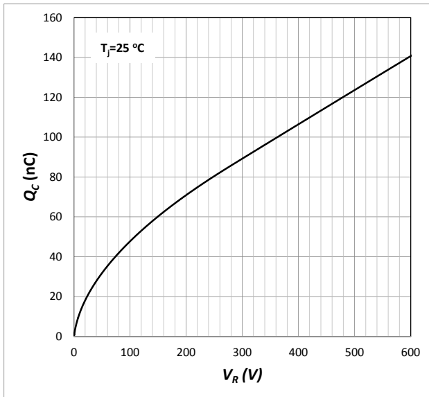
Fig. 7 Capacitive Charge
