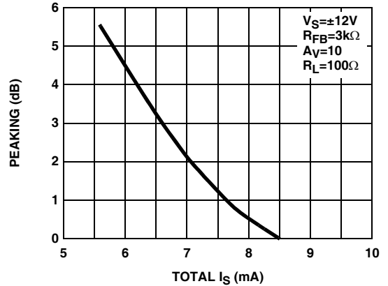
FIGURE 10. PEAKING vs I_{S+}
