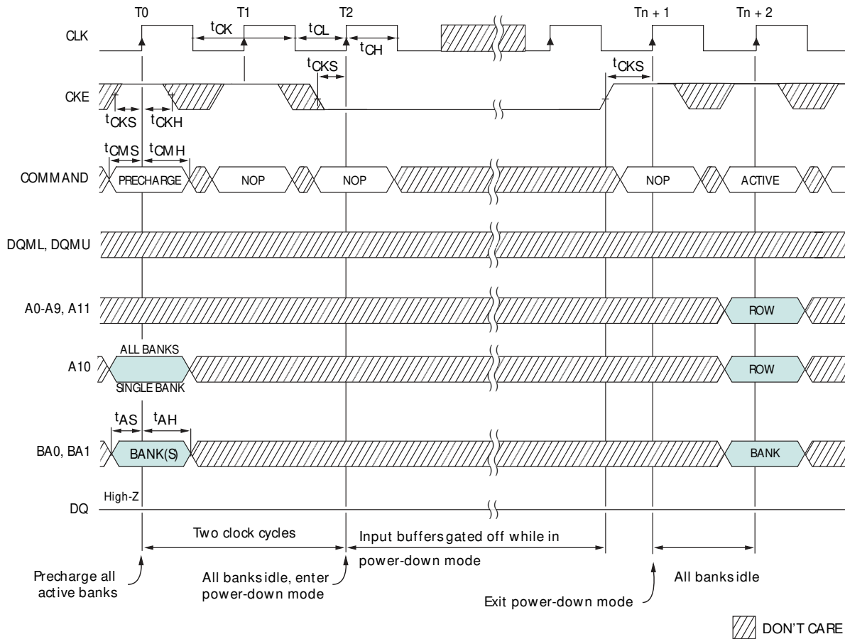
Figure 32: Power-Down Mode 1
