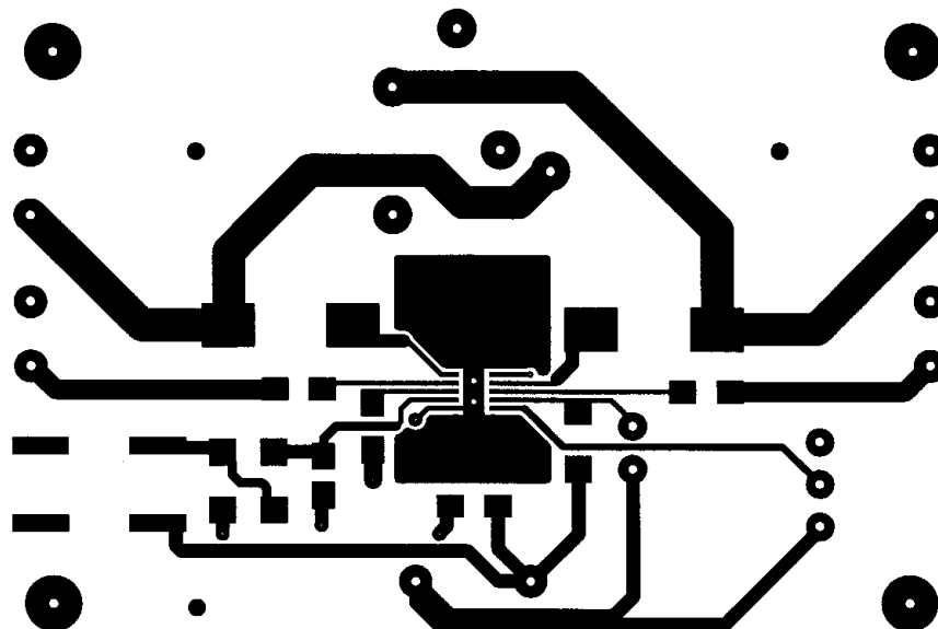
Figure 47. Recommended WSON/SOP PC Board Layout: TOP Top Layer
