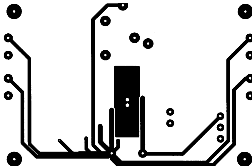
Figure 48. Recommended WSON/SOP PC Board Layout: Bottom Layer
