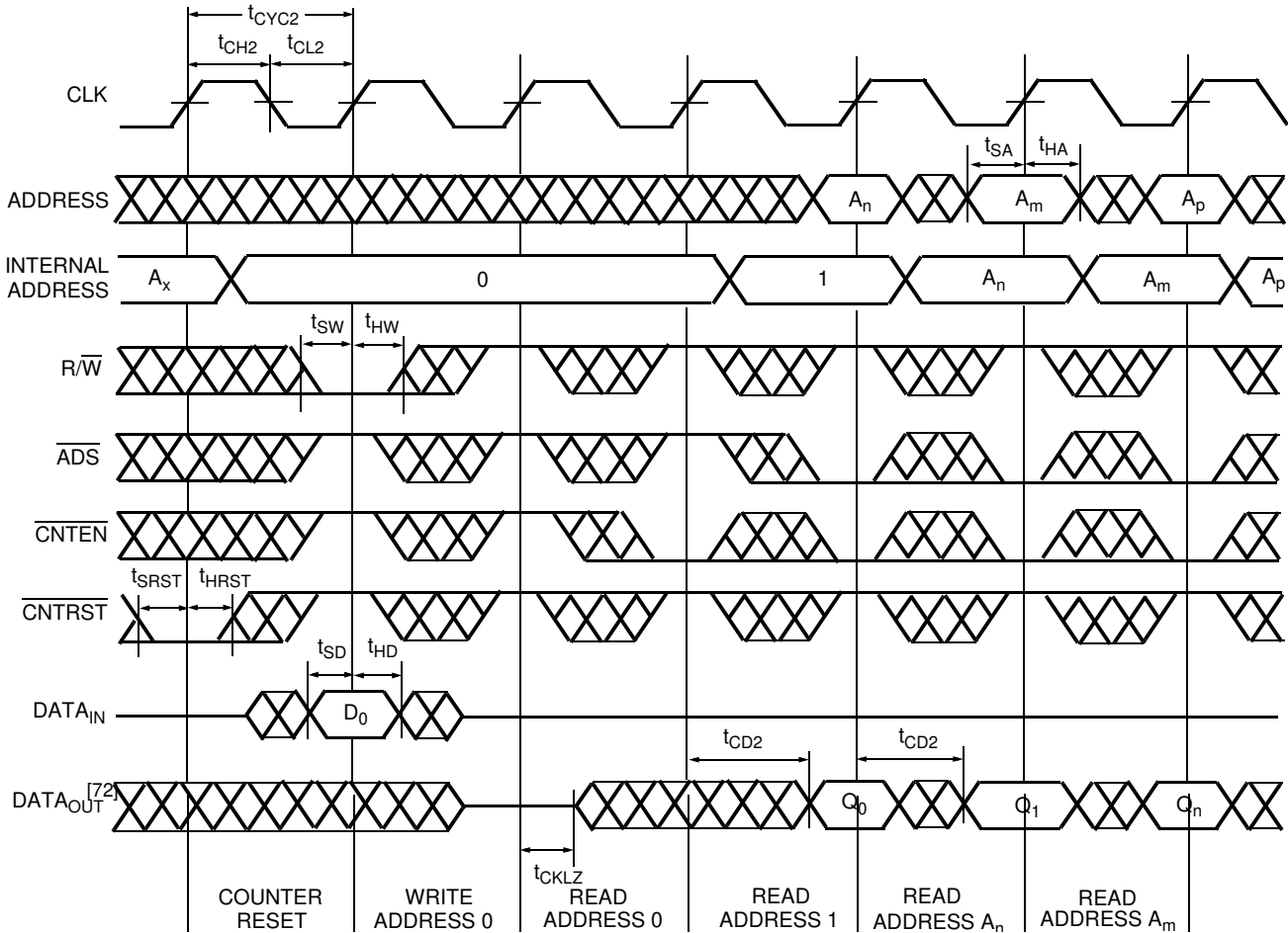
Figure 11. Counter Reset [59, 60]
