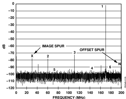
Figure 20. AD12401 with AFB Digital Postprocessing
