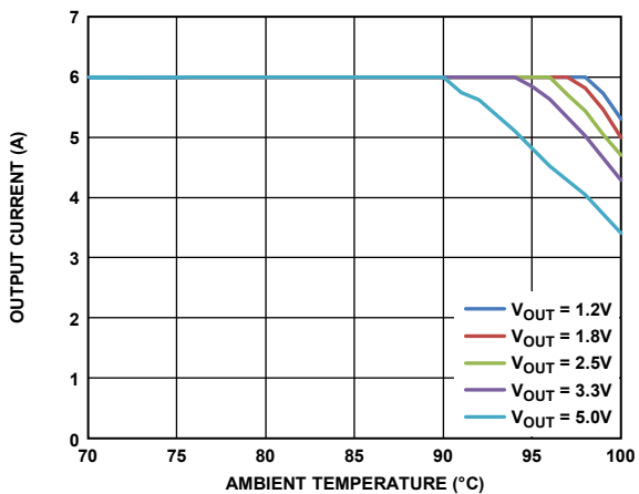
Figure 25. Output Current vs. Ambient Temperature at V_{IN} = 12 V , f_{SW} = 600 \text{ kHz} , Measured on the ADP2387 Evaluation Board
