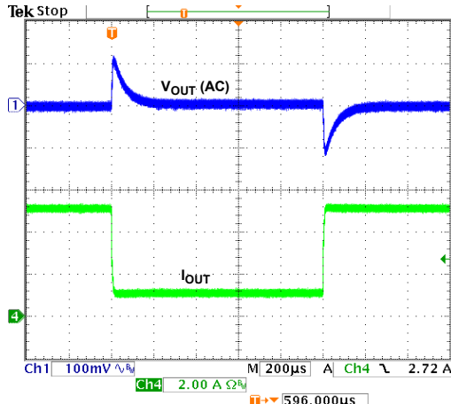
Figure 23. Load Transient Response, 1 A to 5 A
