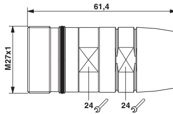
Dimensioned drawing
