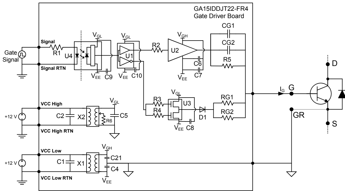
Figure 25: Topology of the GA15IDDJT2-FR4 Two Voltage Source gate driver.
