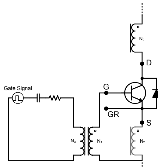
Figure 30: Simplified Current Controlled Proportional Driver
