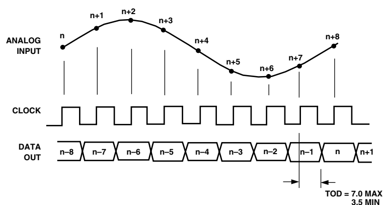
Figure 1. Timing Diagram
