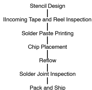
FIGURE 5. SMT Assembly Process Flow
