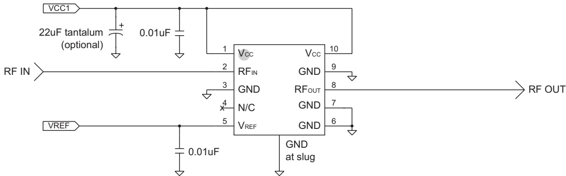
Figure 11: Application Circuit
