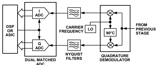
Figure 30. Typical Analog QAM Demodulator
