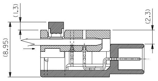
SECT B-B
