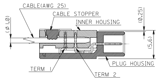
SECT C-C
