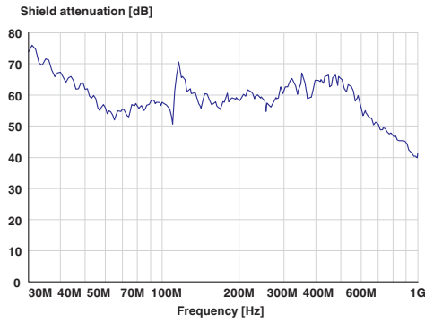
Shield attenuation
