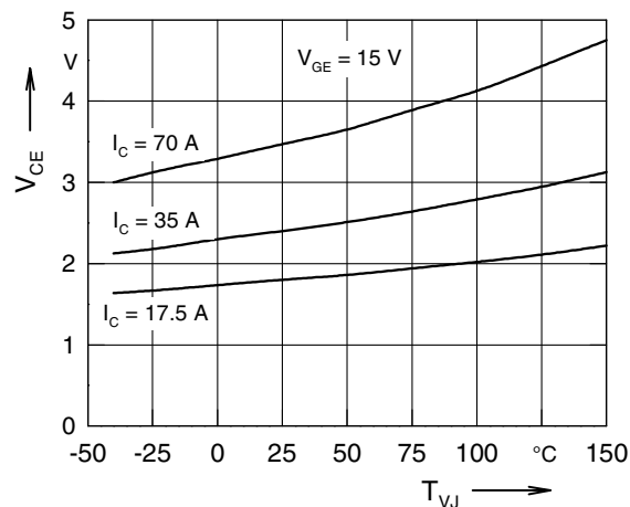
Fig. 4 Typ. collector emitter saturation as a function of case temperature
