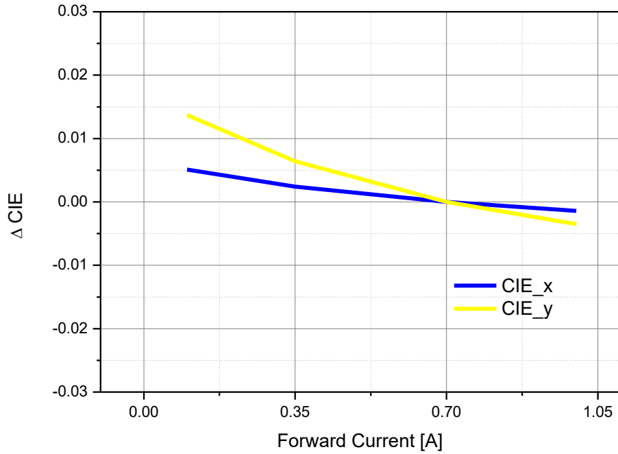
Forward Current vs \Delta CIE , T_j=25^\circ C (White)
