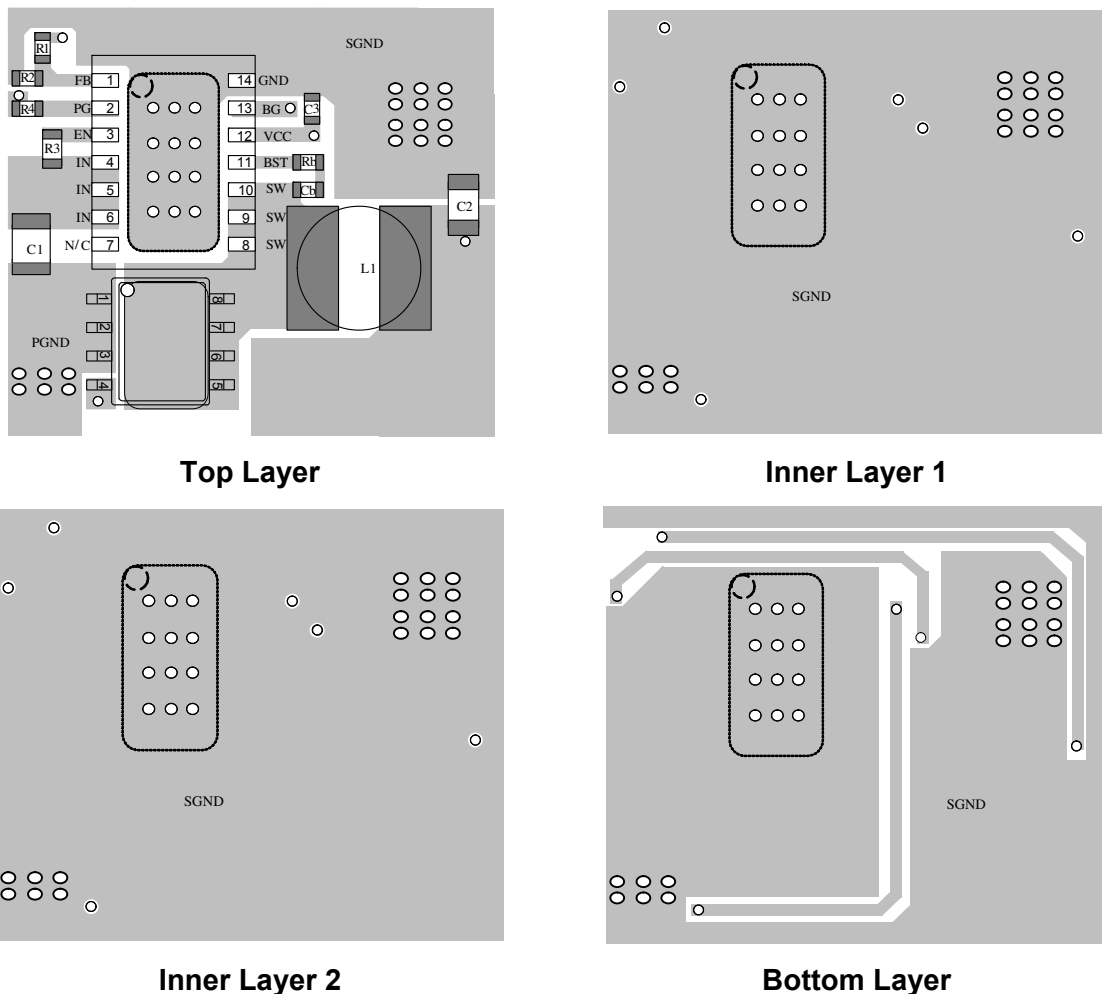
Figure 4—PCB Layout
