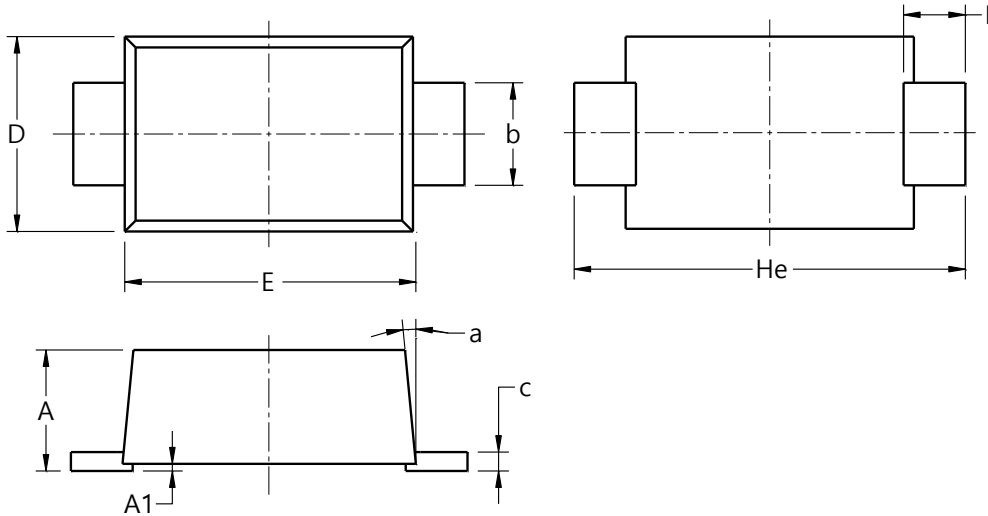
DO-219AA
