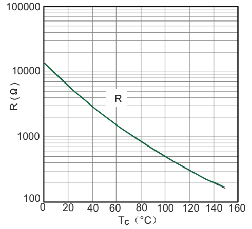
Figure 14: NTC Characteristics
