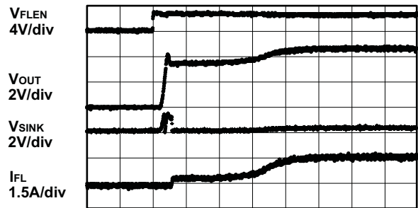
Time (40 \mu\text{s/div} )
