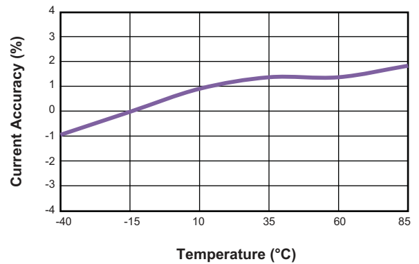
Movie Mode Accuracy vs. Temperature (I FL = 216mA, V IN = 3.6V, L = 1μH)
