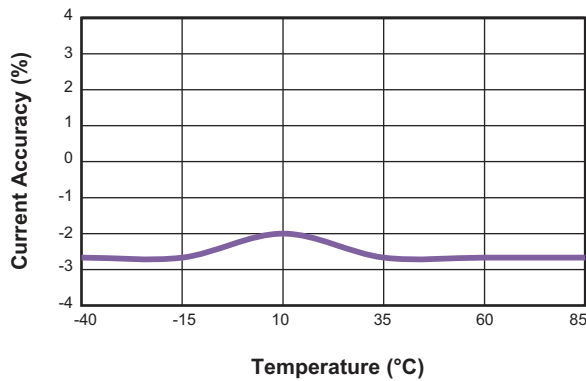
Flash Mode Accuracy vs. Temperature (I FL = 1.5A, V IN = 3.6V, L = 1μH)
