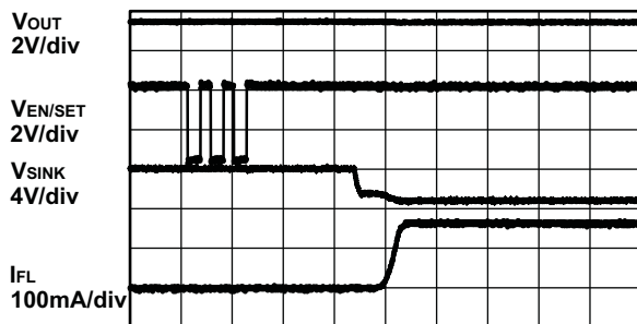
Time (20 \mu\text{s/div} )
