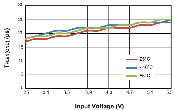
Flash On-Time Delay vs. Input Voltage (I FL = 1.5A, C OUT = 2.2μH, L = 1μH)
