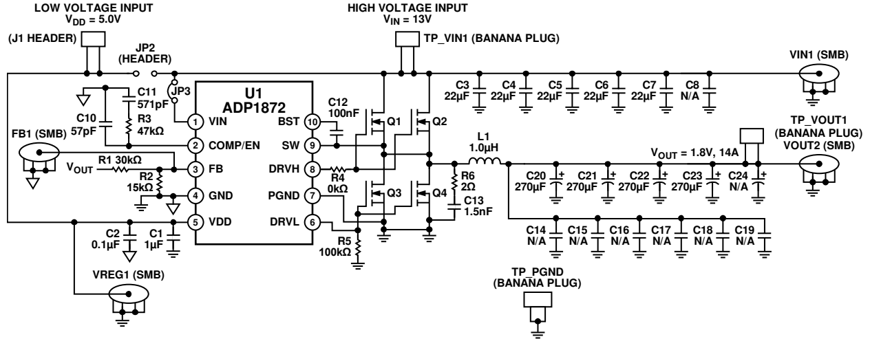
Figure 29. 1.8 V Output, 300 kHz, 14 A Application Circuit
