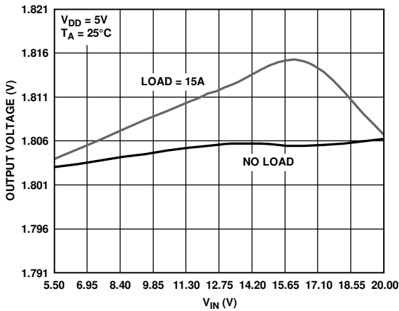
Figure 5. Line Regulation Plot for f_{SW} = 300\text{ kHz} , V_{OUT} = 1.8\text{ V}
