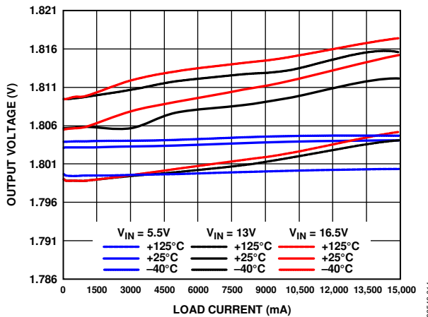
Figure 7. Output Voltage Accuracy—300 kHz, V_{OUT} = 1.8\text{ V}
