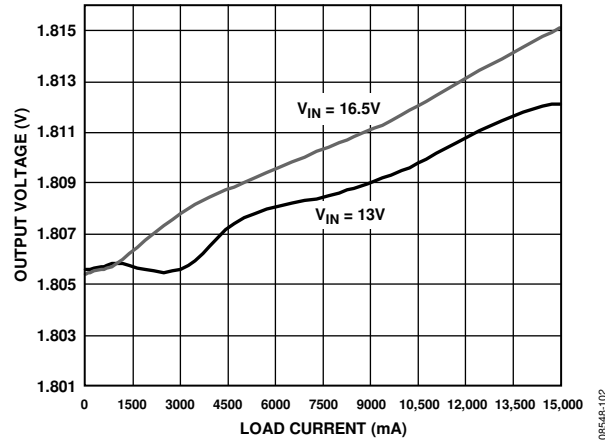
Figure 6. Load Regulation Plot for f_{SW} = 300\text{ kHz} , V_{OUT} = 1.8\text{ V}
