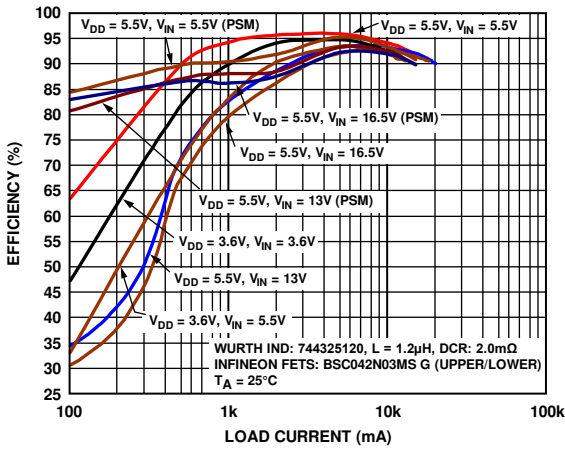
Figure 3. Efficiency—300 kHz, V_{OUT} = 1.8\text{ V}
