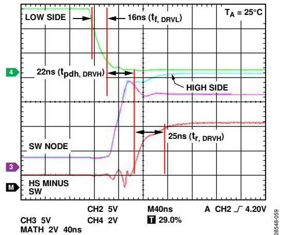
Figure 25. Upper-Side Driver Rising and Lower-Side Falling Edge Waveforms, C_{IN} = 4.3 \text{ nF} (Upper-/Lower-Side MOSFET), Q_{TOTAL} = 27 \text{ nC} ( V_{GS} = 4.4 \text{ V} (Q1), V_{GS} = 5 \text{ V} (Q3))
