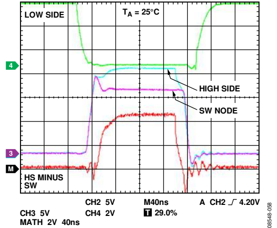
Figure 24. Output Drivers and SW Node Waveforms
