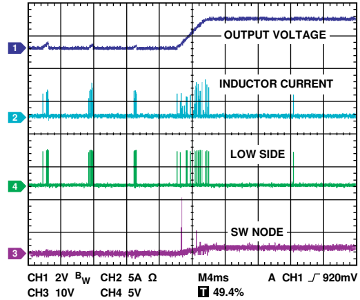
Figure 18. Output Short-Circuit Behavior Leading to Hiccup Mode
