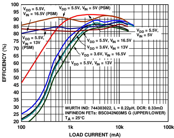
Figure 4. Efficiency—1 MHz, V_{OUT} = 1.8\text{ V}
