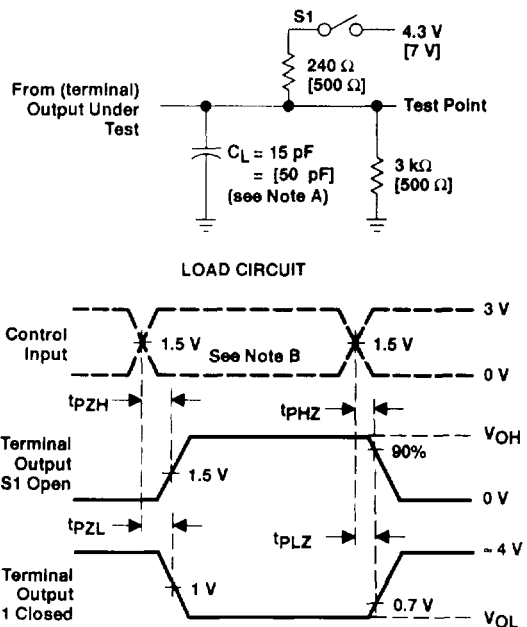
Figure 4. Terminal Load Circuit and Voltage Waveforms
