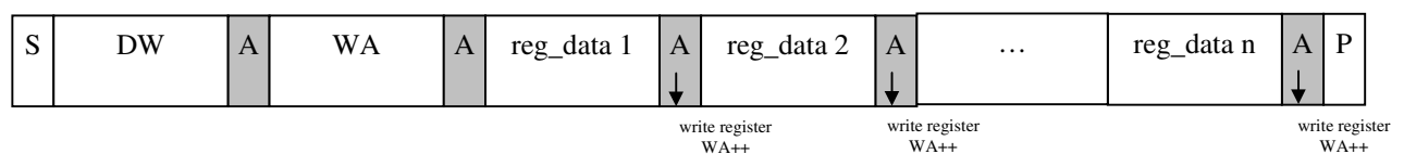
Figure 25 – I 2 C Page-Write:
