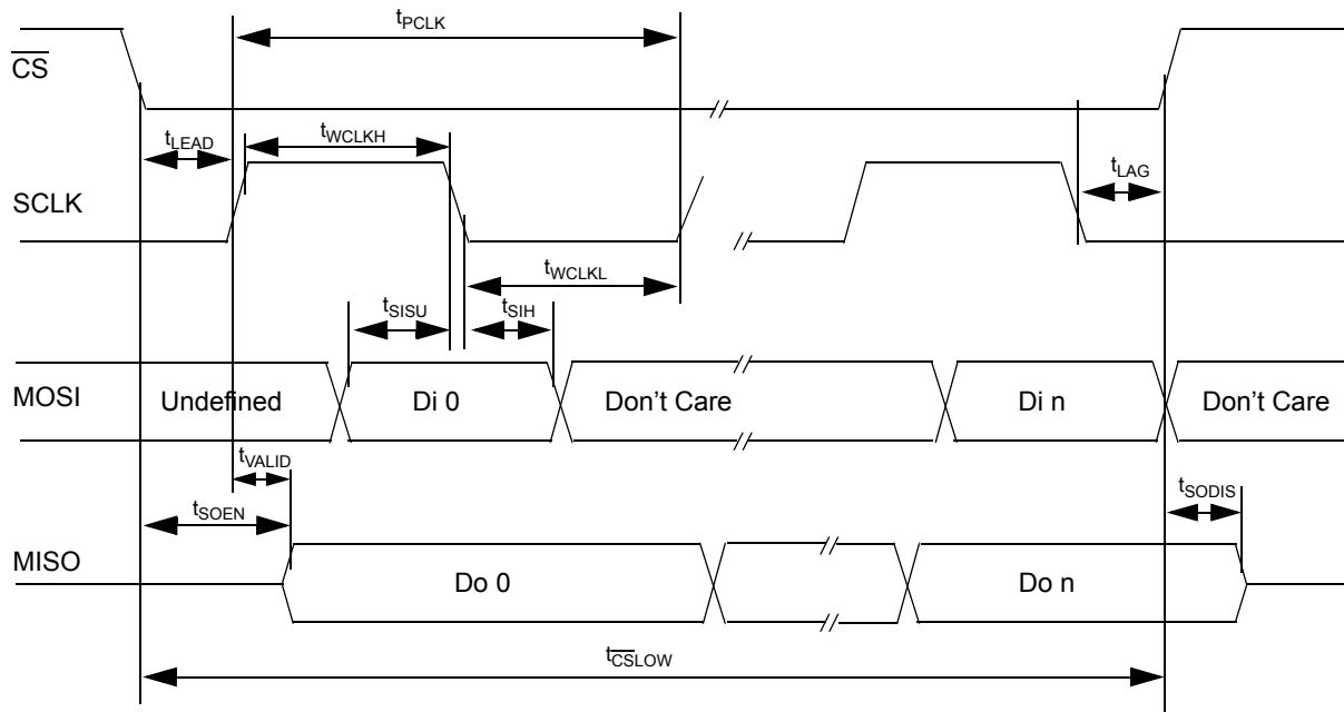
Figure 14. SPI Timing
