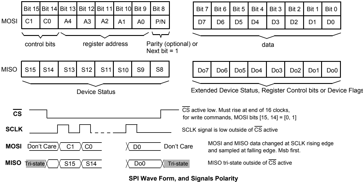
Figure 41. SPI Overview
