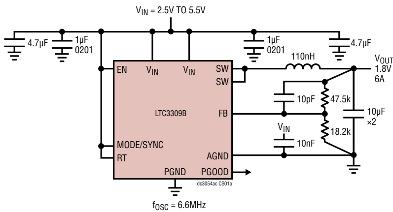
High Efficiency, 6.6MHz, 1.8V 6A Step-Down Converter
