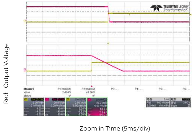
Figure 18. PG# alarmed 10ms prior to V_o < 40V , V_{IN} = 230V_{AC} , Output at Full load
