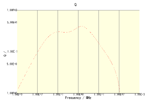
CLF7045T-1R5N-CA
