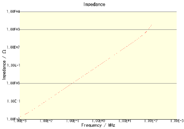
CLF7045T-1R5N-CA
