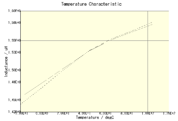
CLF7045T-1R5N-CA(DC = 0A)
