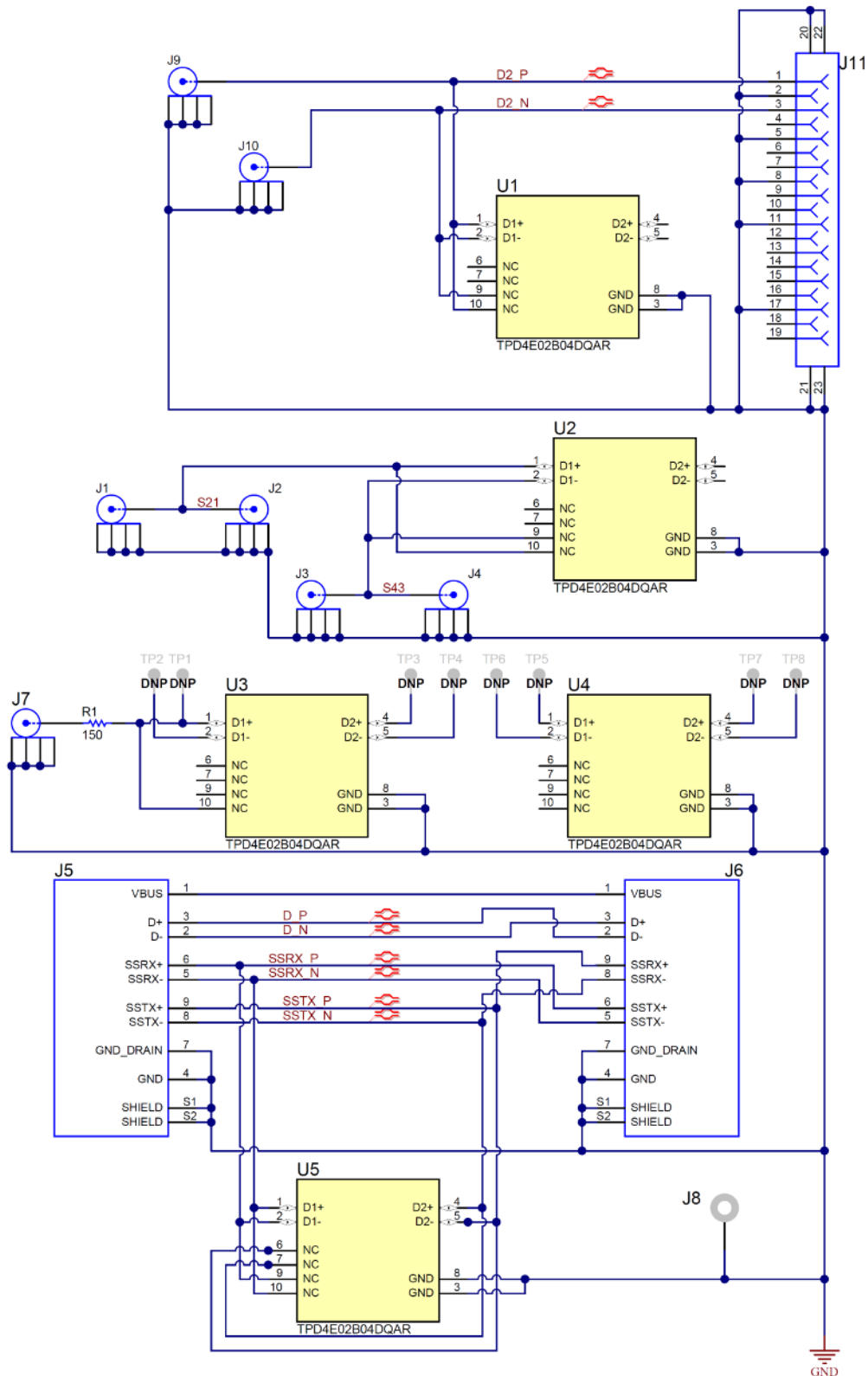
Figure 4. TPD4E02B04EVM Schematic
