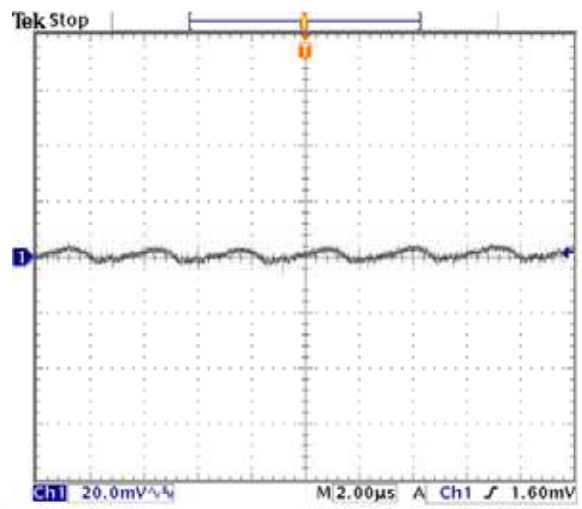
Fig-2.0V-5: Output voltage ripple (20mV/div.) for V_{out}=2.0V at full rated load current into a resistive load with external capacitance 47\mu F \times 2 ceramic + 1\mu F ceramic at V_{in}=12.0V . Time scale: 2μs/div
