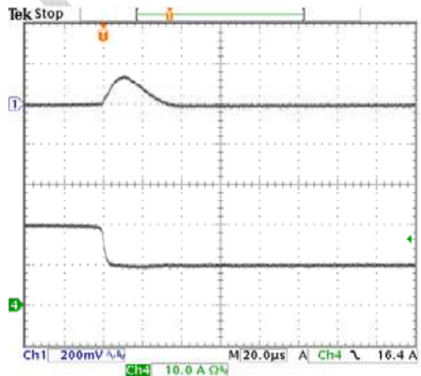
Fig-1.0V-7: Output voltage response for V_{out}=1.0V to positive load current step-change from 20A to 10A with slew rate of -5A/\mu s at V_{in}=12.0V . C_o=47\mu F \times 2 ceramic. Top trace: output voltage (200mV/div.) Bottom trace: load current (10A/div.) Time scale: 20µs/div.
