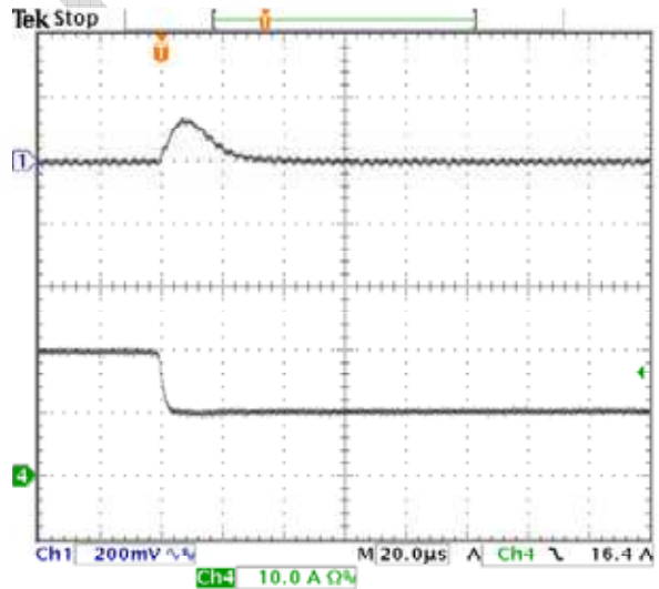
Fig-3.3V-7: Output voltage response for V_{out}=3.3V to positive load current step-change from 20A to 10A with slew rate of -5A/\mu s at V_{in}=12.0V . C_o=47\mu F \times 2 ceramic. Top trace: output voltage (200mV/div.) Bottom trace: load current (10A/div.) Time scale: 20μs/div.
