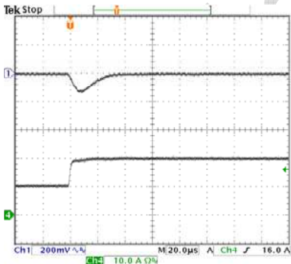
Fig-2.0V-6: Output voltage response for V_{out}=2.0V to positive load current step-change from 10A to 20A with slew rate of 5A/\mu s at V_{in}=12.0V . C_o=47\mu F \times 2 ceramic. Top trace: output voltage (200mV/div.) Bottom trace: load current (10A/div.) Time scale: 20μs/div.
