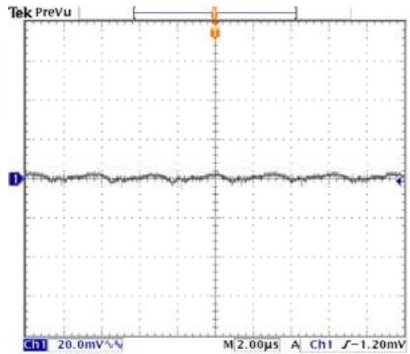
Fig-1.5V-5: Output voltage ripple (20mV/div.) for V_{out}=1.5V at full rated load current into a resistive load with external capacitance 47\mu F \times 2 ceramic + 1\mu F ceramic at V_{in}=12.0V . Time scale: 2μs/div
