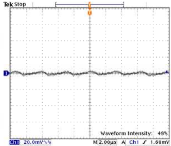
Fig-1.8V-5: Output voltage ripple (20mV/div.) for V_{out}=1.8V at full rated load current into a resistive load with external capacitance 47\mu F \times 2 ceramic + 1\mu F ceramic at V_{in}=12.0V . Time scale: 2µs/div
