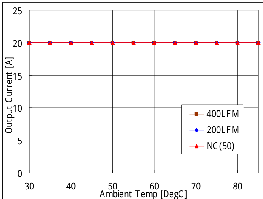
Fig-2.0V-1: Available load current vs. ambient temperature and airflow rates for V_{out}=2.0V with V_{in}=12.0V . Maximum component temperature \leq 120^{\circ}C
