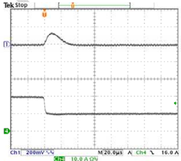
Fig-2.0V-7: Output voltage response for V_{out}=2.0V to positive load current step-change from 20A to 10A with slew rate of -5A/\mu s at V_{in}=12.0V . C_o=47\mu F \times 2 ceramic. Top trace: output voltage (200mV/div.) Bottom trace: load current (10A/div.) Time scale: 20μs/div.
