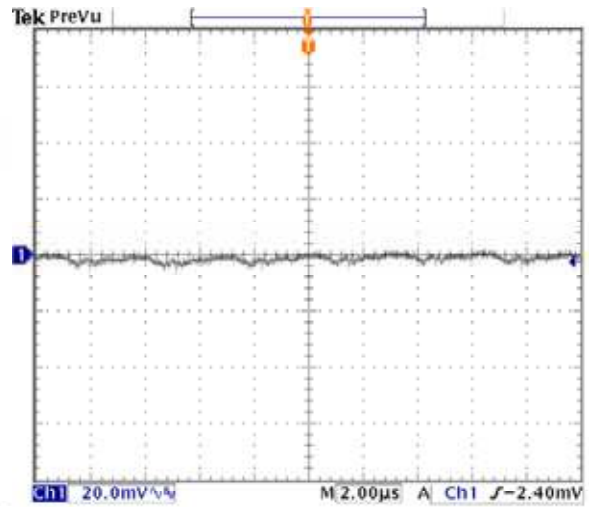
Fig-1.2V-5: Output voltage ripple (20mV/div.) for V_{out}=1.2V at full rated load current into a resistive load with external capacitance 47\mu F \times 2 ceramic + 1\mu F ceramic at V_{in}=12.0V . Time scale: 2μs/div
