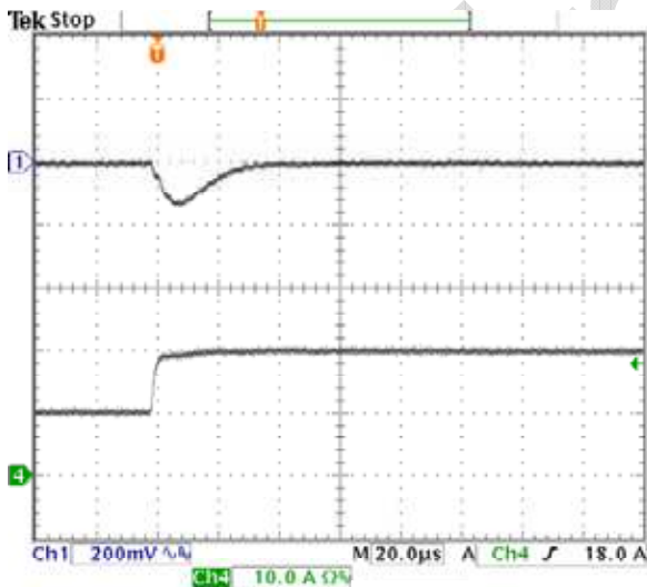
Fig-1.8V-6: Output voltage response for V_{out}=1.8V to positive load current step-change from 10A to 20A with slew rate of 5A/\mu s at V_{in}=12.0V . C_o=47\mu F \times 2 ceramic. Top trace: output voltage (200mV/div.) Bottom trace: load current (10A/div.) Time scale: 20µs/div.
