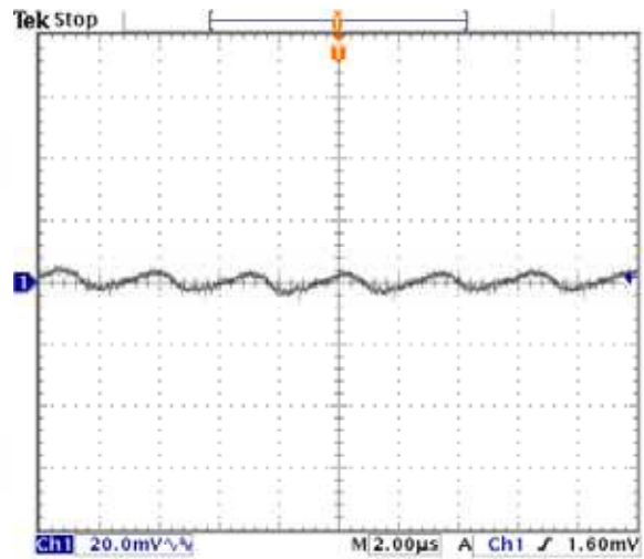
Fig-2.5V-5: Output voltage ripple (20mV/div.) for V_{out}=2.5V at full rated load current into a resistive load with external capacitance 47\mu F \times 2 ceramic + 1\mu F ceramic at V_{in}=12.0V . Time scale: 2μs/div
