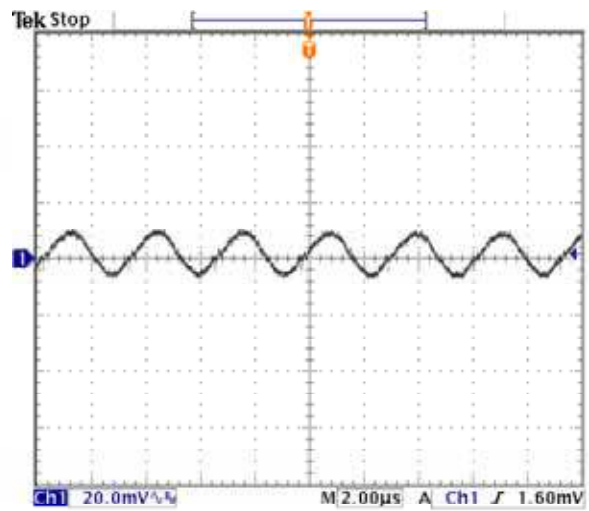
Fig-5.0V-5: Output voltage ripple (20mV/div.) for V_{out}=5.0V at full rated load current into a resistive load with external capacitance 47\mu F \times 2 ceramic + 1\mu F ceramic at V_{in}=12.0V . Time scale: 2 µs/div
