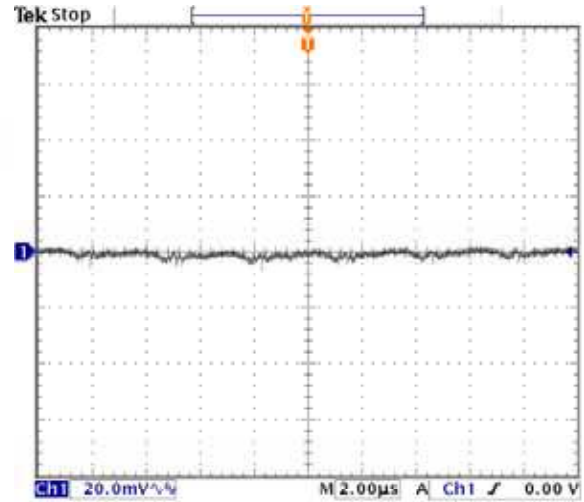
Fig-1.0V-5: Output voltage ripple (20mV/div.) for V_{out}=1.0V at full rated load current into a resistive load with external capacitance 47\mu F \times 2 ceramic + 1\mu F ceramic at V_{in}=12.0V . Time scale: 2µs/div
