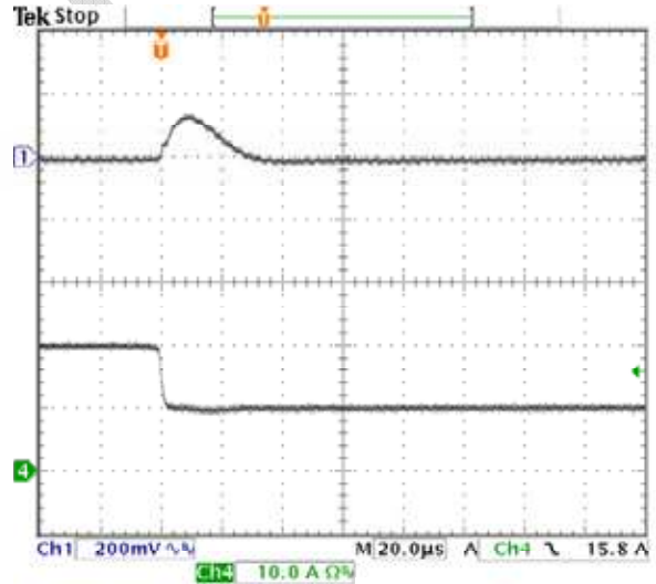
Fig-1.8V-7: Output voltage response for V_{out}=1.8V to positive load current step-change from 20A to 10A with slew rate of -5A/\mu s at V_{in}=12.0V . C_o=47\mu F \times 2 ceramic. Top trace: output voltage (200mV/div.) Bottom trace: load current (10A/div.) Time scale: 20µs/div.
