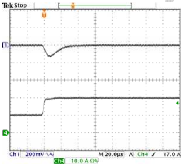
Fig-2.5V-6: Output voltage response for V_{out}=2.5V to positive load current step-change from 10A to 20A with slew rate of 5A/\mu s at V_{in}=12.0V . C_o=47\mu F \times 2 ceramic. Top trace: output voltage (200mV/div.) Bottom trace: load current (10A/div.) Time scale: 20μs/div.
