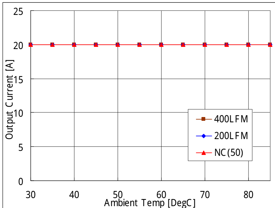
Fig-1.0V-1: Available load current vs. ambient temperature and airflow rates for Vout=1.0V with Vin=12.0V. Maximum component temperature ≤ 120°C
