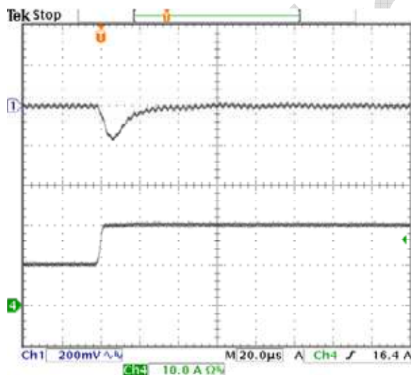
Fig-5.0V-6: Output voltage response for V_{out}=5.0V to positive load current step-change from 10A to 20A with slew rate of 5A/\mu s at V_{in}=12.0V . C_o=47\mu F \times 2 ceramic. Top trace: output voltage (200mV/div.) Bottom trace: load current (10A/div.) Time scale: 20\mu s /div.
