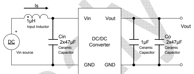
Fig. I: Test setup for measuring output voltage ripple
