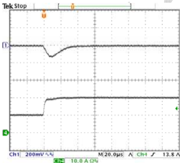
Fig-1.5V-6: Output voltage response for V_{out}=1.5V to positive load current step-change from 10A to 20A with slew rate of 5A/\mu s at V_{in}=12.0V . C_o=47\mu F \times 2 ceramic. Top trace: output voltage (200mV/div.) Bottom trace: load current (10A/div.) Time scale: 20μs/div.
