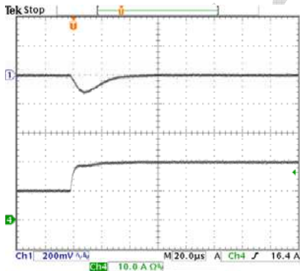
Fig-1.0V-6: Output voltage response for V_{out}=1.0V to positive load current step-change from 10A to 20A with slew rate of 5A/\mu s at V_{in}=12.0V . C_o=47\mu F \times 2 ceramic. Top trace: output voltage (200mV/div.) Bottom trace: load current (10A/div.) Time scale: 20µs/div.
