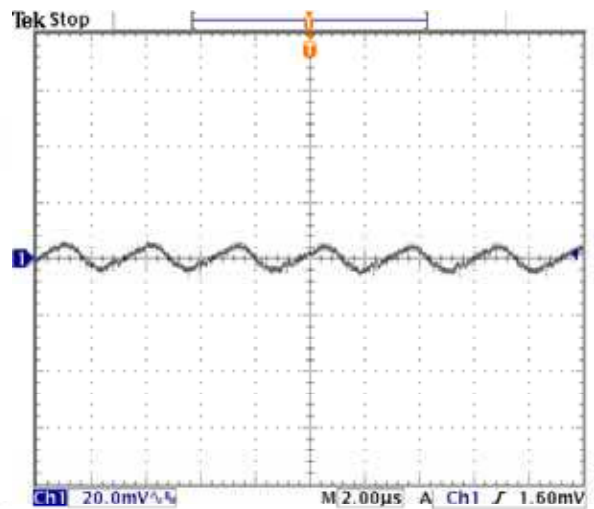
Fig-3.3V-5: Output voltage ripple (20mV/div.) for V_{out}=3.3V at full rated load current into a resistive load with external capacitance 47\mu F \times 2 ceramic + 1\mu F ceramic at V_{in}=12.0V . Time scale: 2μs/div
