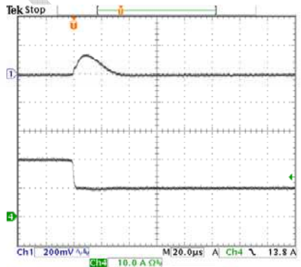
Fig-1.5V-7: Output voltage response for V_{out}=1.5V to positive load current step-change from 20A to 10A with slew rate of -5A/\mu s at V_{in}=12.0V . C_o=47\mu F \times 2 ceramic. Top trace: output voltage (200mV/div.) Bottom trace: load current (10A/div.) Time scale: 20μs/div.
