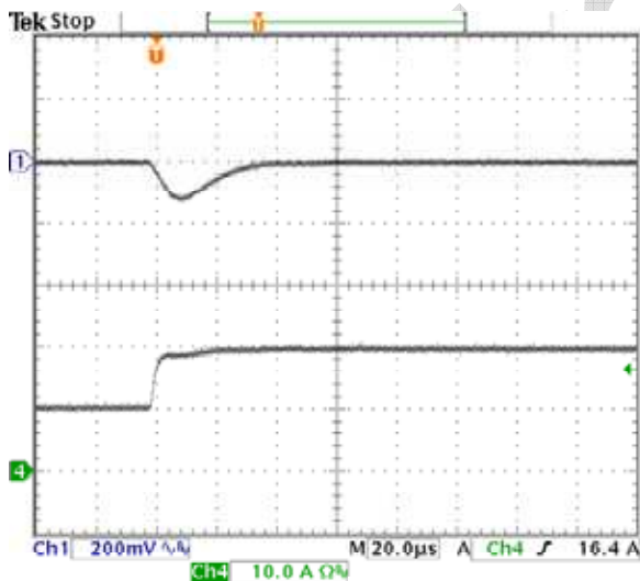
Fig-1.2V-6: Output voltage response for V_{out}=1.2V to positive load current step-change from 10A to 20A with slew rate of 5A/\mu s at V_{in}=12.0V . C_o=47\mu F \times 2 ceramic. Top trace: output voltage (200mV/div.) Bottom trace: load current (10A/div.) Time scale: 20μs/div.
