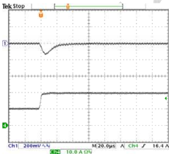
Fig-3.3V-6: Output voltage response for V_{out}=3.3V to positive load current step-change from 10A to 20A with slew rate of 5A/\mu s at V_{in}=12.0V . C_o=47\mu F \times 2 ceramic. Top trace: output voltage (200mV/div.) Bottom trace: load current (10A/div.) Time scale: 20μs/div.
