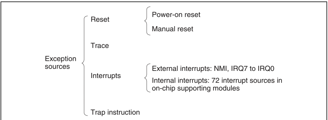
Figure 4.1 Exception Sources
