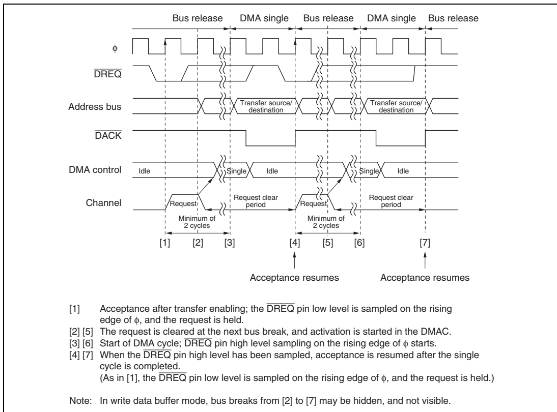
Figure 8.31 Example of DREQ Pin Falling Edge Activated Single Address Mode Transfer
