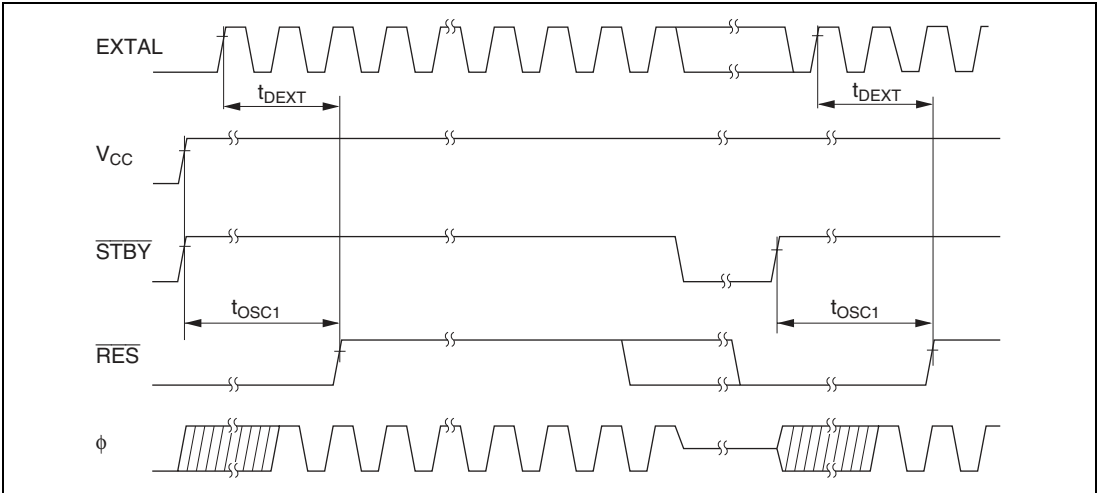
Figure 27.3 Oscillator Settling Timing
