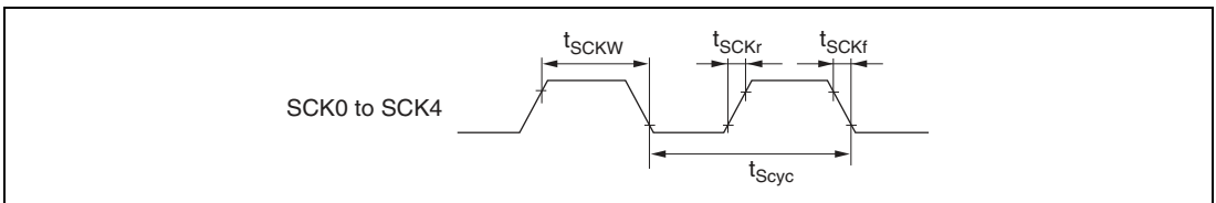
Figure 25.30 SCK Clock Input Timing
