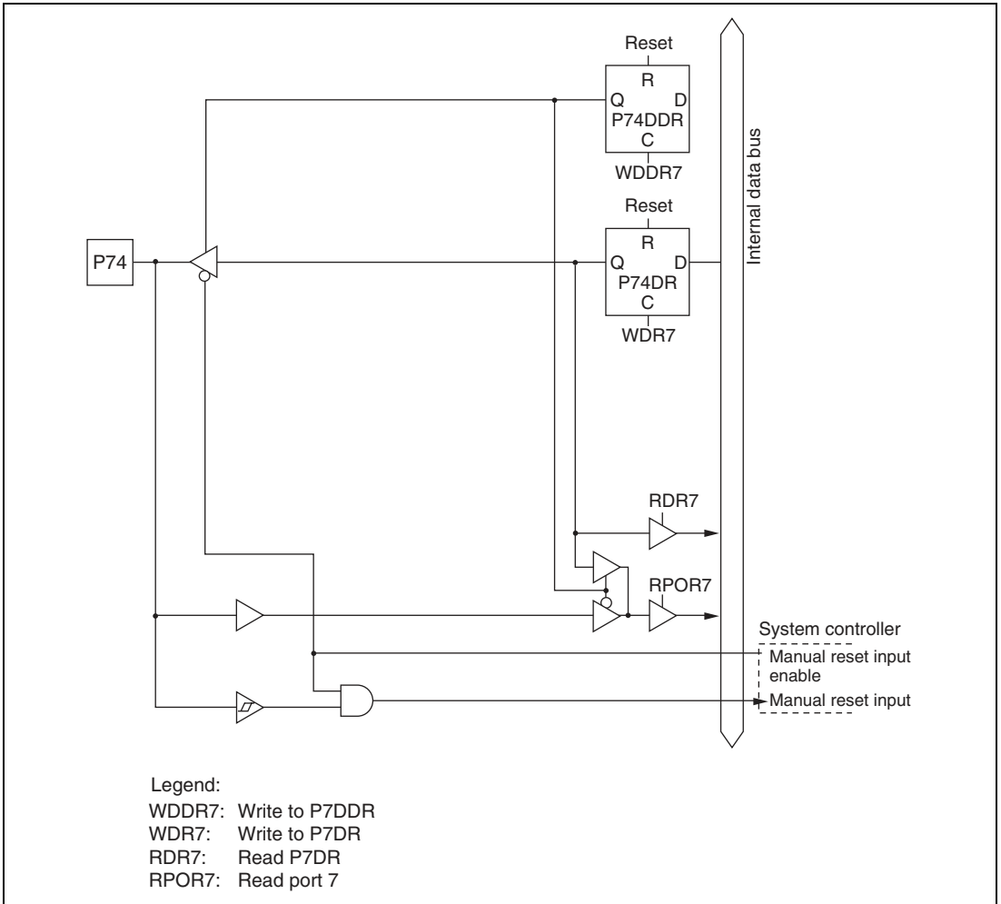
Figure C.16 (b) Port 7 Block Diagram (Pin P74)
