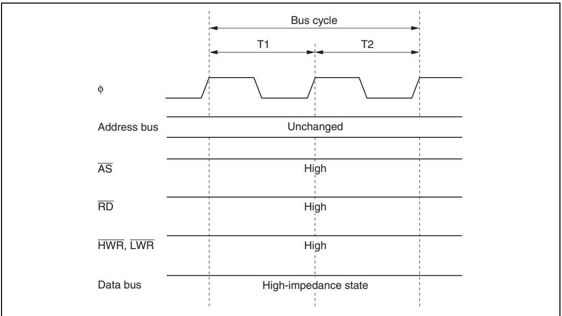
Figure 2.20 Pin States during On-Chip Supporting Module Access
