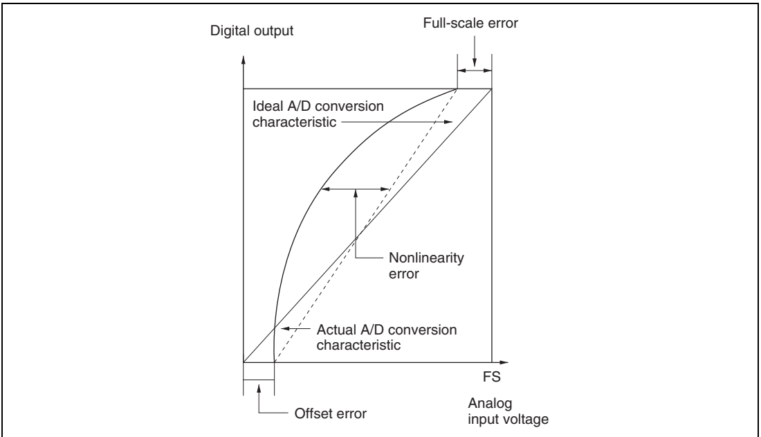
Figure 19.10 A/D Conversion Precision Definitions (2)
