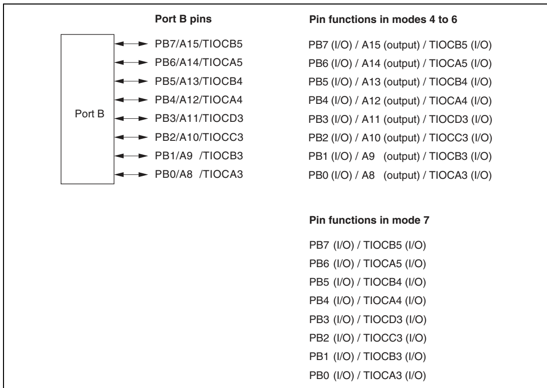
Figure 10B.7 Port B Pin Functions
