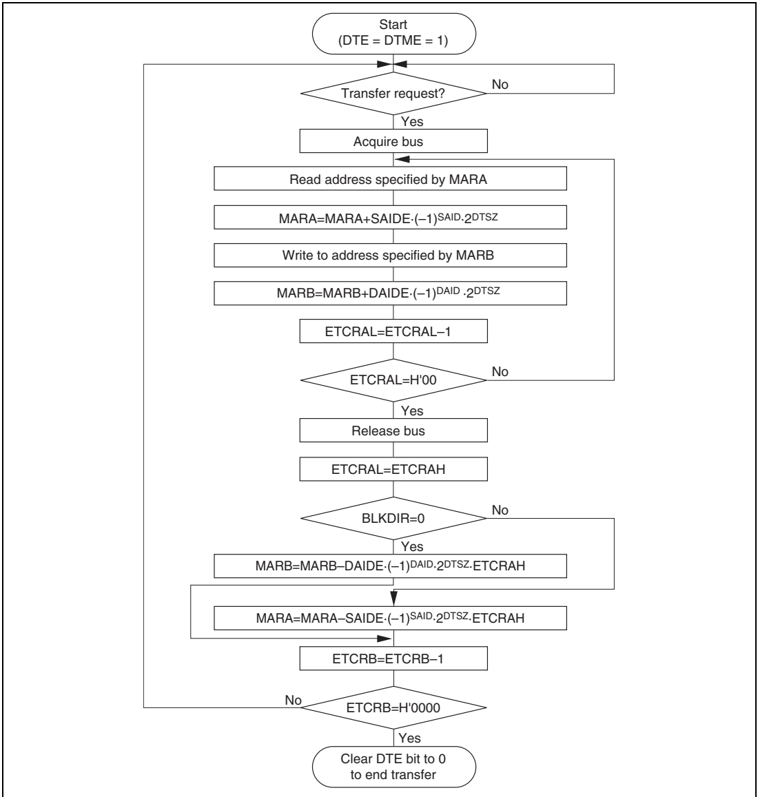
Figure 8.15 Operation Flow in Block Transfer Mode
