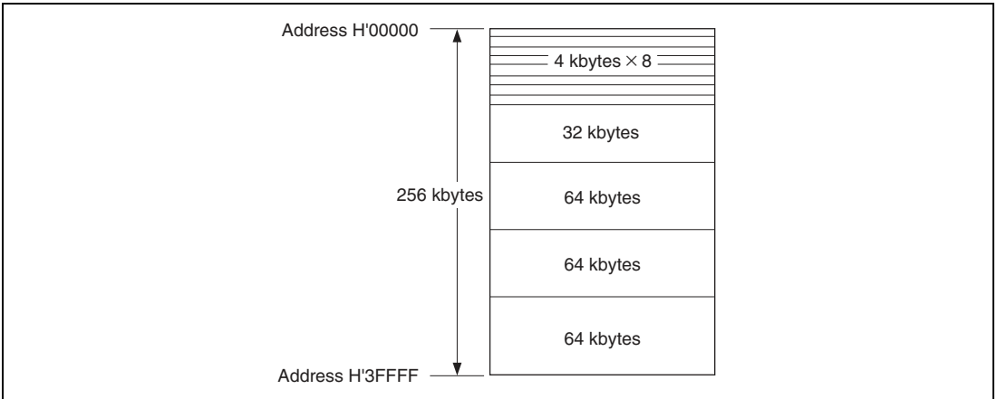
Figure 22.6 Flash Memory Block Configuration
