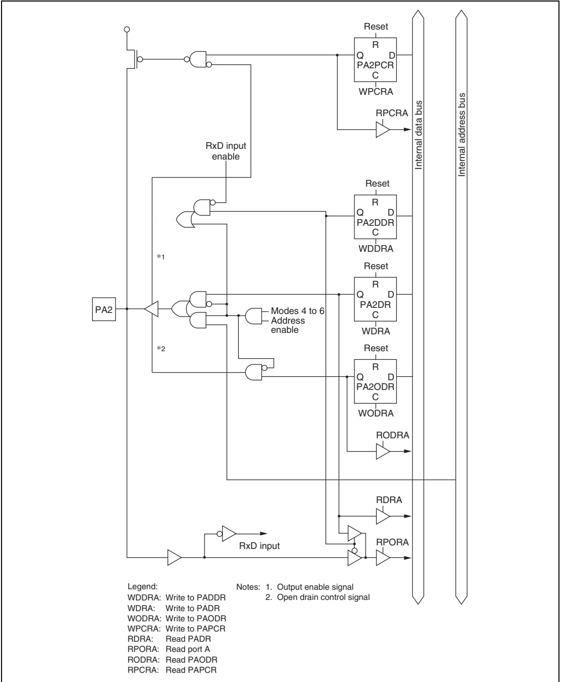
Figure C.6 (c) Port A Block Diagram (Pin PA2)
