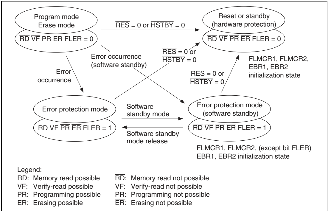
Figure 22.15 Flash Memory State Transitions
