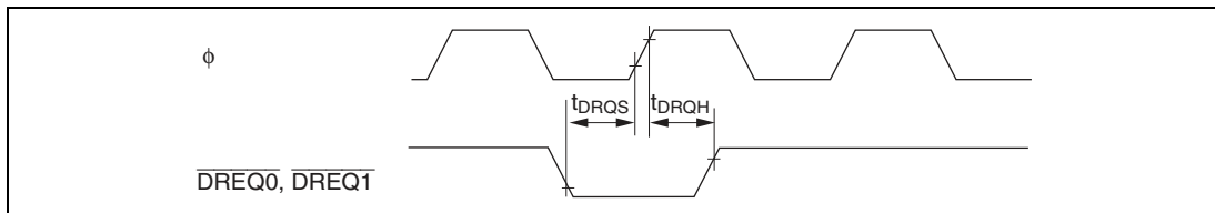
Figure 26.19 DMAC DREQ Input Timing
