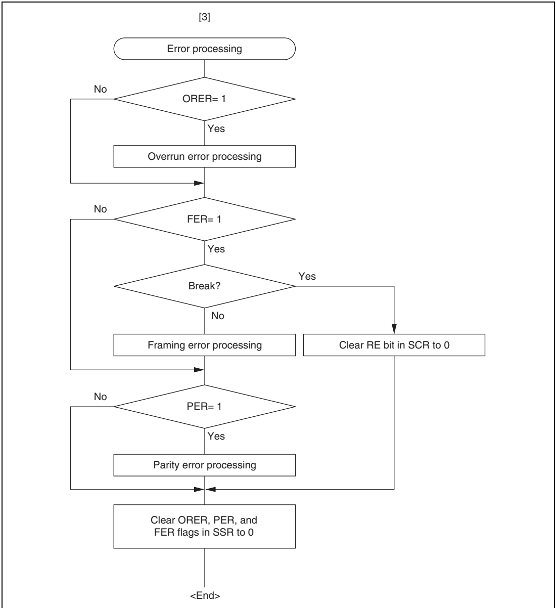
Figure 16.7 Sample Serial Reception Data Flowchart (cont)
