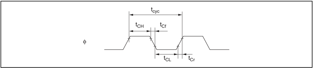
Figure 26.2 System Clock Timing
