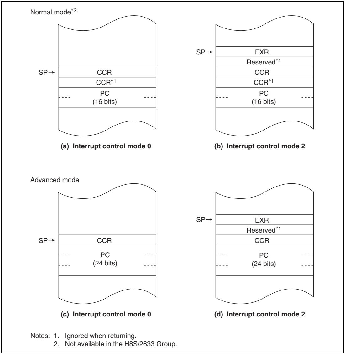
Figure 2.16 Stack Structure after Exception Handling (Examples)
