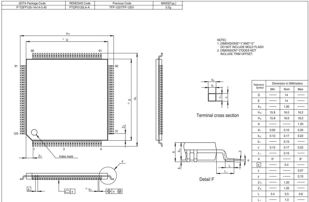
Figure G.1 TFP-120 Package Dimensions
