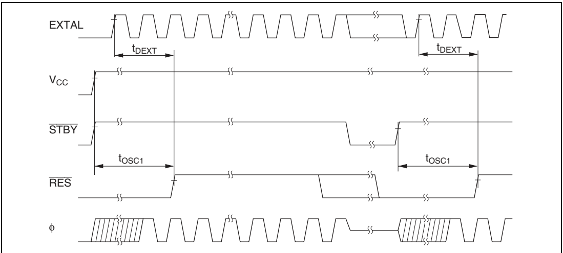
Figure 26.3 Oscillator Settling Timing
