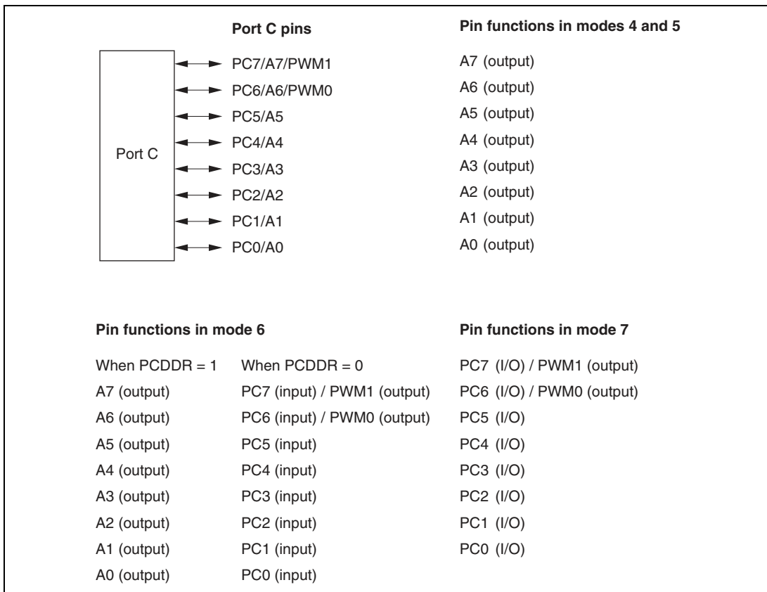
Figure 10A.8 Port C Pin Functions
