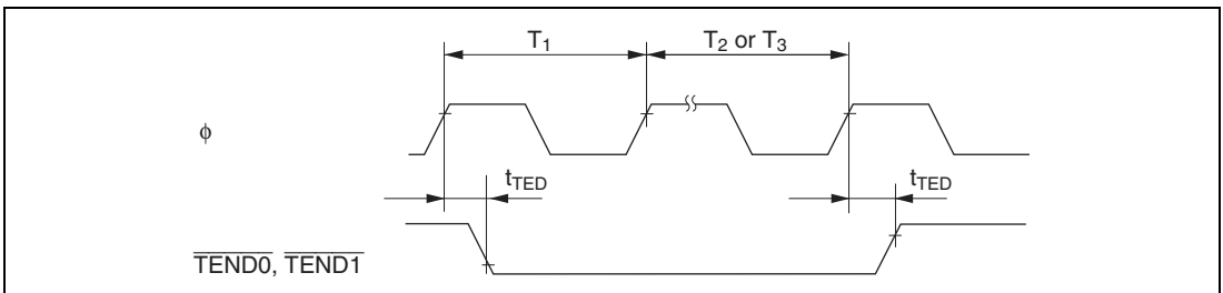
Figure 25.18 DMAC TEND Output Timing
