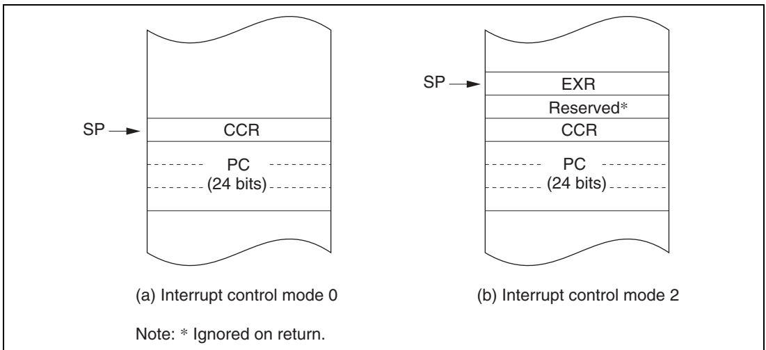
Figure 4.5 (2) Stack Status after Exception Handling (Advanced Modes)
