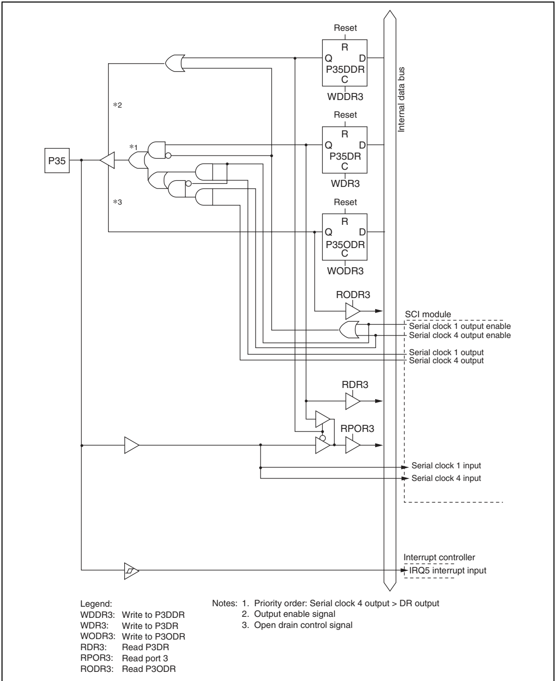
Figure C.14 (f) Port 3 Block Diagram (Pin P35)
