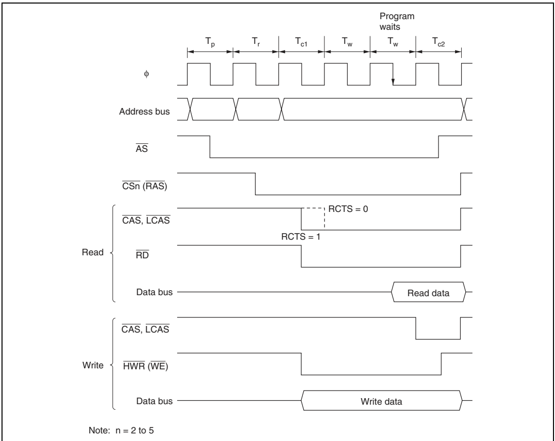
Figure 7.17 Example Program Wait Insertion Timing (Wait 2 State Insertion)
