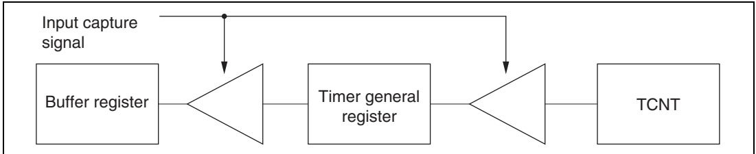
Figure 11.17 Input Capture Buffer Operation
