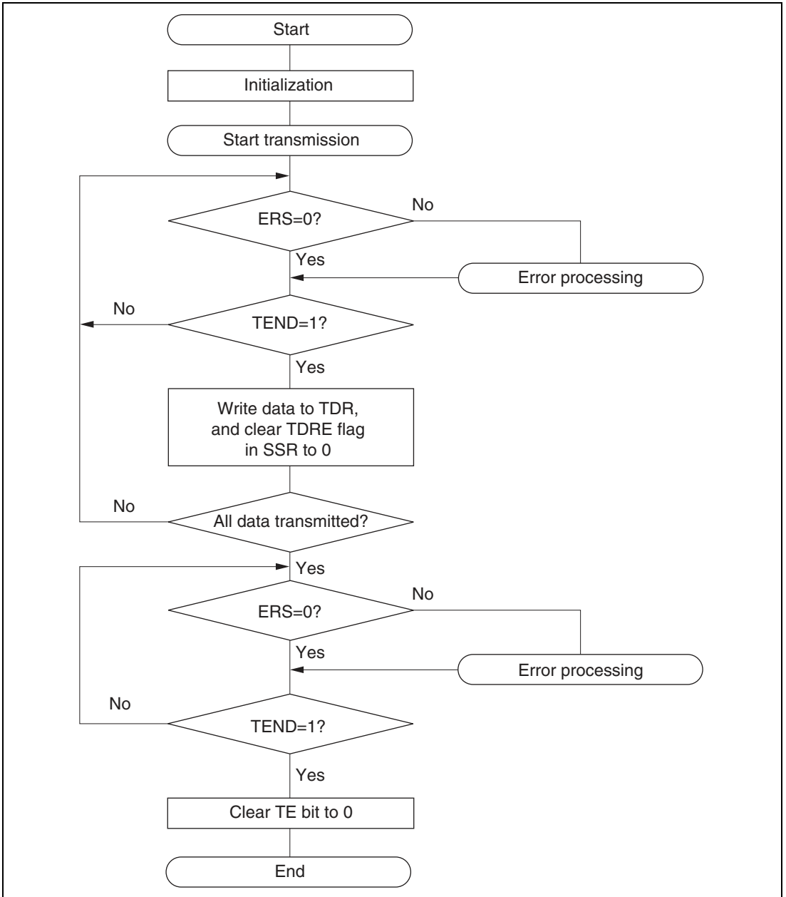
Figure 17.4 Example of Transmission Processing Flow
