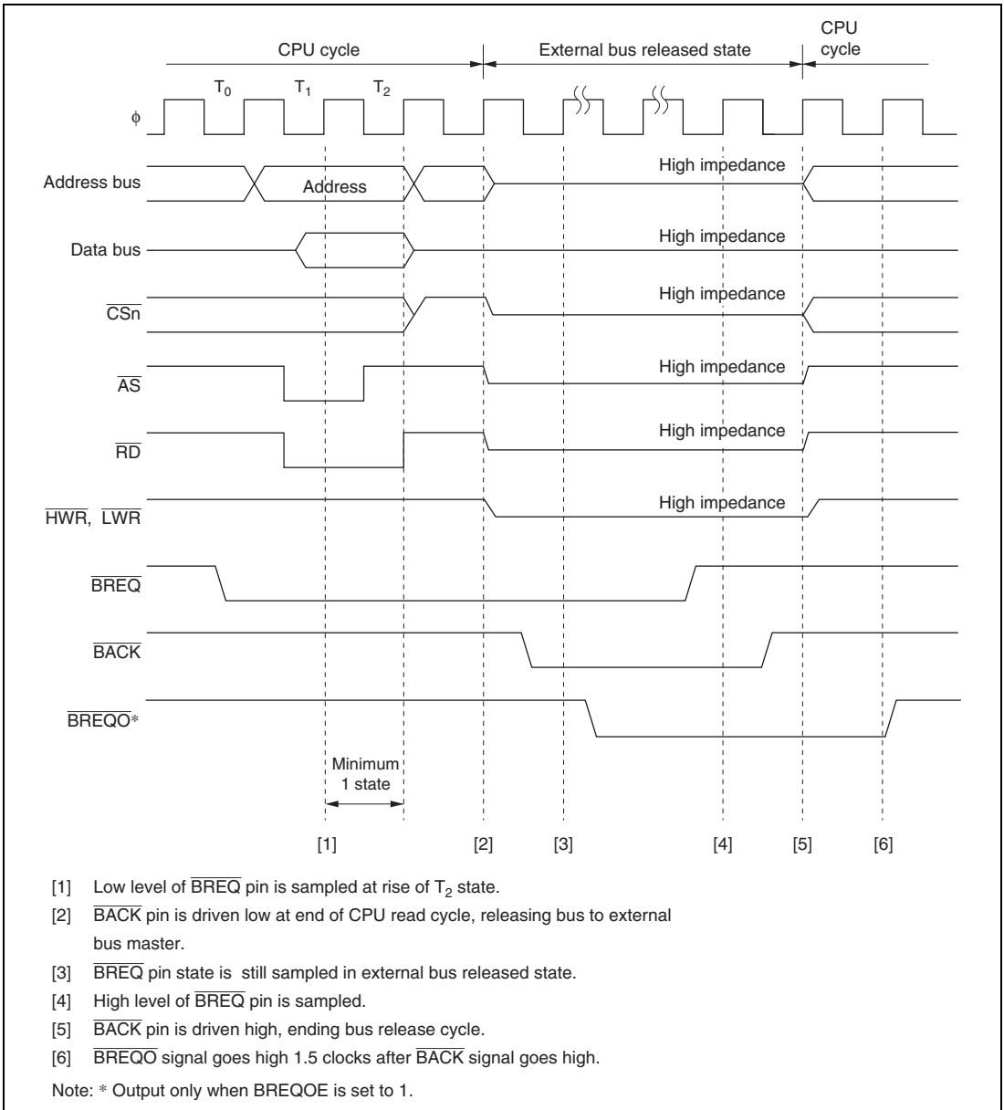
Figure 7.39 Bus-Released State Transition Timing
