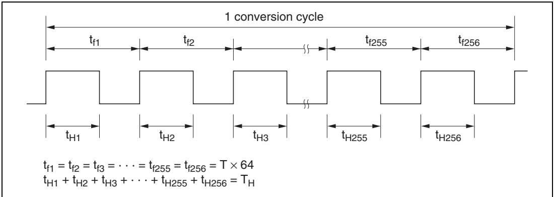
Figure 14.4 (3) Output Waveform
