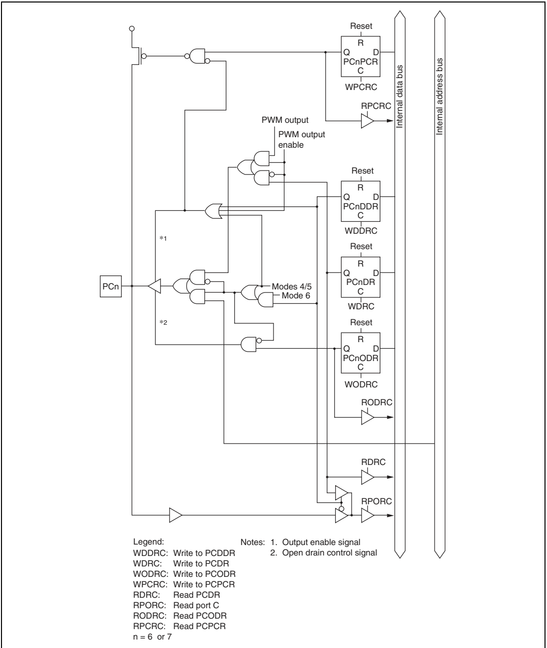
Figure C.8 (b) Port C Block Diagram (Pins PC6 and PC7)
