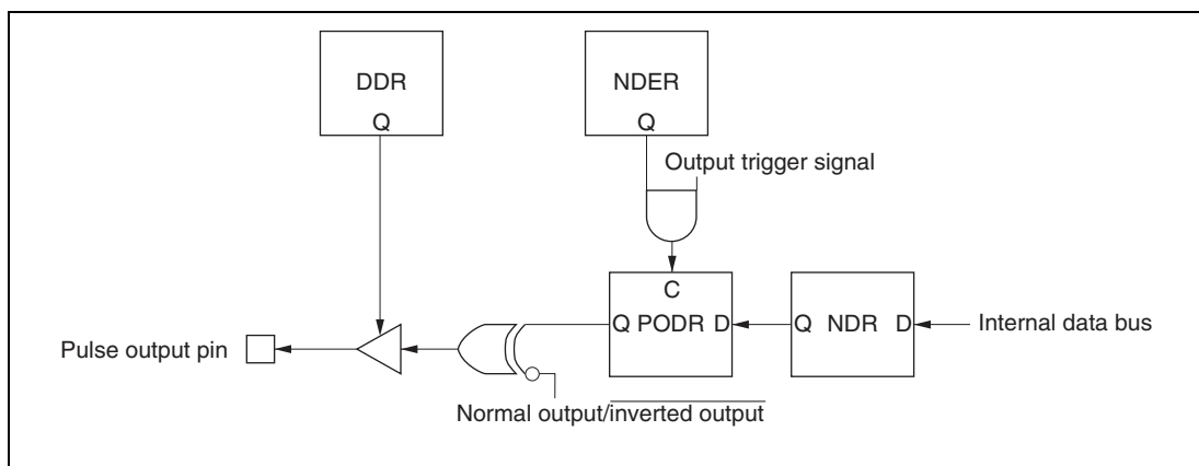
Figure 12.2 PPG Output Operation
