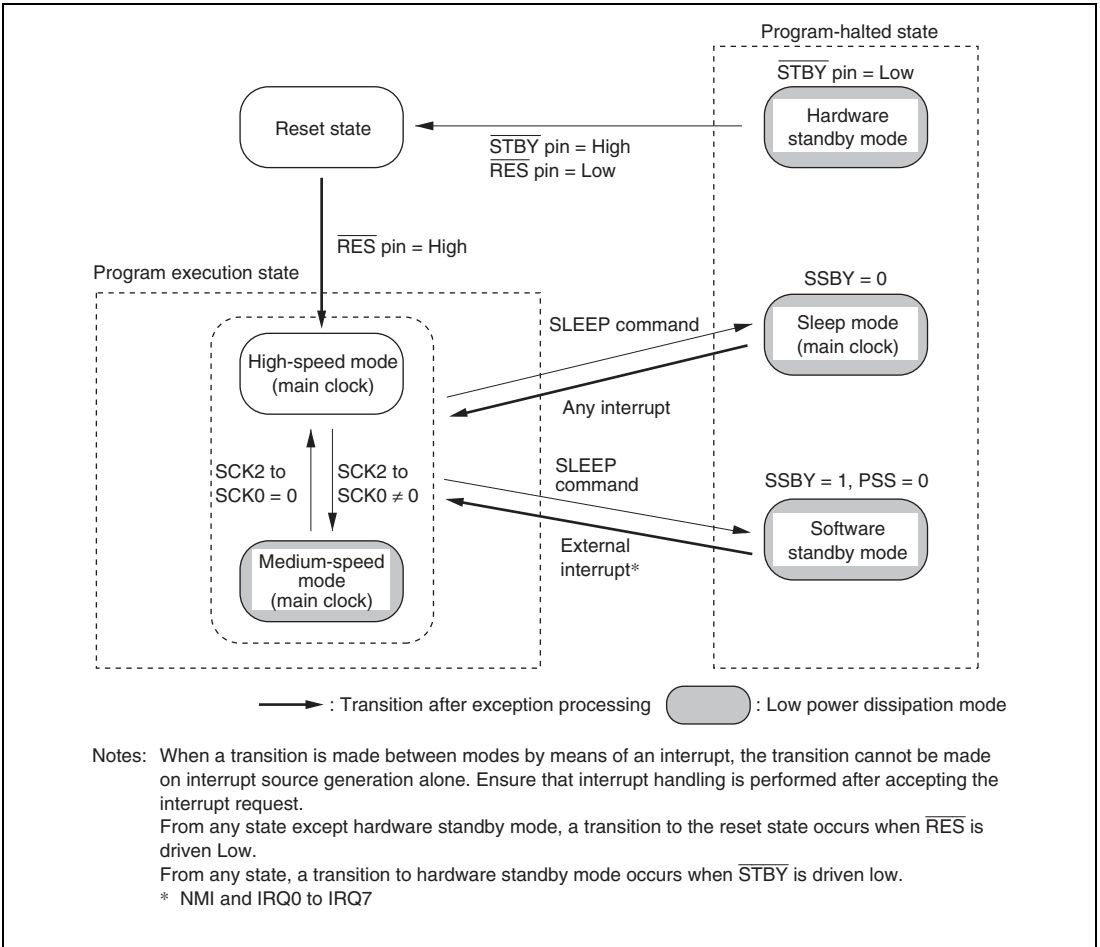
Figure 24.1 (b) Mode Transition Diagram (H8S/2695)
