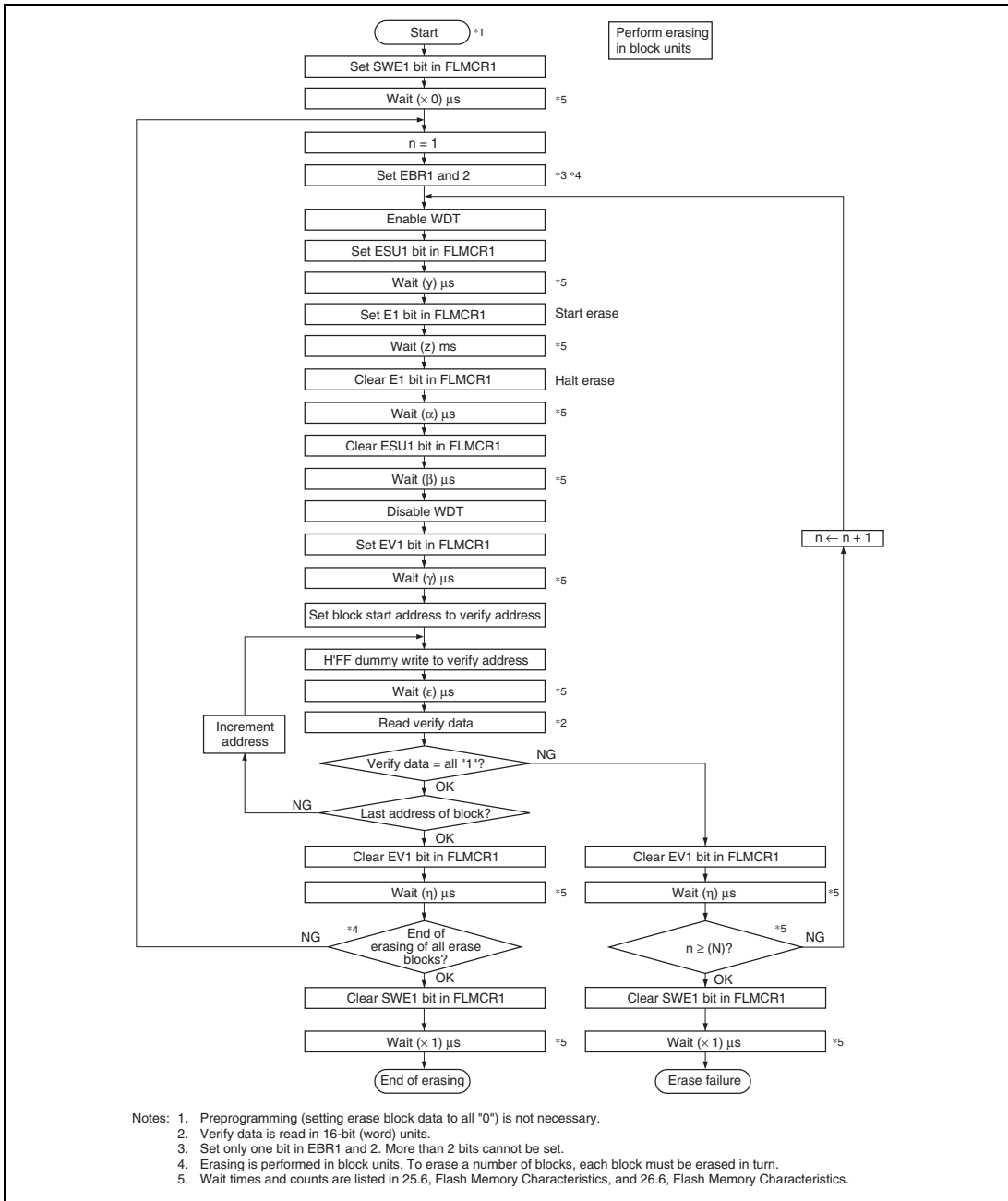
Figure 22.14 Erase/Erase-Verify Flowchart
