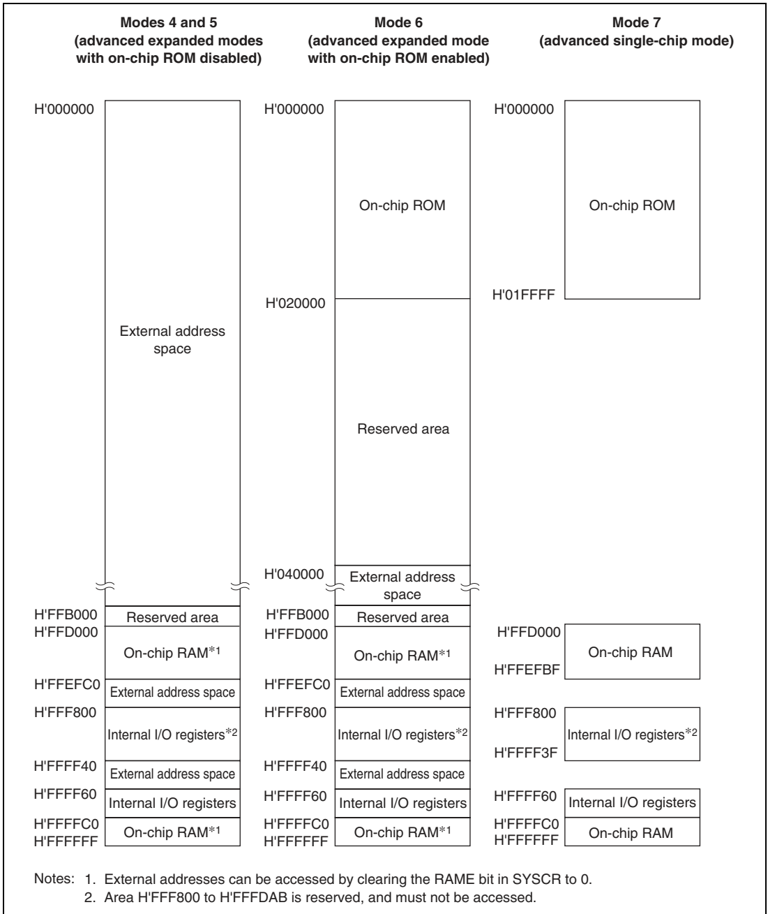
Figure 3.3 Memory Map in Each Operating Mode in the H8S/2631
