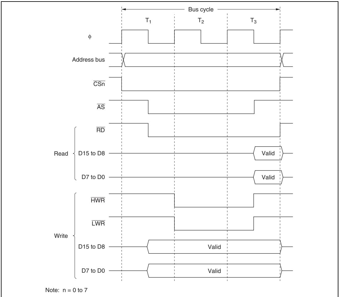
Figure 7.13 Bus Timing for 16-Bit 3-State Access Space (3) (Word Access)
