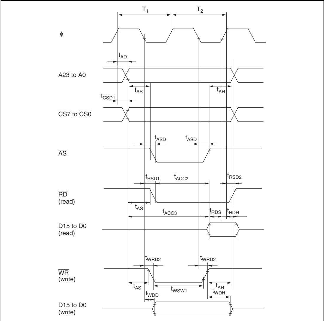
Figure 26.6 Basic Bus Timing (Two-State Access)
