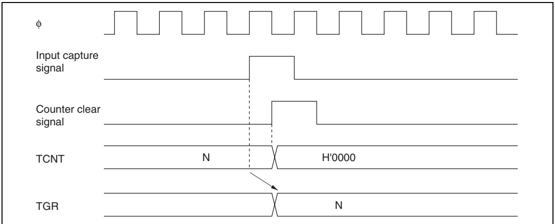
Figure 11.39 Counter Clear Timing (Input Capture)
