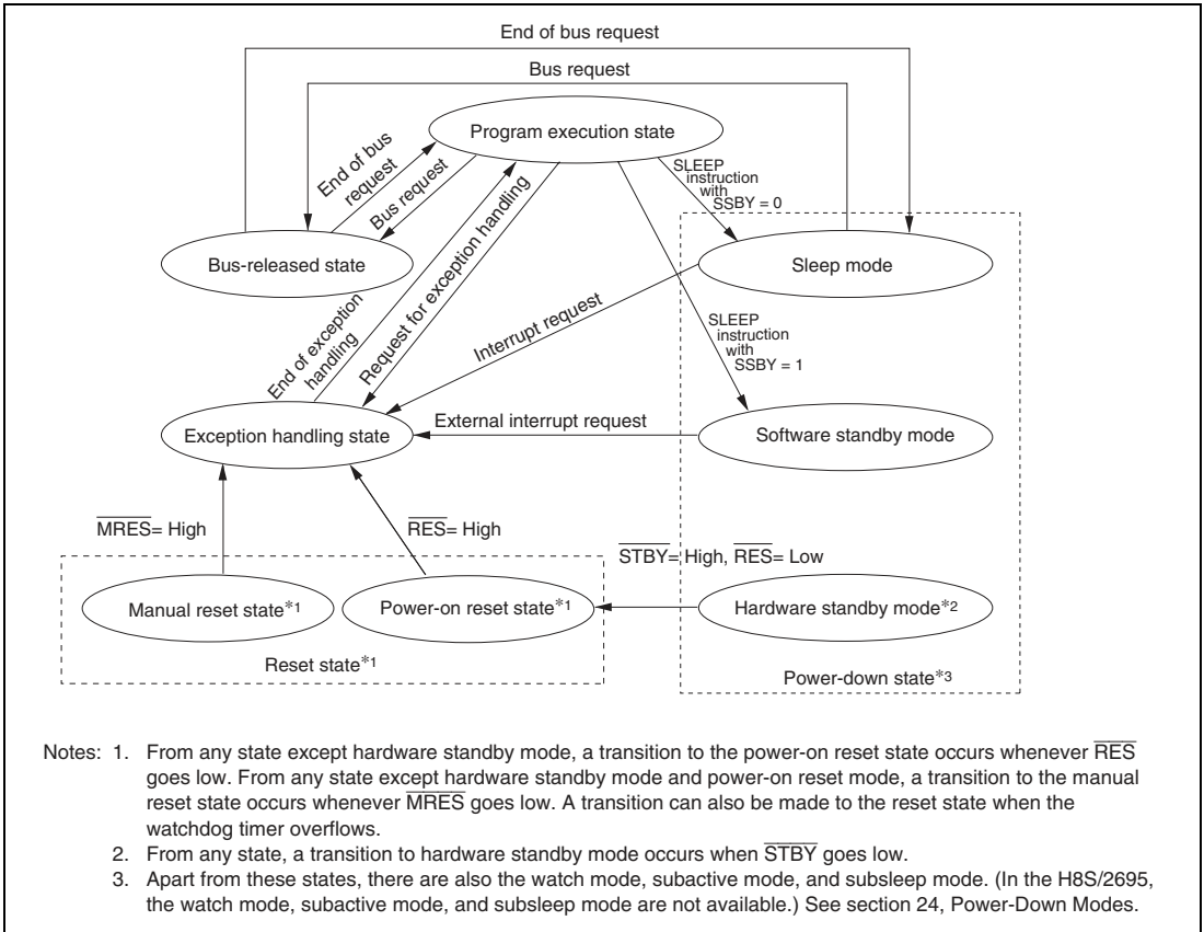
Figure 2.15 State Transitions
