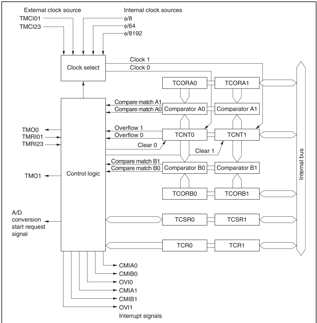
Figure 13.1 Block Diagram of 8-Bit Timer
