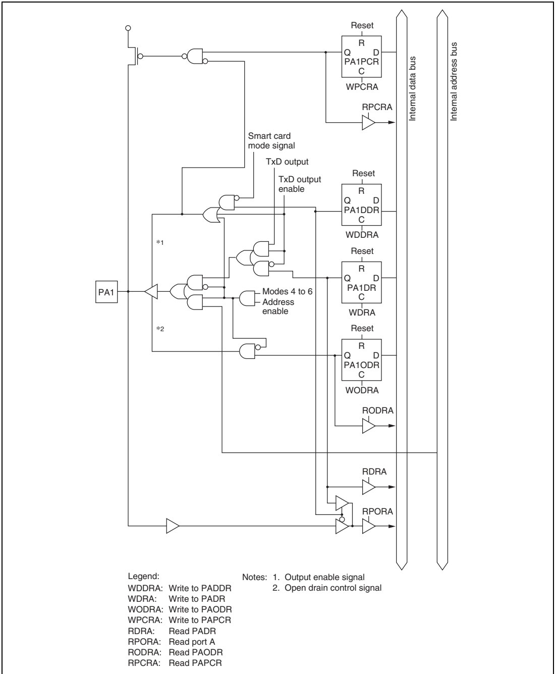
Figure C.18 (b) Port A Block Diagram (Pin PA1)
