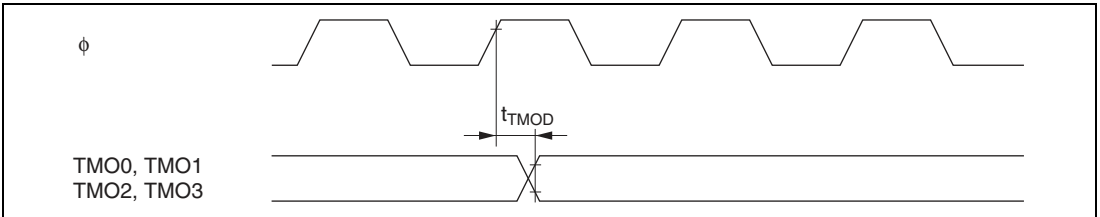
Figure 26.24 8-bit Timer Output Timing
