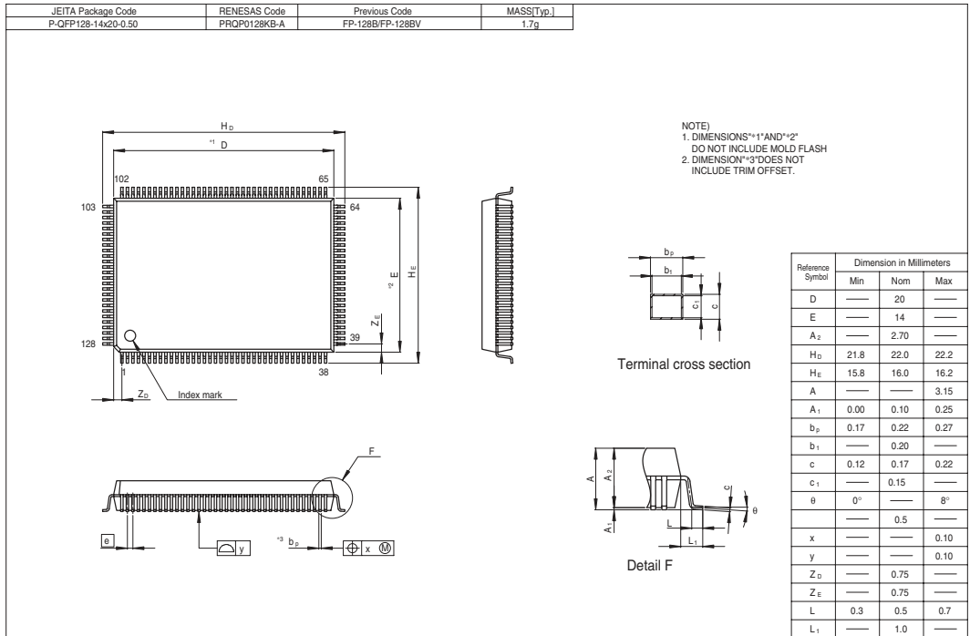
Figure G.2 FP-128B Package Dimensions
