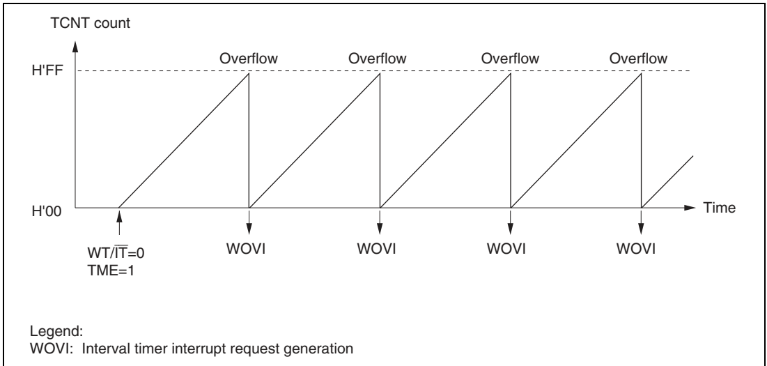
Figure 15.5 Interval Timer Operation
