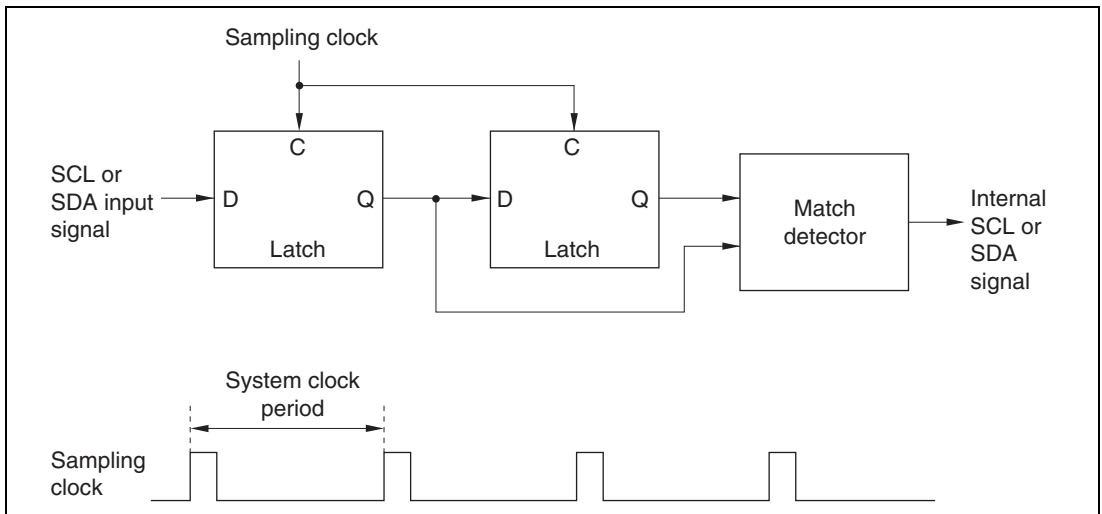
Figure 18.20 Block Diagram of Noise Canceler
