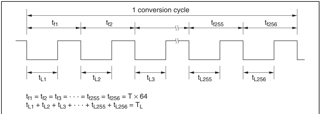
Figure 14.4 (1) Output Waveform
