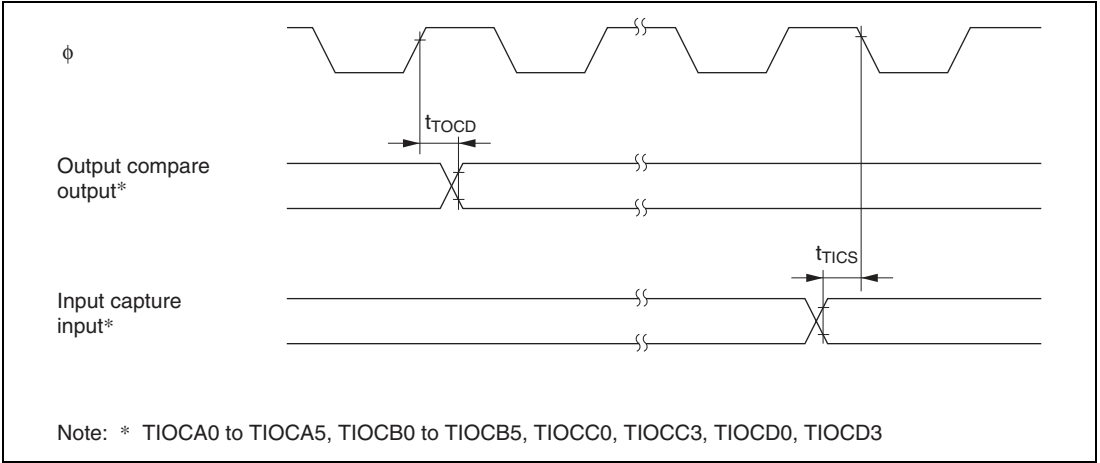
Figure 26.22 TPU Input/Output Timing
