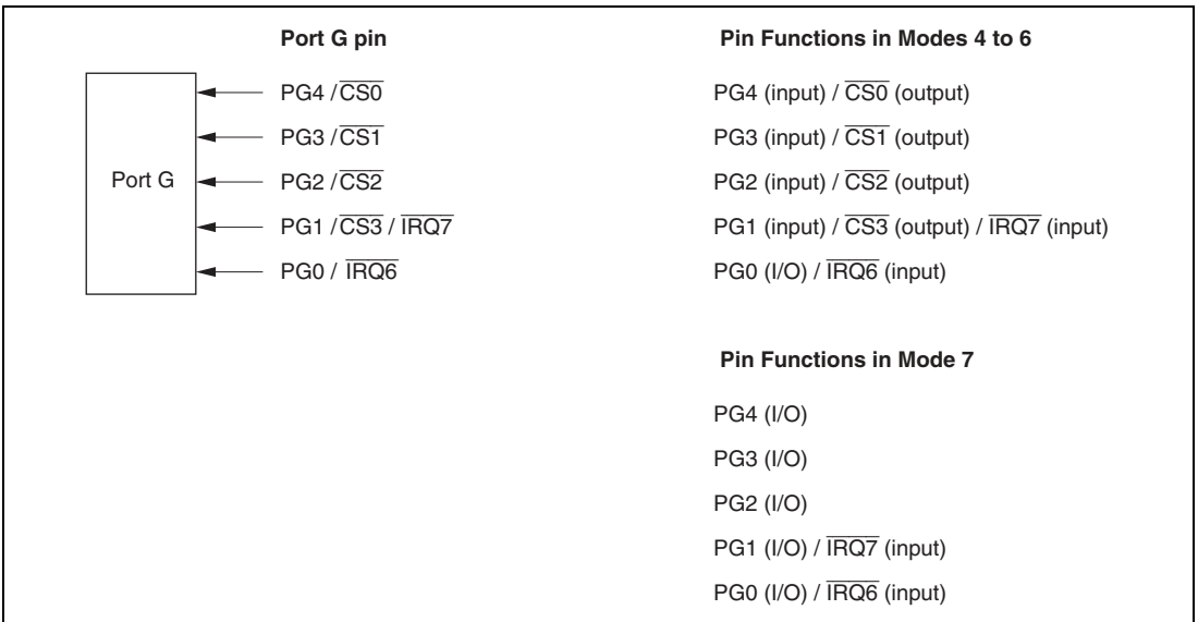
Figure 10B.19 Port G Pin Functions
