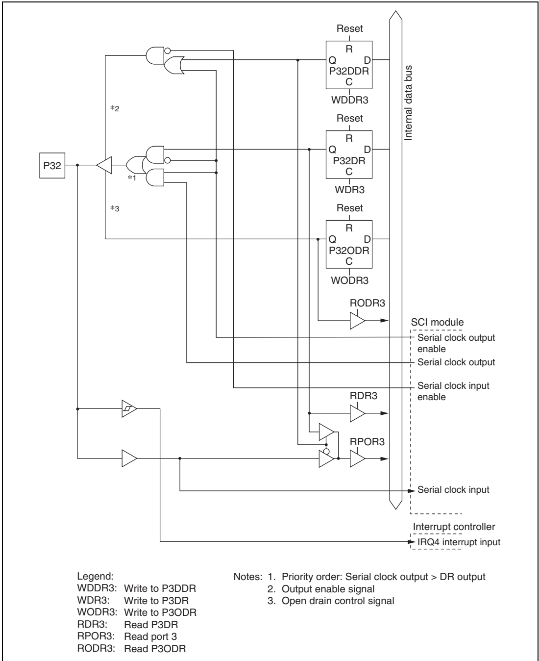
Figure C.14 (c) Port 3 Block Diagram (Pin P32)
