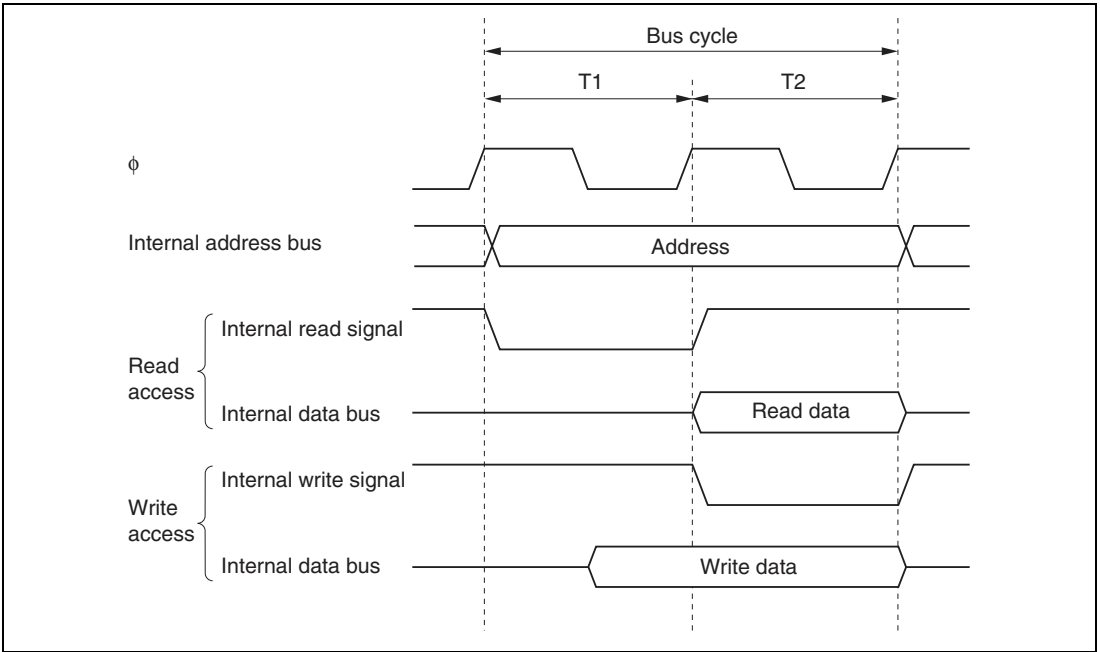
Figure 2.19 On-Chip Supporting Module Access Cycle
