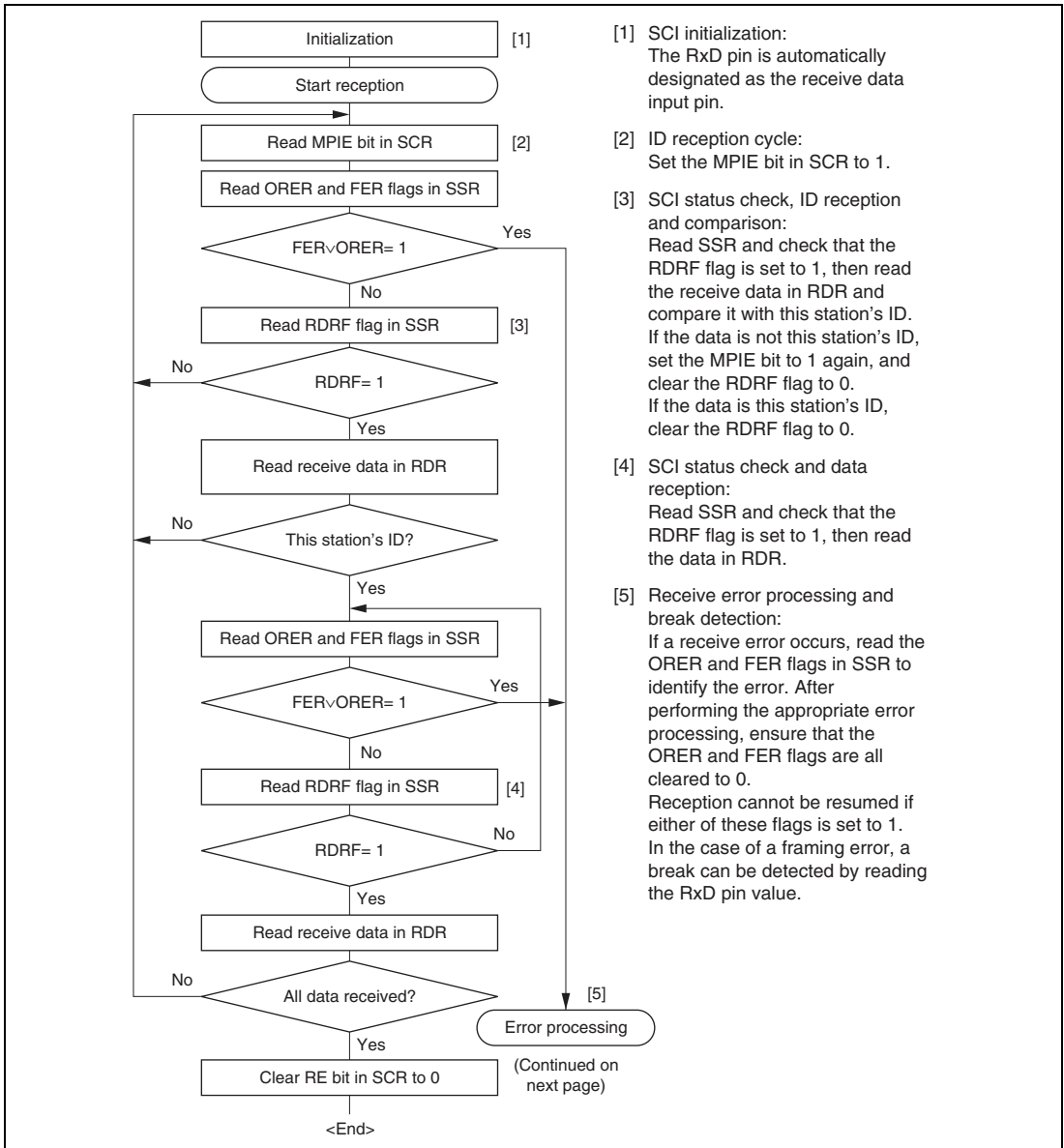
Figure 16.12 Sample Multiprocessor Serial Reception Flowchart
