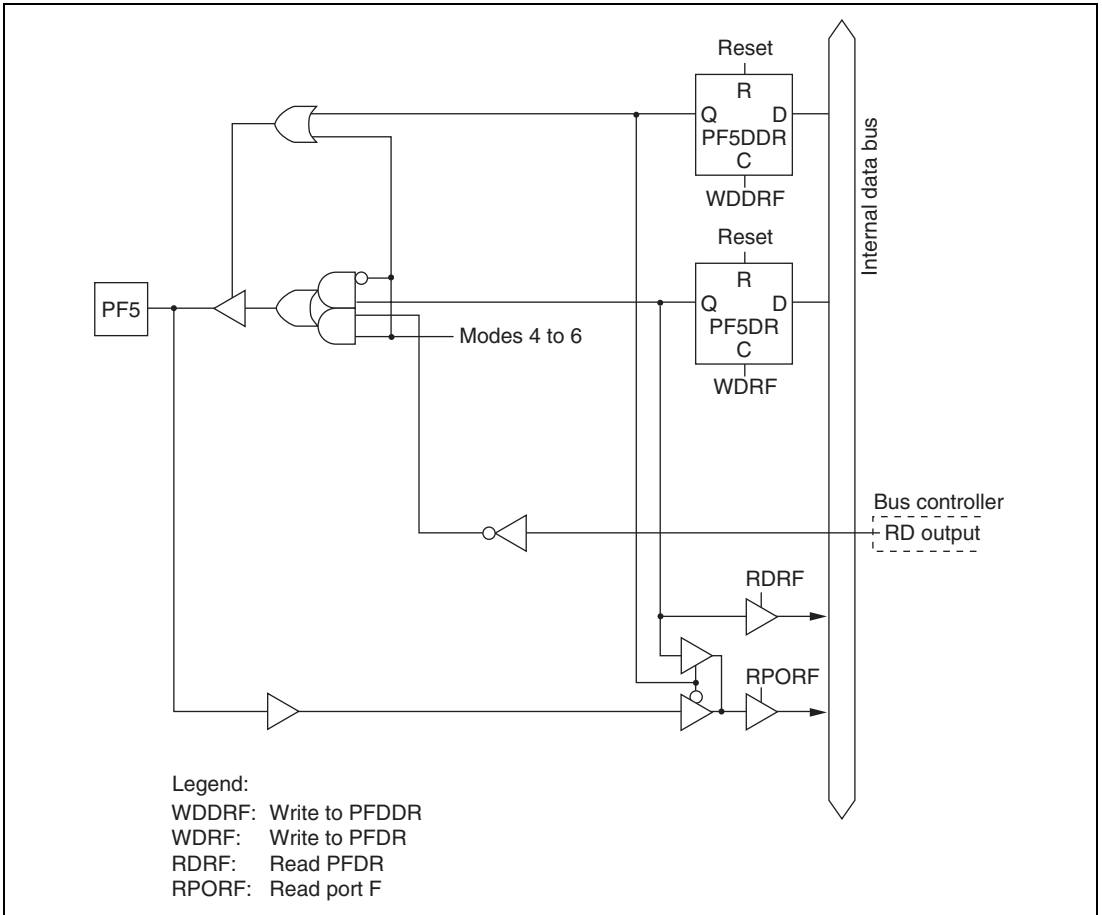
Figure C.23 (f) Port F Block Diagram (Pin PF5)
