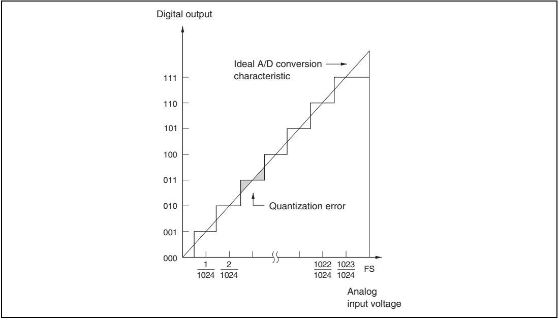
Figure 19.9 A/D Conversion Precision Definitions (1)
