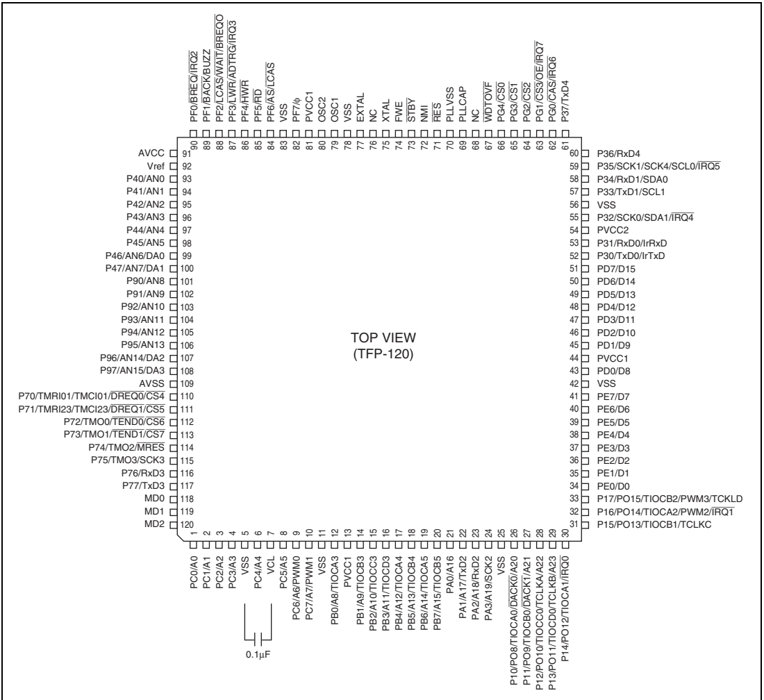
Figure 1.2 (b) H8S/2633R Pin Arrangement (TFP-120: Top View)
