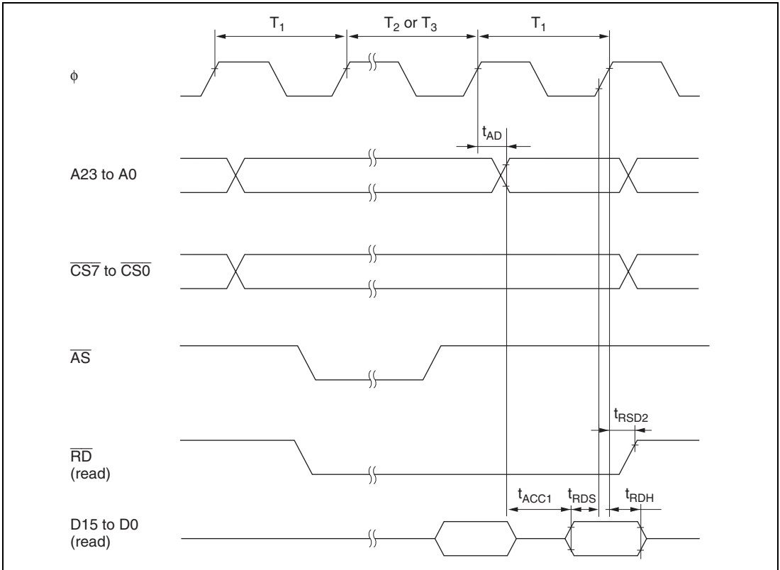
Figure 25.10 Burst ROM Access Timing (One-State Access)
