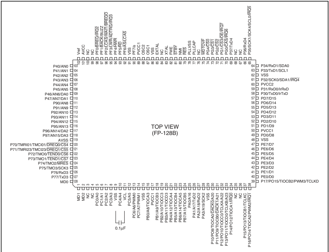
Figure 1.3 (b) H8S/2633R Pin Arrangement (FP-128B: Top View)
