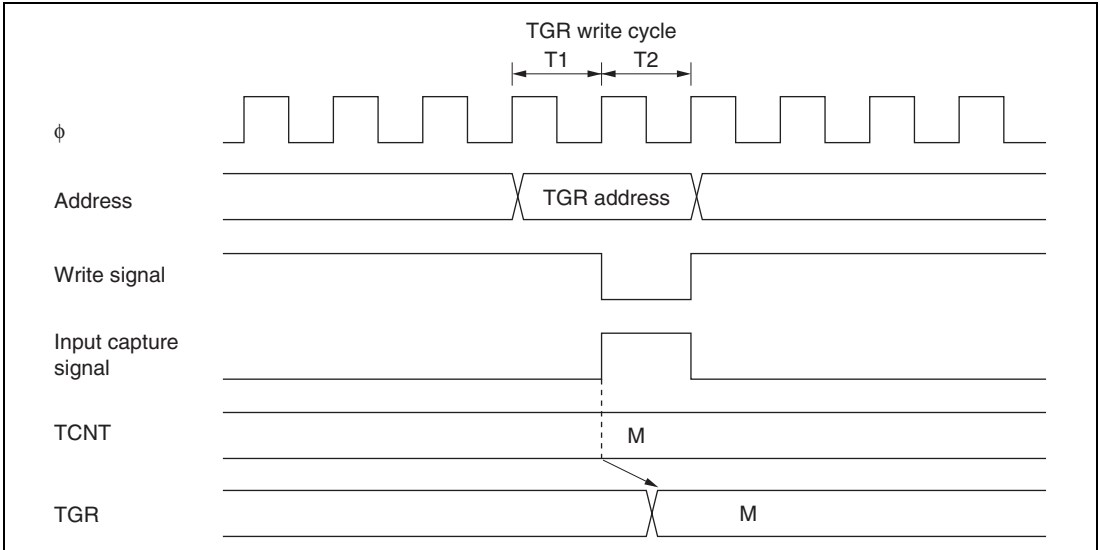
Figure 11.54 Contention between TGR Write and Input Capture
