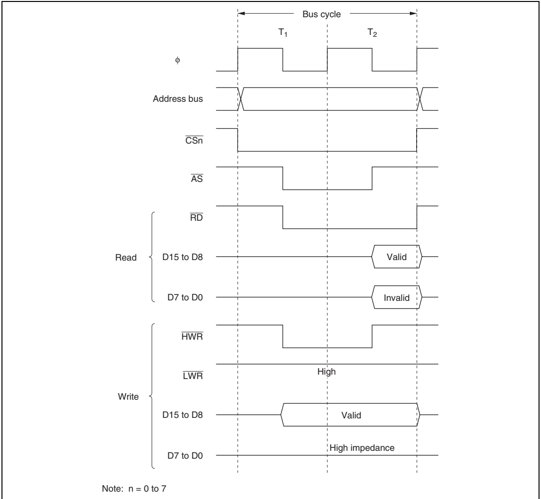
Figure 7.6 Bus Timing for 8-Bit 2-State Access Space
