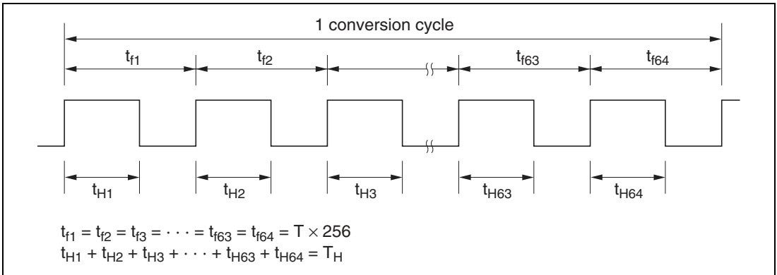
Figure 14.4 (4) Output Waveform
