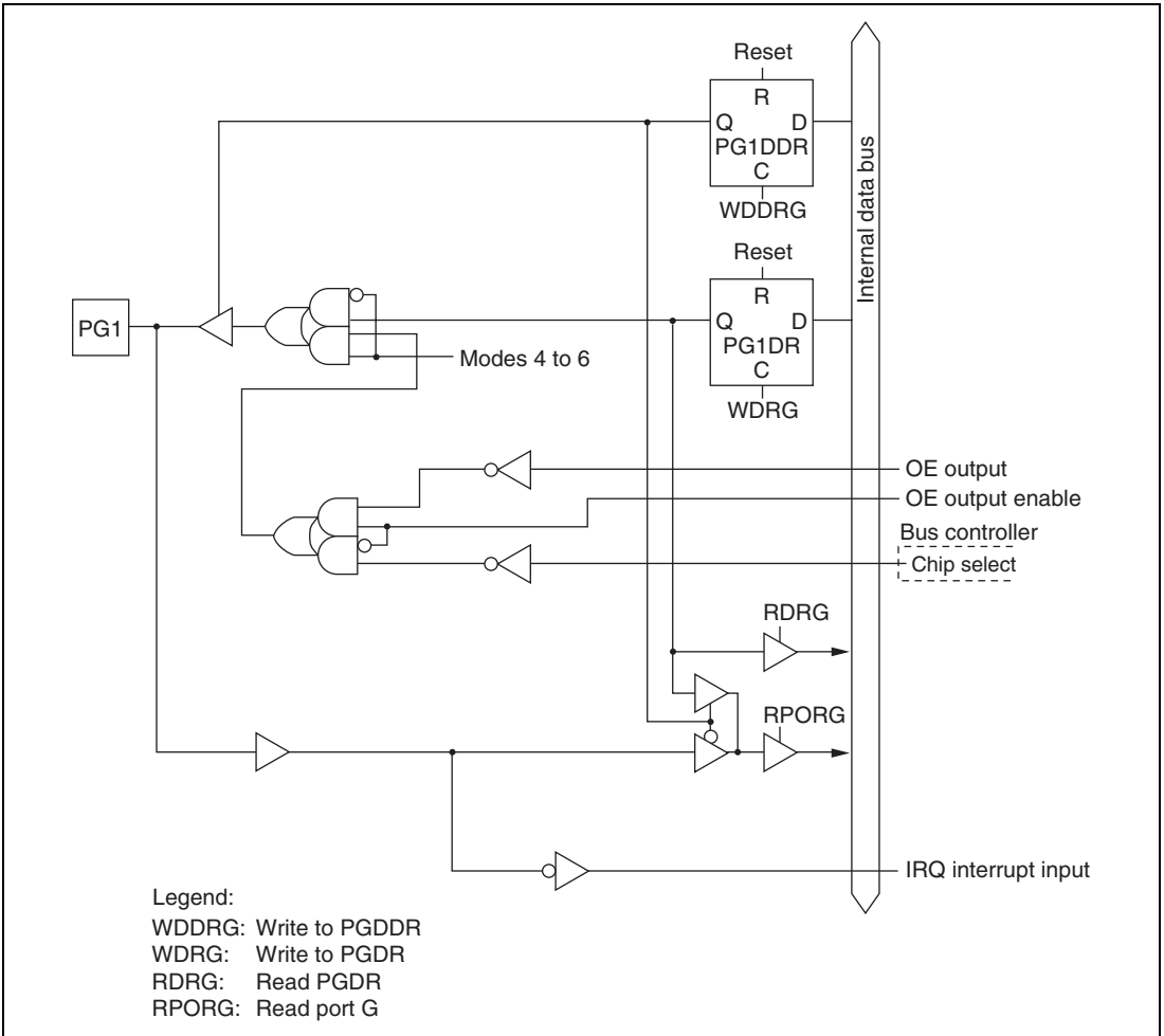
Figure C.12 (b) Port G Block Diagram (Pin PG1)
