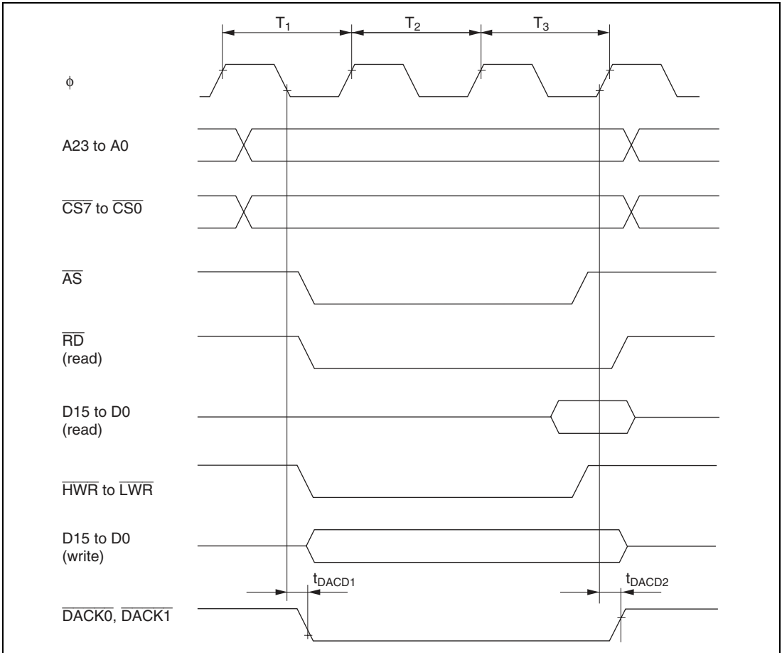
Figure 25.17 DMAC Single Address Transfer Timing / Three-State Access
