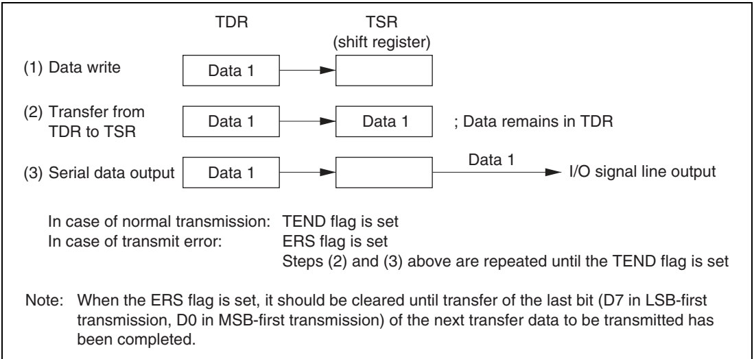
Figure 17.5 Relation Between Transmit Operation and Internal Registers
