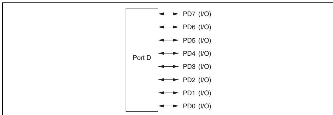
Figure 10B.14 Port D Pin Functions (Mode 7)
