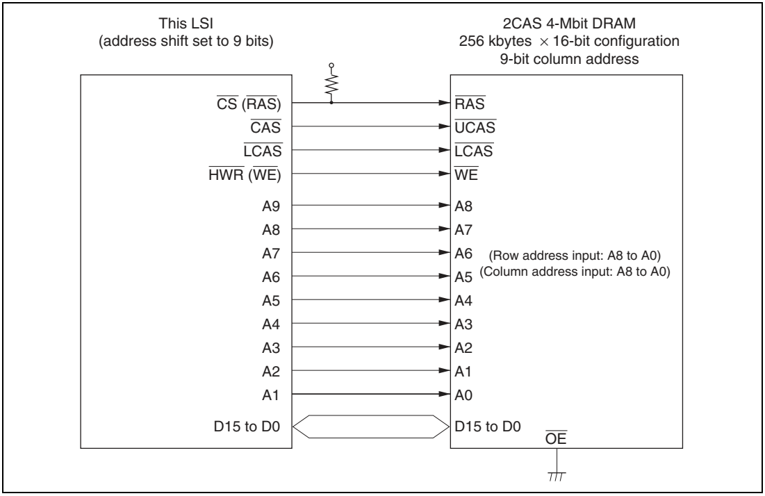
Figure 7.20 High-speed Page Mode DRAM
