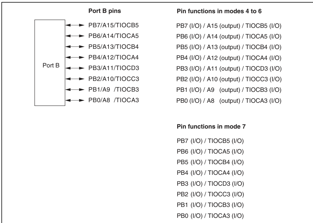
Figure 10A.7 Port B Pin Functions
