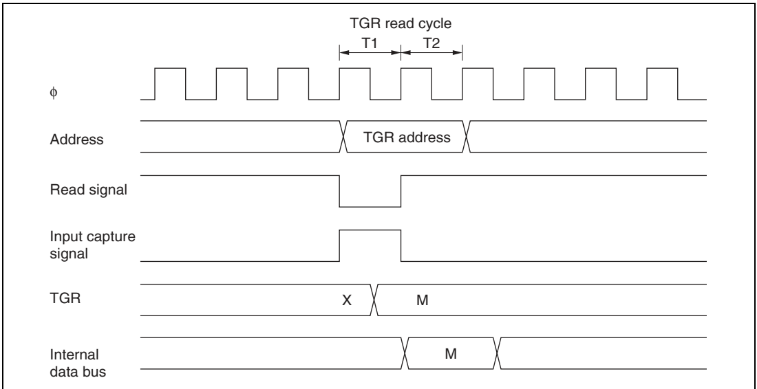
Figure 11.53 Contention between TGR Read and Input Capture
