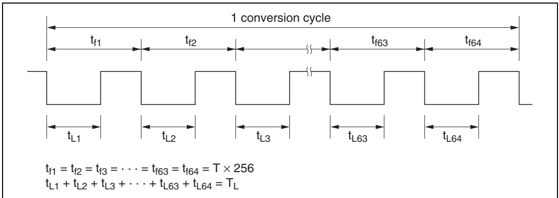
Figure 14.4 (2) Output Waveform
