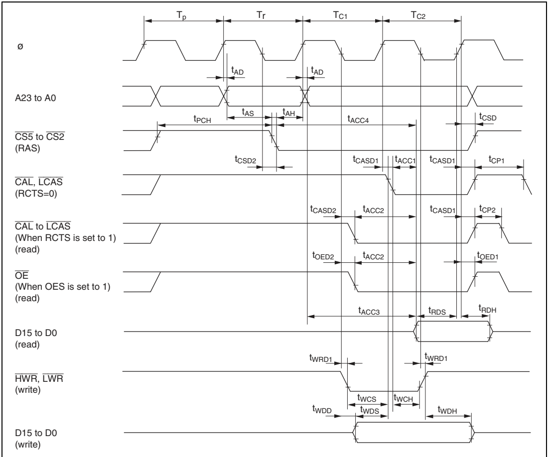
Figure 26.11 DRAM Access Timing
