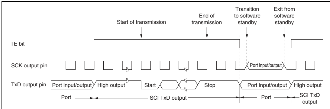
Figure 16.26 Asynchronous Transmission Using Internal Clock
