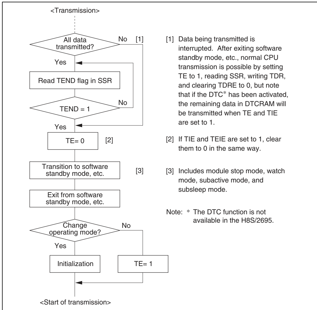
Figure 16.25 Sample Flowchart for Mode Transition during Transmission
