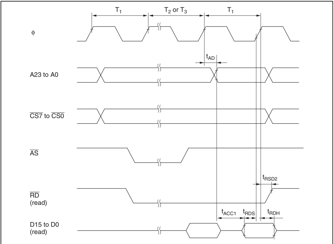
Figure 27.10 Burst ROM Access Timing (One-State Access)
