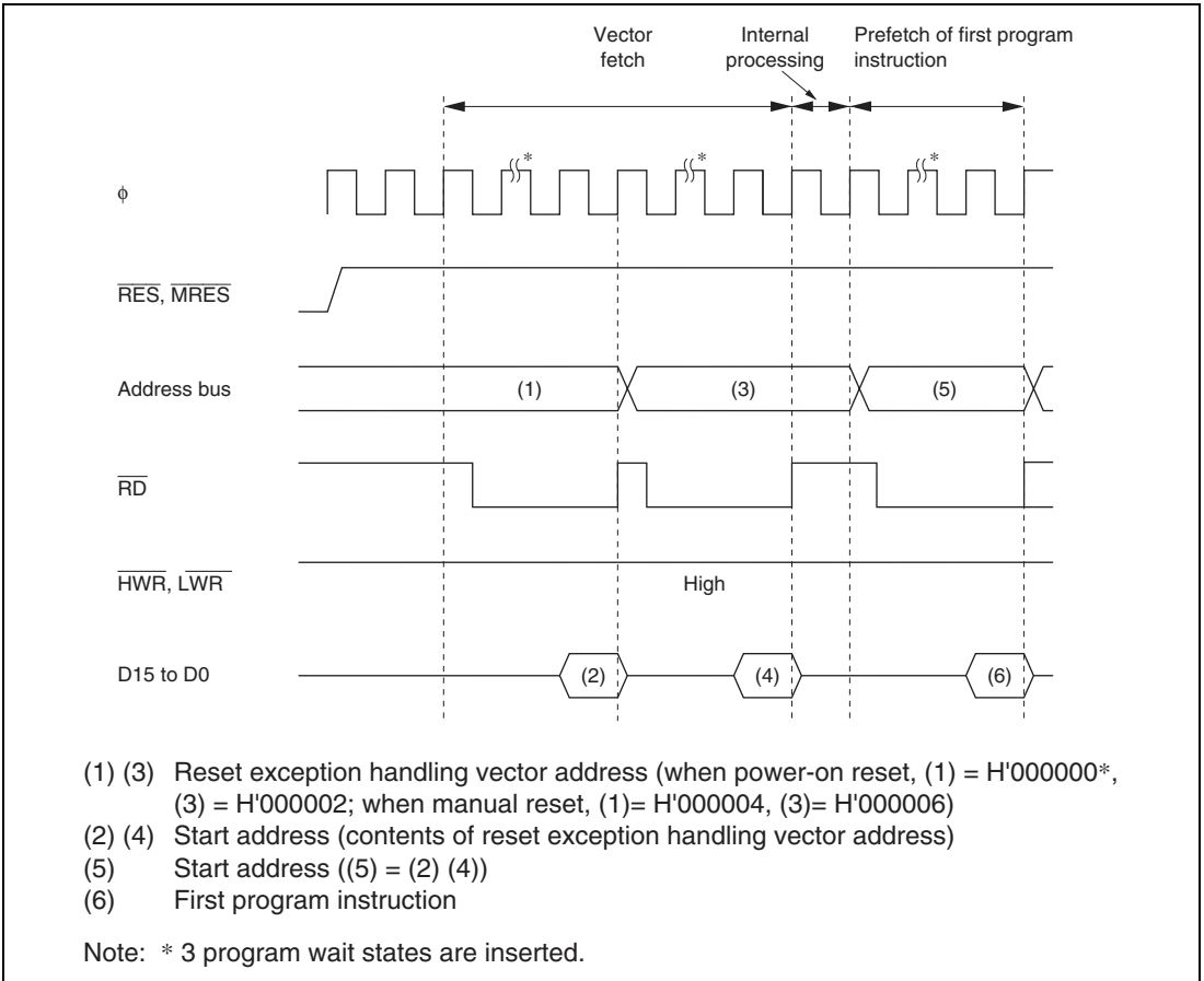
Figure 4.2 Reset Sequence (Modes 4 and 5)
