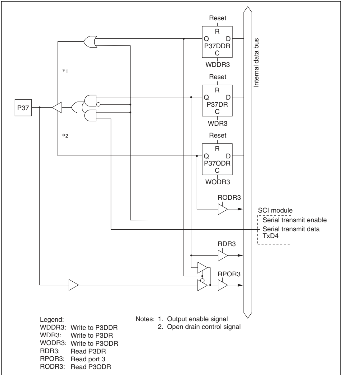
Figure C.14 (h) Port 3 Block Diagram (Pin P37)
