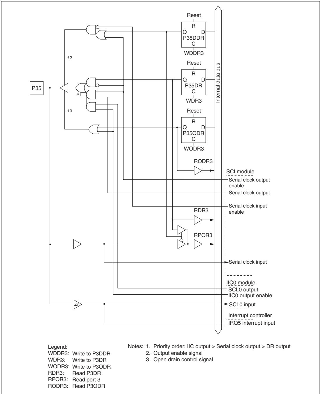
Figure C.2 (f) Port 3 Block Diagram (Pin P35)
