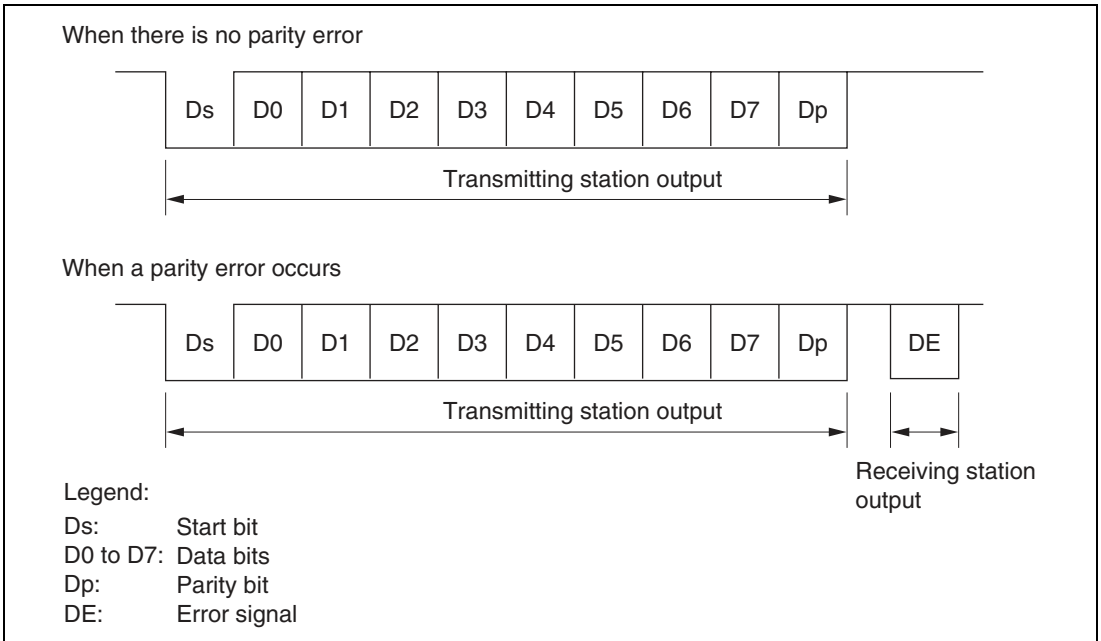
Figure 17.3 Normal Smart Card Interface Data Format
