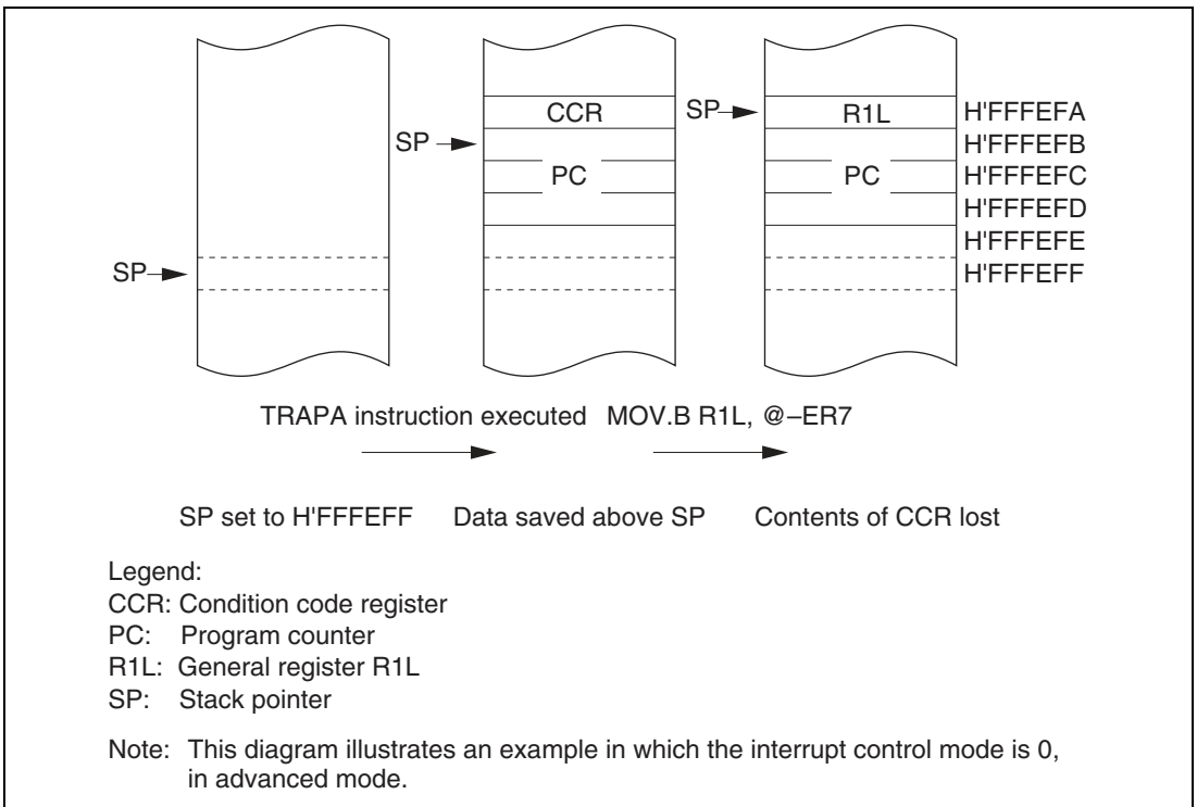
Figure 4.6 Operation when SP Value is Odd
