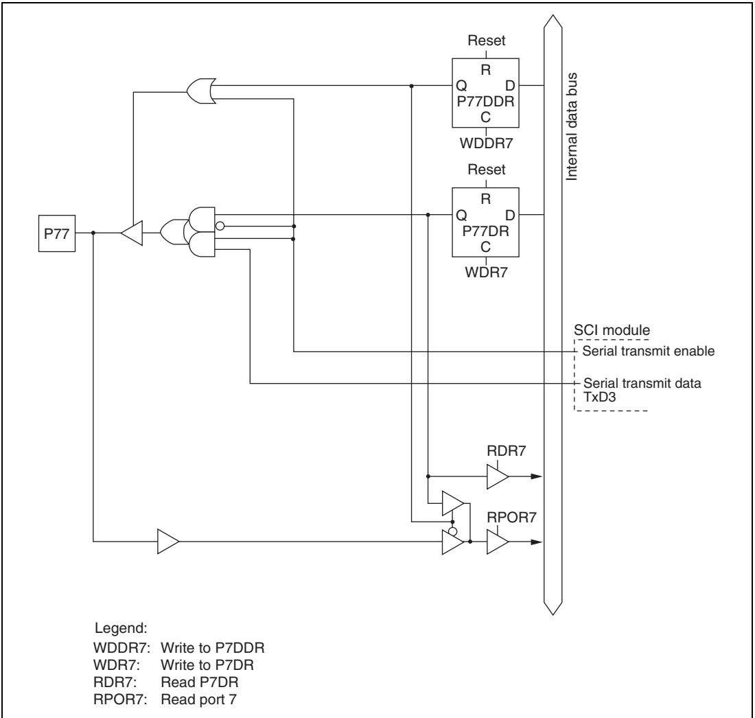
Figure C.16 (e) Port 7 Block Diagram (Pin P77)
