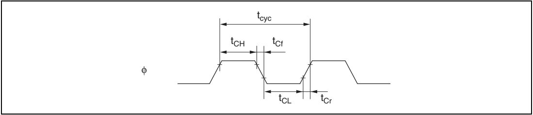
Figure 27.2 System Clock Timing
