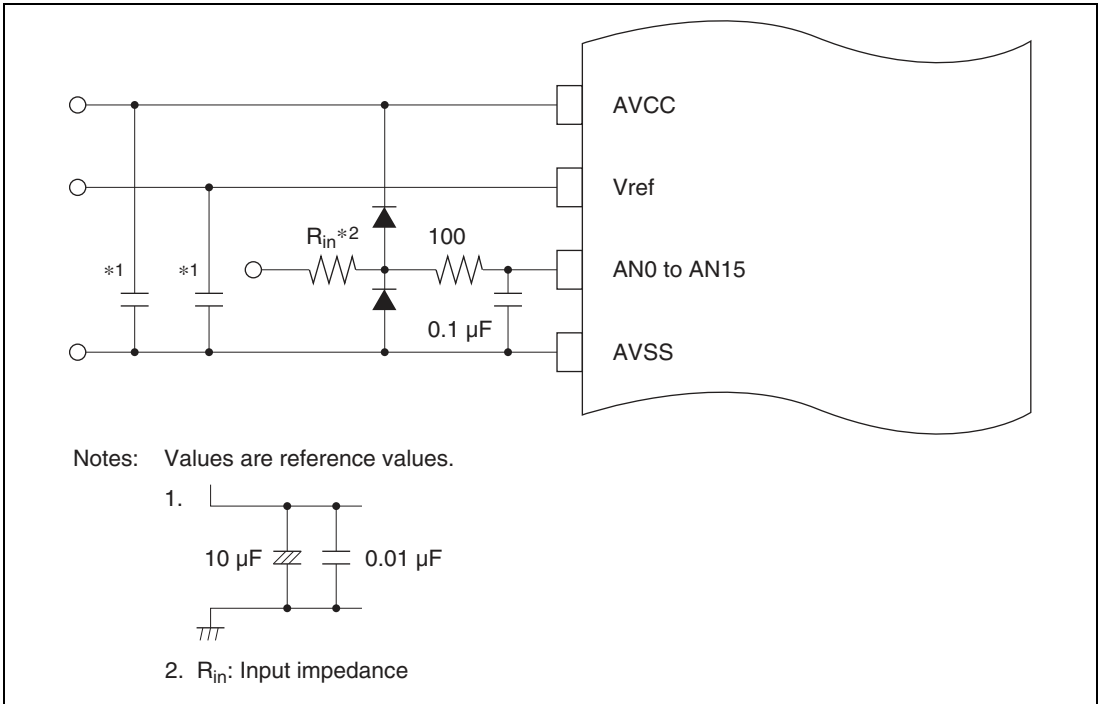
Figure 19.7 Example of Analog Input Protection Circuit
