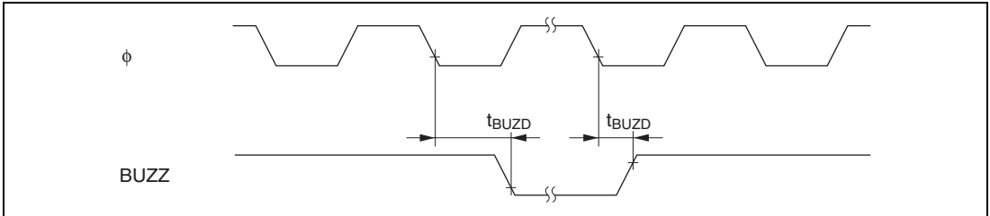
Figure 25.28 WDT1 Output Timing
