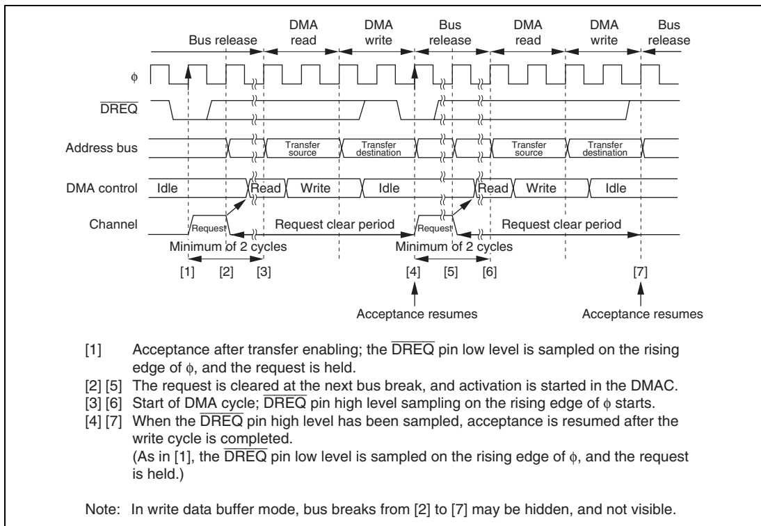
Figure 8.23 Example of DREQ Pin Falling Edge Activated Normal Mode Transfer
