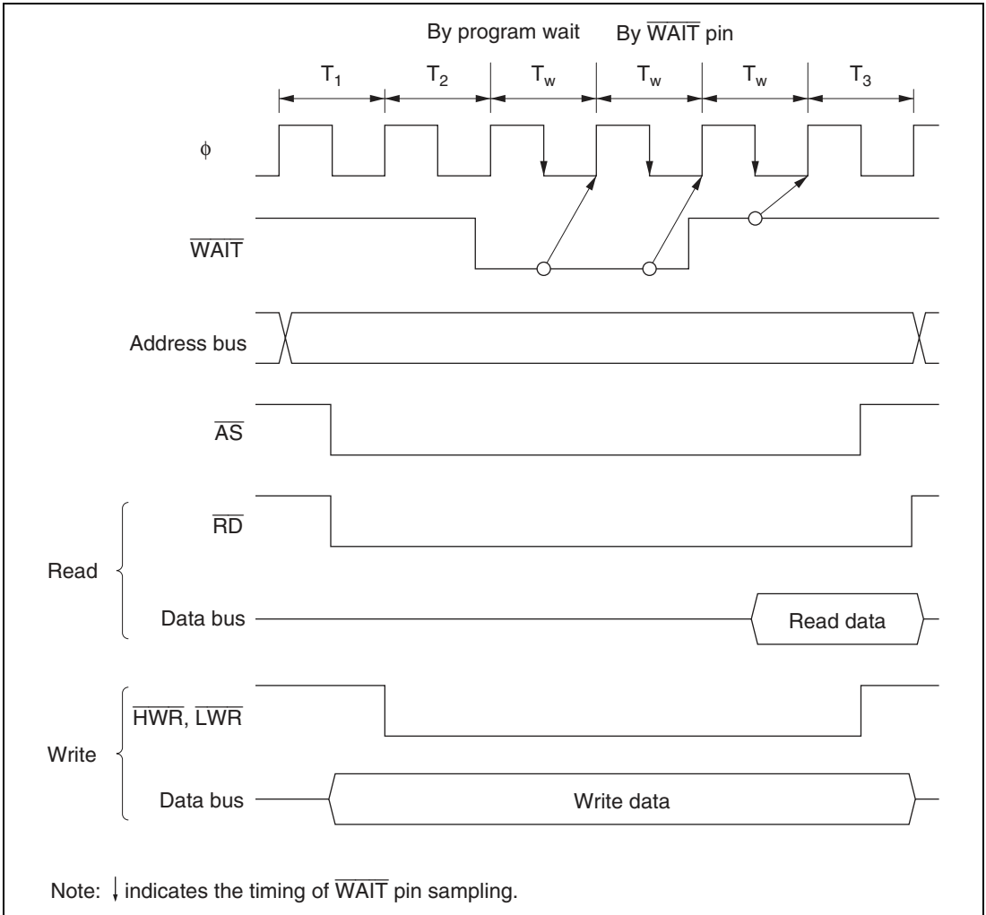
Figure 7.14 Example of Wait State Insertion Timing
