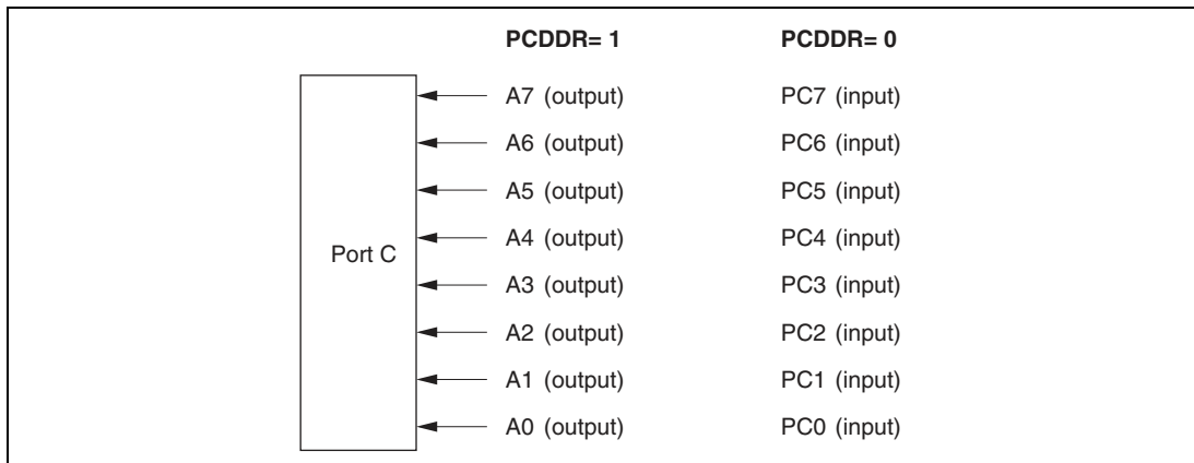
Figure 10B.10 Port C Pin Functions (Mode 6)
