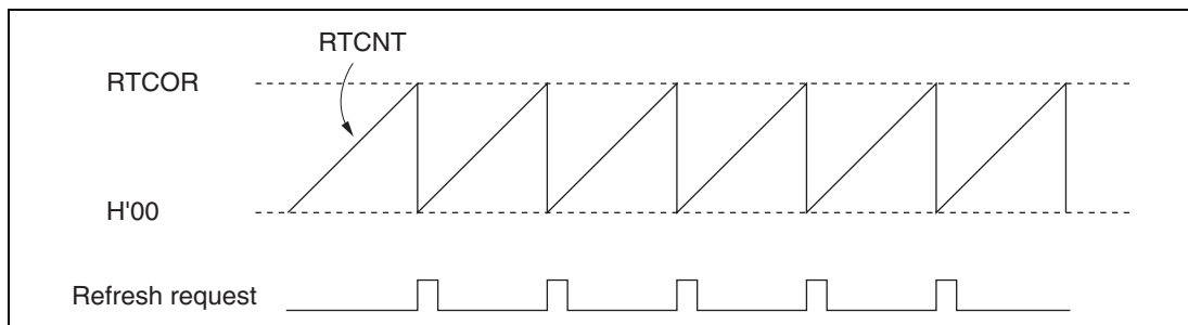
Figure 7.25 RTCNT Operation
