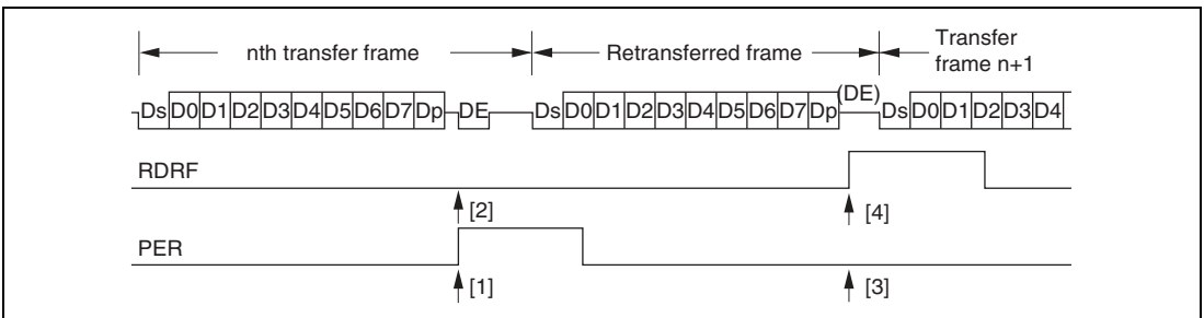
Figure 17.11 Retransfer Operation in SCI Receive Mode
