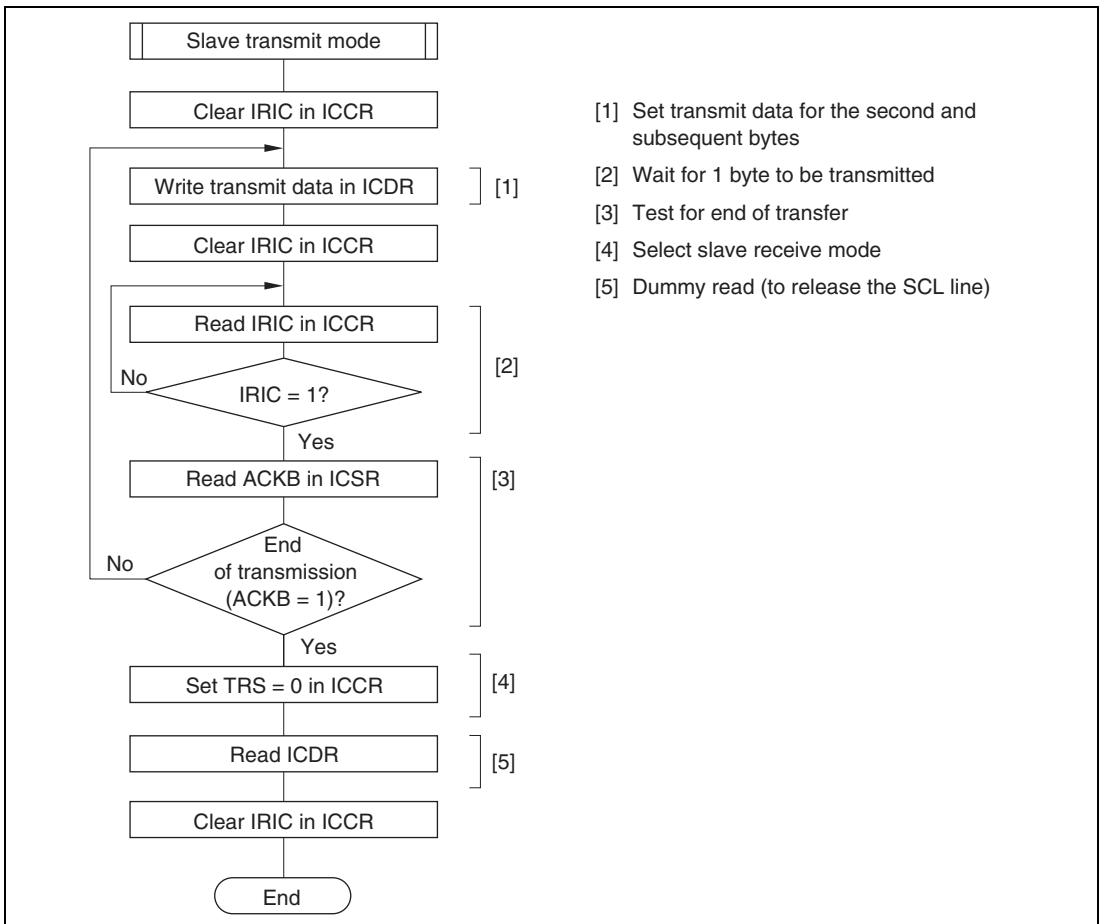
Figure 18.17 Flowchart for Slave Transmit Mode (Example)
