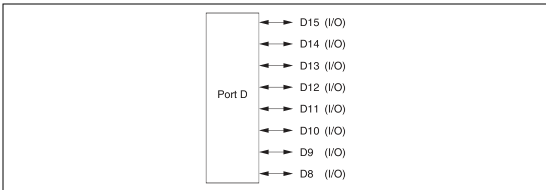
Figure 10A.13 Port D Pin Functions (Modes 4 to 6)
