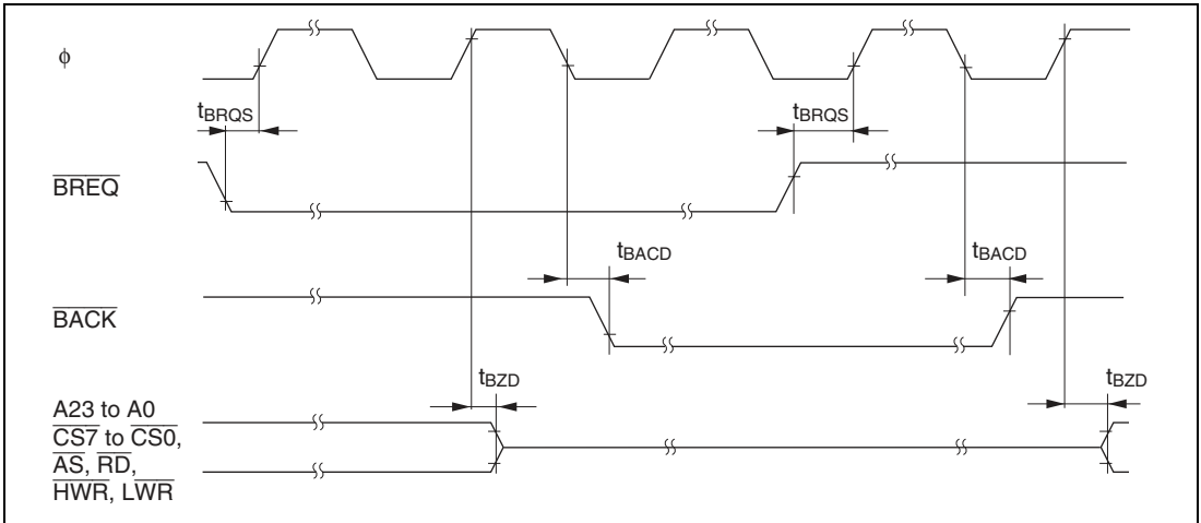
Figure 27.11 External Bus Release Timing
