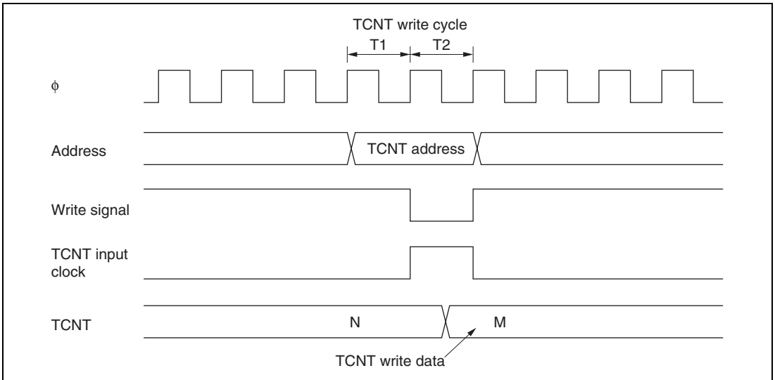
Figure 11.50 Contention between TCNT Write and Increment Operations
