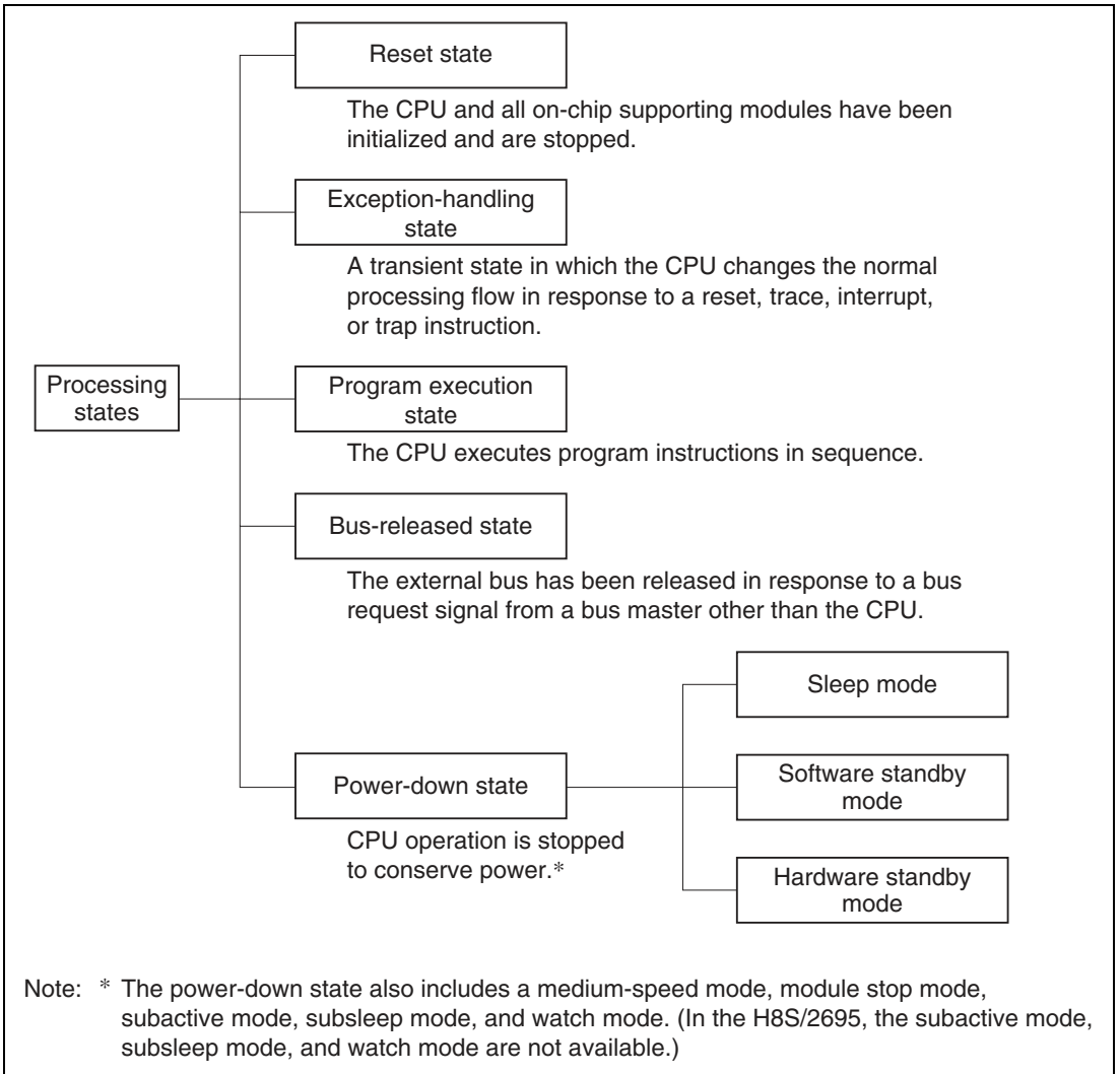
Figure 2.14 Processing States
