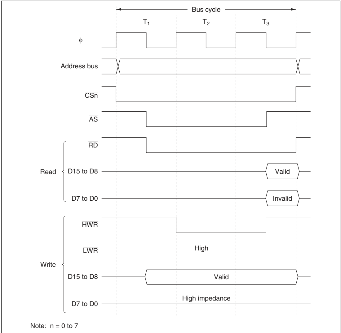
Figure 7.7 Bus Timing for 8-Bit 3-State Access Space
