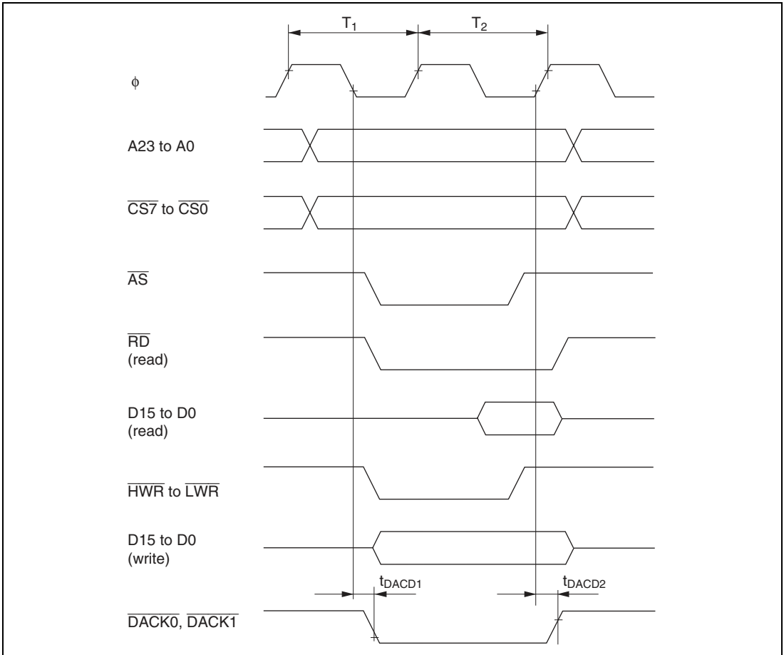
Figure 26.16 DMAC Single Address Transfer Timing / Two-State Access
