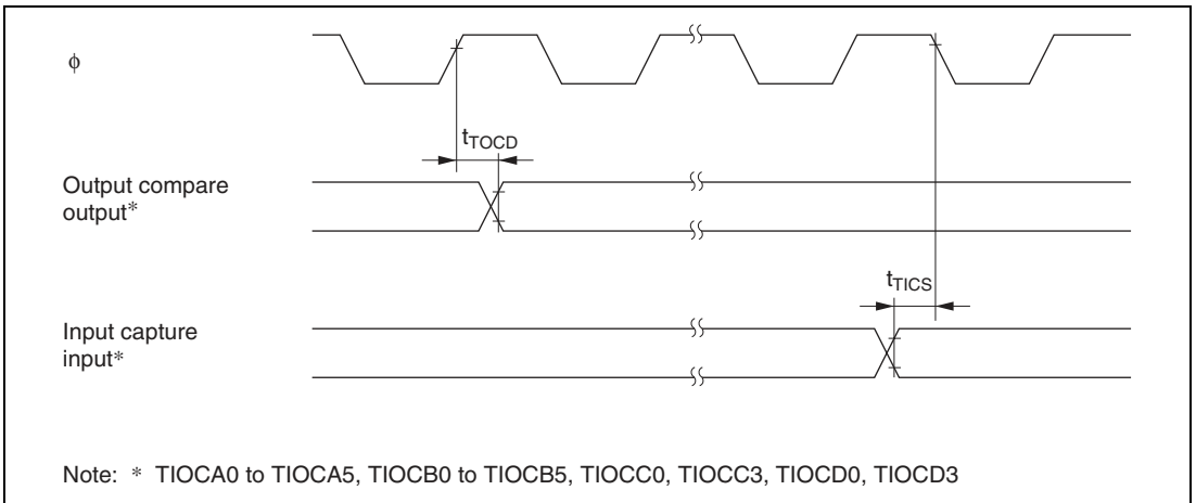
Figure 27.14 TPU Input/Output Timing
