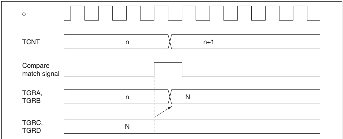
Figure 11.40 Buffer Operation Timing (Compare Match)
