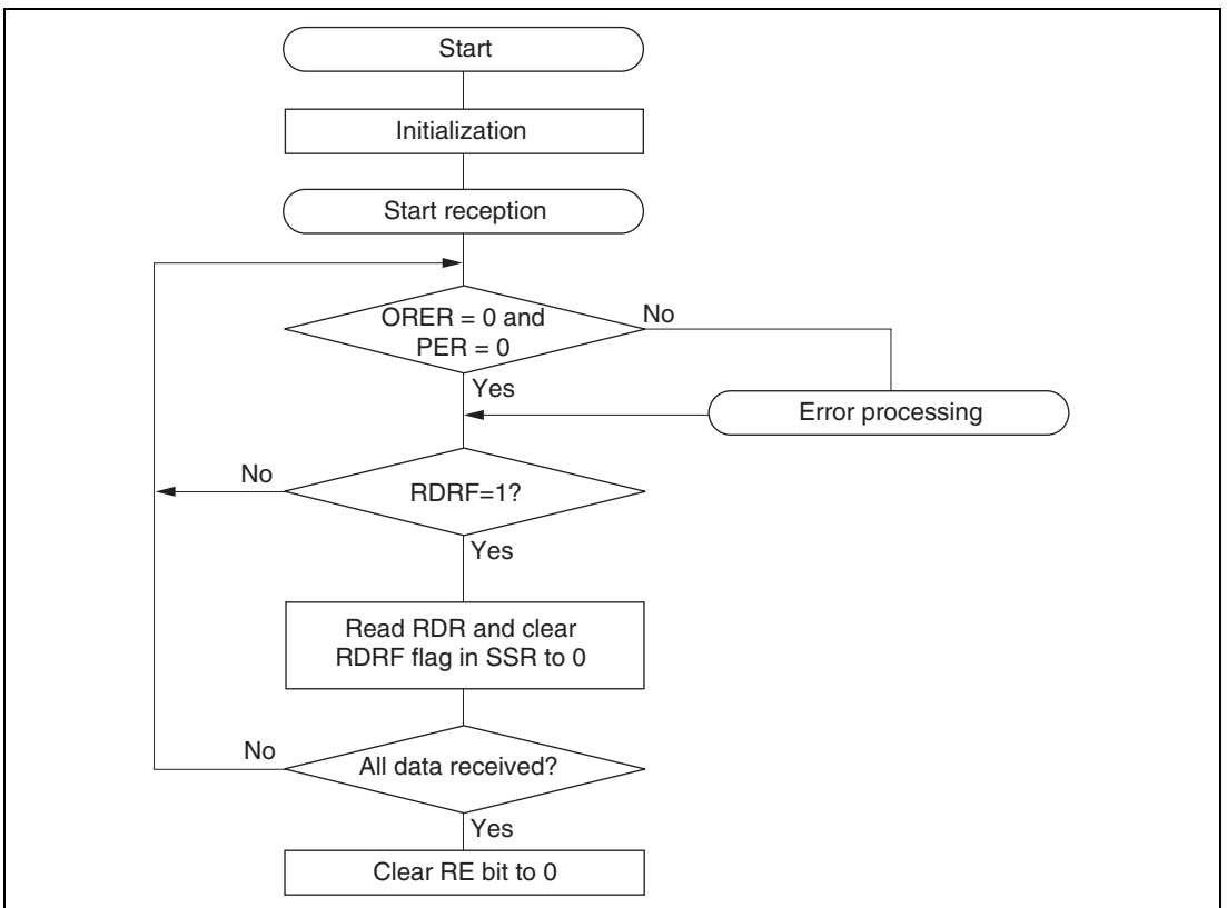
Figure 17.7 Example of Reception Processing Flow
