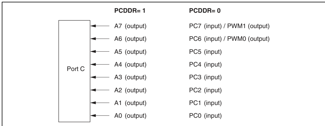
Figure 10A.10 Port C Pin Functions (Mode 6)
