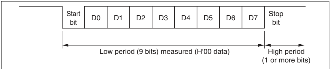
Figure 22.9 SCI Bit Rate Adjustment Operation
