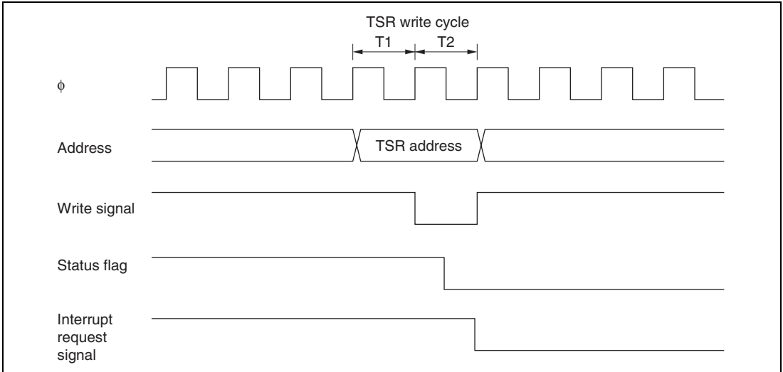
Figure 11.46 Timing for Status Flag Clearing by CPU
