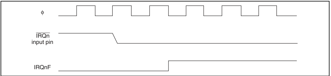
Figure 5.3 Timing of Setting IRQnF
