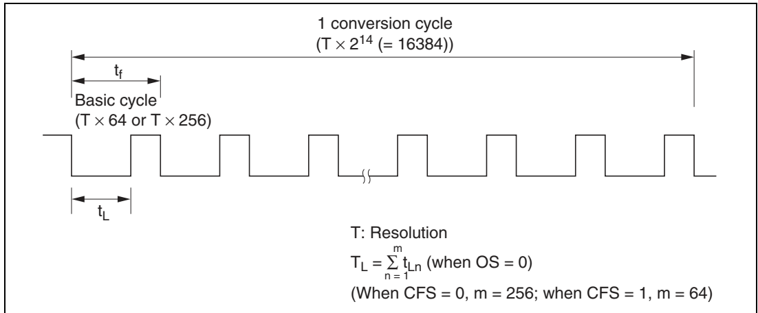
Figure 14.3 PWM D/A Operation
