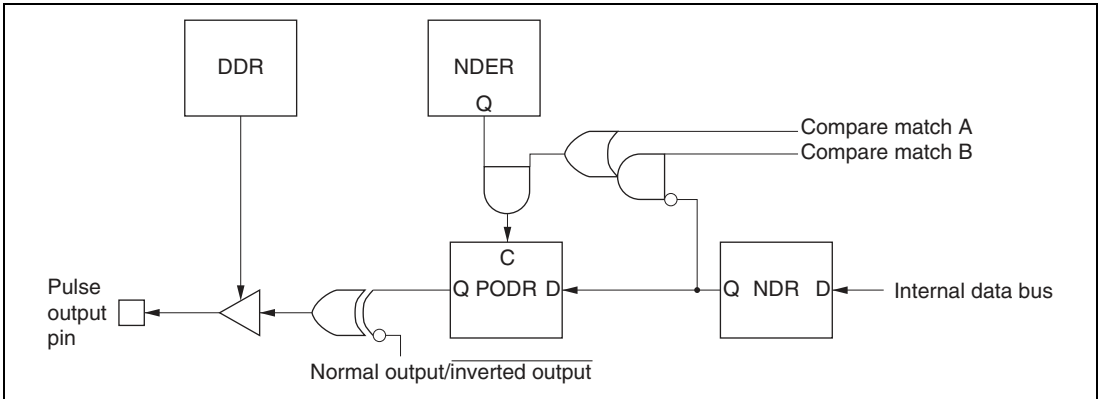
Figure 12.10 Non-Overlapping Pulse Output
