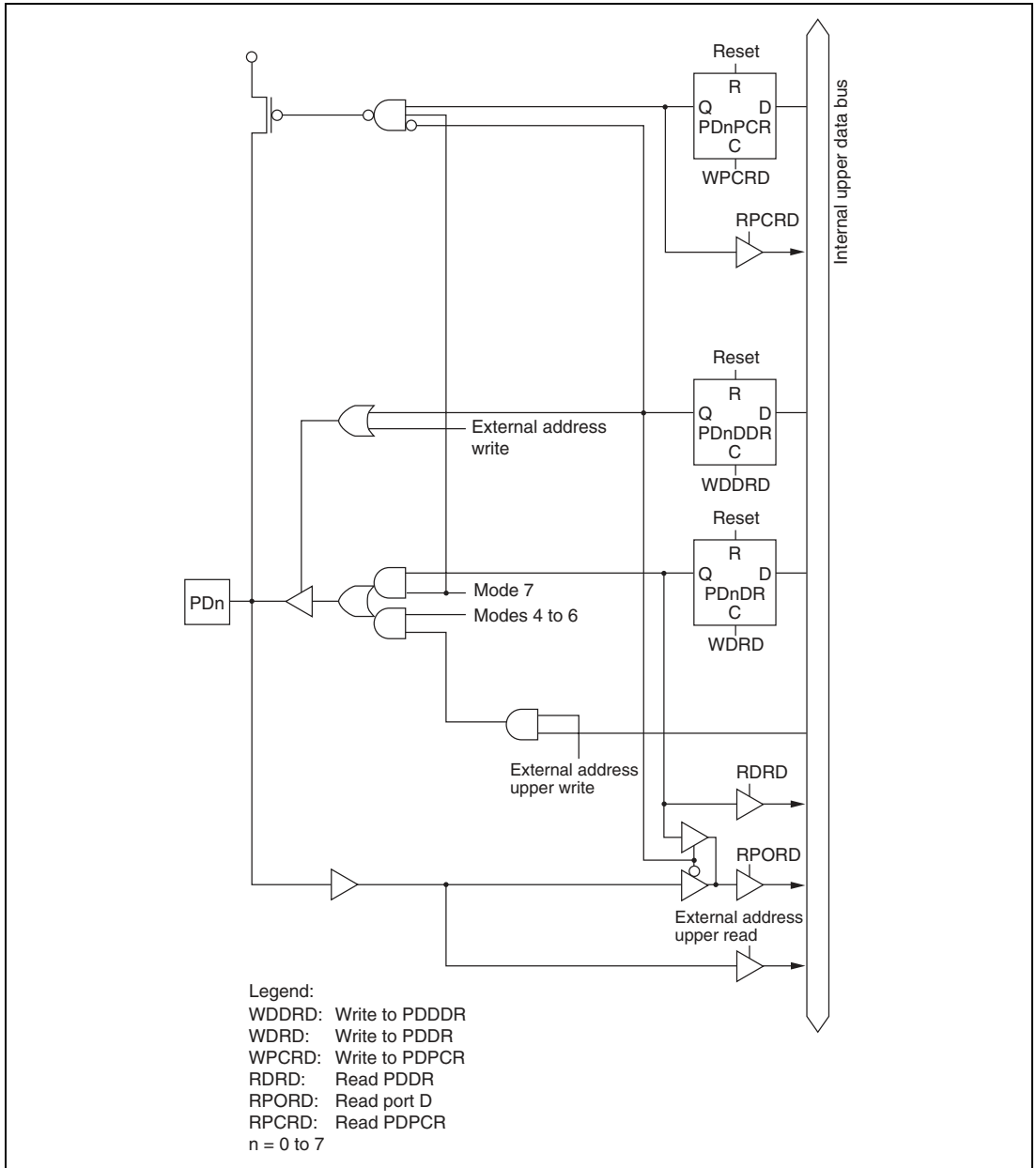
Figure C.21 Port D Block Diagram (Pins PD0 to PD7)
