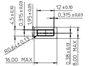
USB CABLE DRAWING
