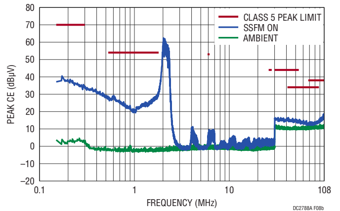
(b) CISPR25 Conducted EMI Performance Voltage Method
