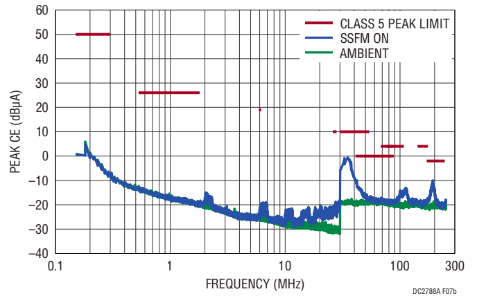
(b) CISPR25 Conducted EMI Performance Current Method
