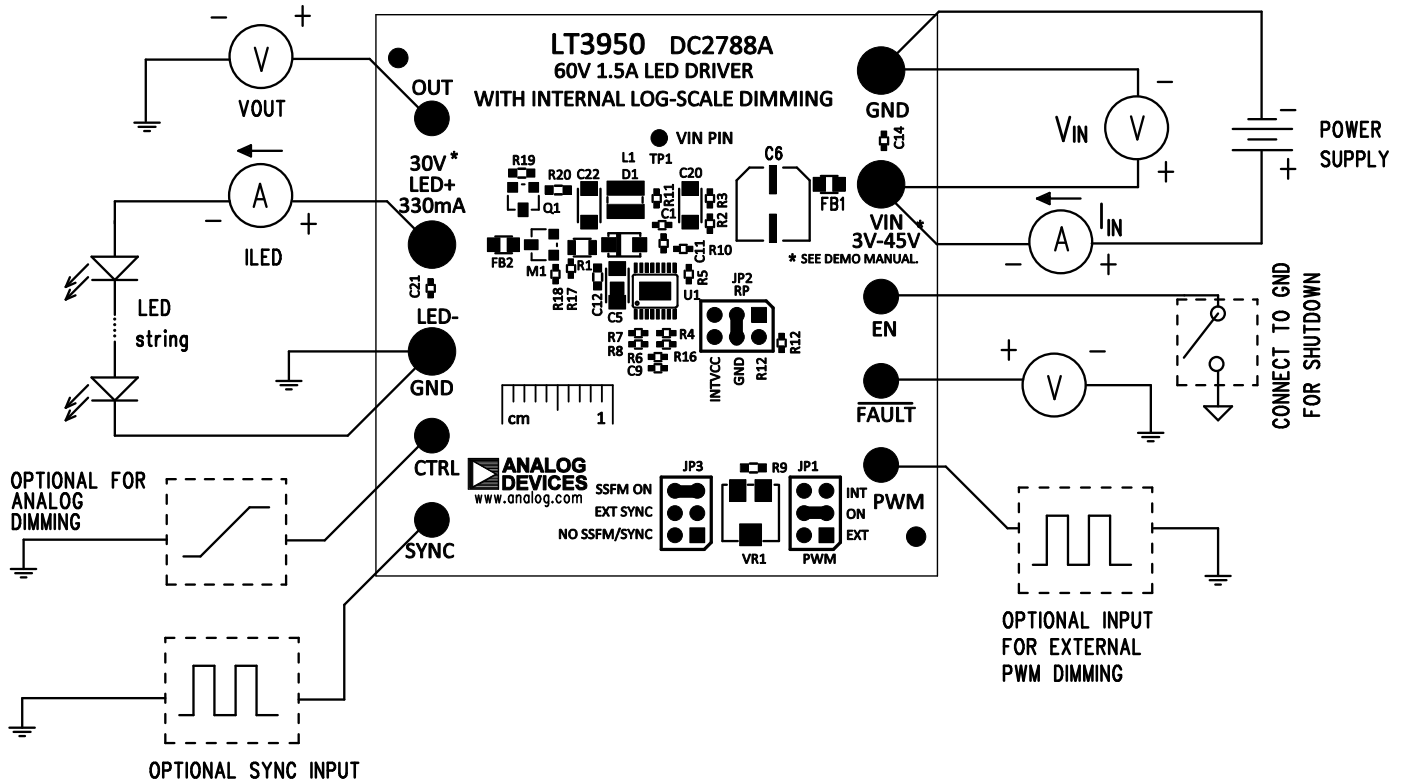
Figure 1. Test Procedure Setup Drawing for DC2788A
