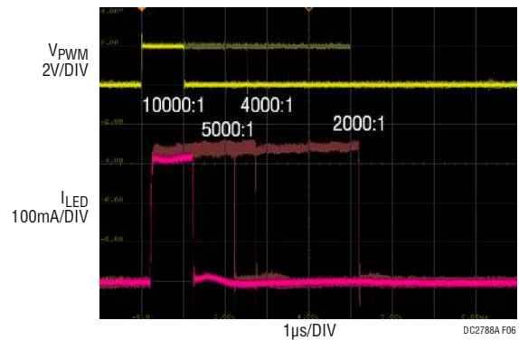
V_{IN} = 12V , V_{LED} = 24V , I_{LED} = 330mA f_{SW} = 2MHz + SSFM ON 100Hz EXTERNAL PWM DIMMING OUTPUT EMI FILTER REMOVED
