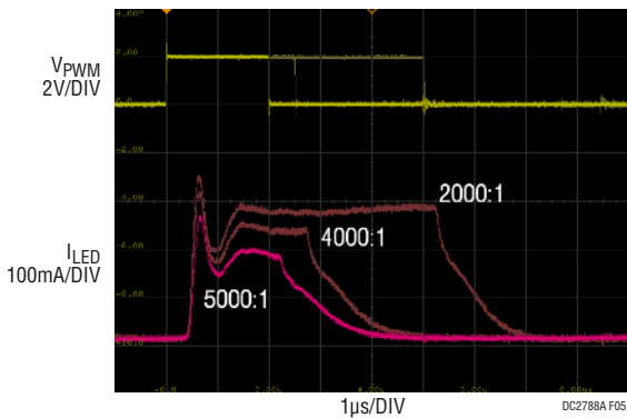
V_{IN} = 12V , V_{LED} = 24V , I_{LED} = 330mA f_{SW} = 2MHz + SSFM ON 100Hz EXTERNAL PWM DIMMING
