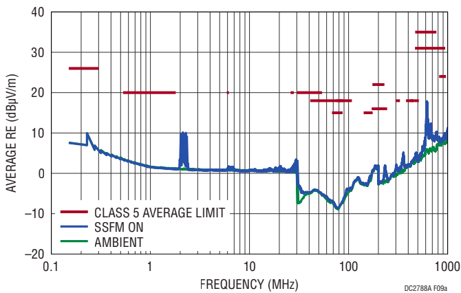
(a) CISPR25 Radiated EMI Performance
