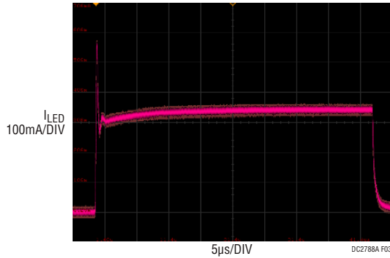
V_{IN} = 12V , V_{LED} = 24V , I_{LED} = 330mA f_{SW} = 2MHz + SSFM ON 50:1, 460Hz INTERNAL PWM DIMMING INFINITE PERSIST
