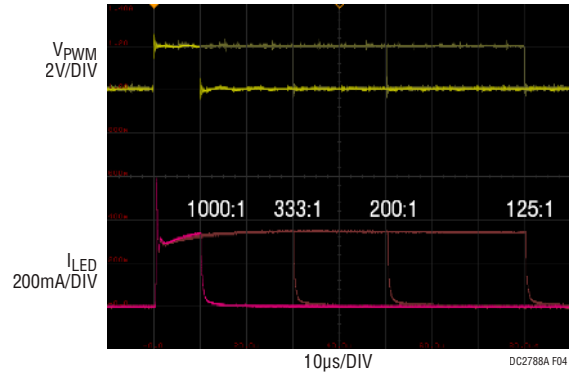
V_{IN} = 12V , V_{LED} = 24V , I_{LED} = 330mA f_{SW} = 2MHz + SSFM ON 100Hz EXTERNAL PWM DIMMING
