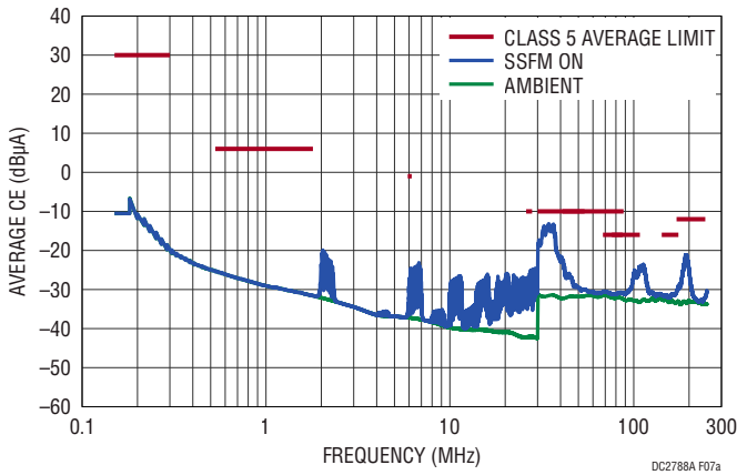
(a) CISPR25 Conducted EMI Performance Current Method
