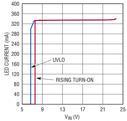
(b) LED Current vs Input Voltage
