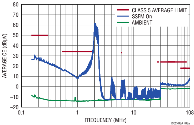
(a) CISPR25 Conducted EMI Performance Voltage Method
