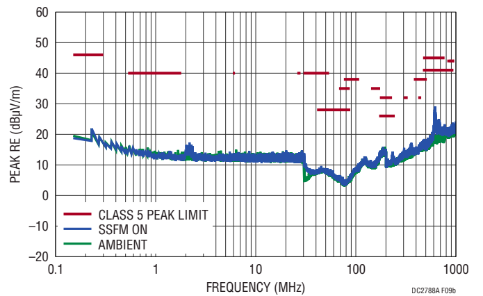
(b) CISPR25 Radiated EMI Performance
