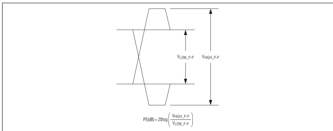
Figure 1. Output Preemphasis
