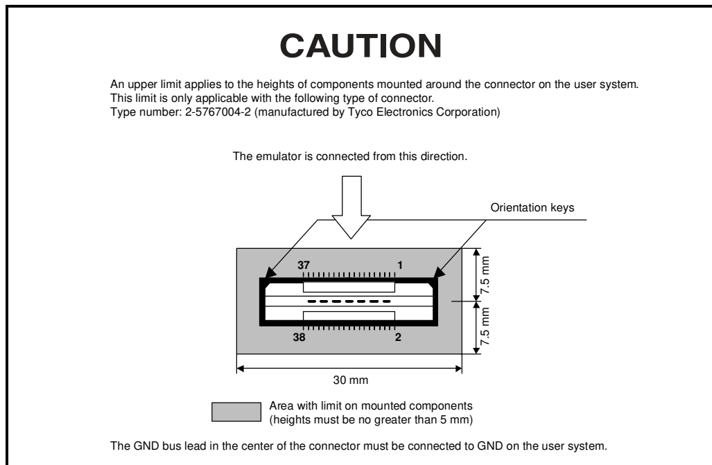
Figure 3 Limit on Height of Components Mounted on the User System
