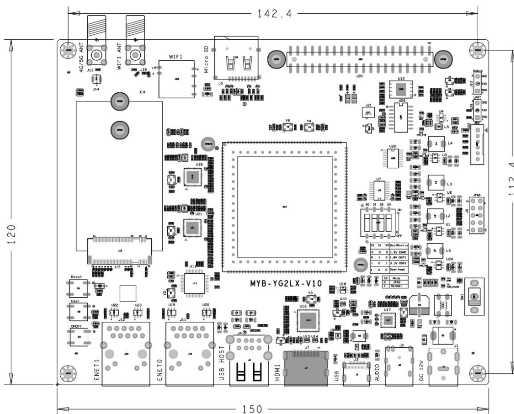
MYD-YG2LX Base Board Dimensions Chart
