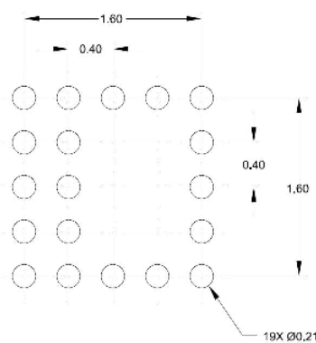
Figure 60 - Outline Drawing - CSP
