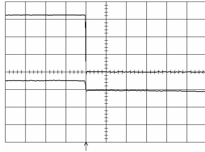
Shut-down enabled by disconnecting V_i at: T_{ref} = +25^\circ\text{C} , I_O = 15\text{ A} resistive load, V_i = 5.0\text{ V} . Top trace: output voltage (1.0 V/div.). Bottom trace: input voltage (2 V/div.). Time scale: 5.0 ms/div..
