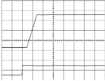
Start-up enabled by connecting V_i at: T_{ref} = +25^\circ\text{C} , I_O = 15\text{ A} resistive load, V_i = 5.0\text{ V} . Top trace: output voltage (1.0 V/div.). Bottom trace: input voltage (5 V/div.). Time scale: 5 ms/div..
