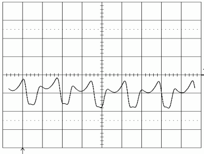
Output voltage ripple (20mV/div.) at: T_{ref} = +25^\circ\text{C} , I_O = 15\text{ A} resistive load, V_i = 5.0\text{ V} . Time scale: 2 \mu\text{s} /div. See the filter in the Output ripple and noise section (EMC Specification).
