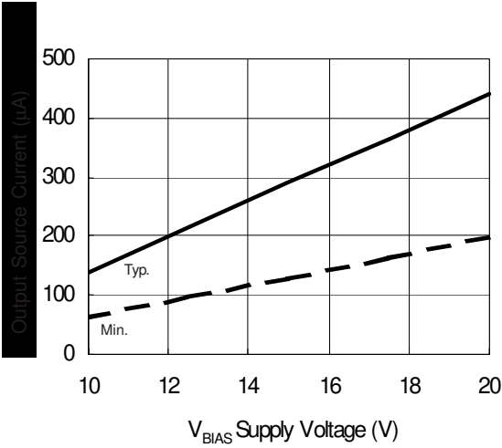
Figure 27B. Output Source Current vs. Supply Voltage
