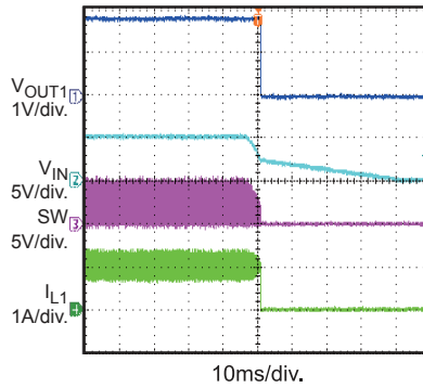
Vin Power Down IOUT1 = 1A, IOUT2 = 0A
