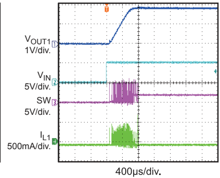
Enable On IOUT1 = IOUT2 = 0A
