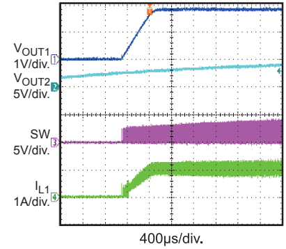
Vin Power On IOUT1 = 1A, IOUT2 = 0A
