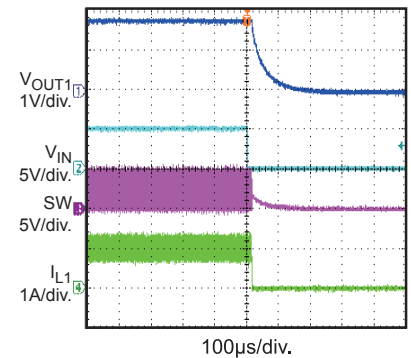
Enable Down IOUT1 = 1A, IOUT2 = 0A
