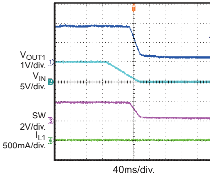
Vin Power Down IOUT1 = IOUT2 = 0A
