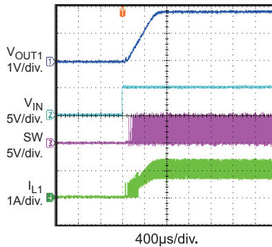
Enable On IOUT1 = 1A, IOUT2 = 0A
