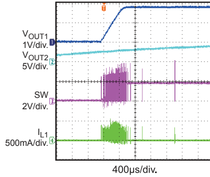
Vin Power On without Load IOUT1 = IOUT2 = 0A
