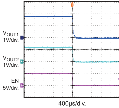
EN Down with Load IOUT1 = IOUT2 = 1A
