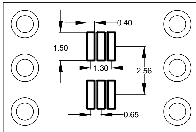
Back: SOT363
