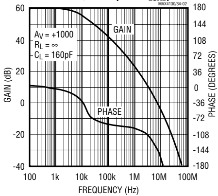
GAIN AND PHASE vs. FREQUENCY (WITH LOAD)
